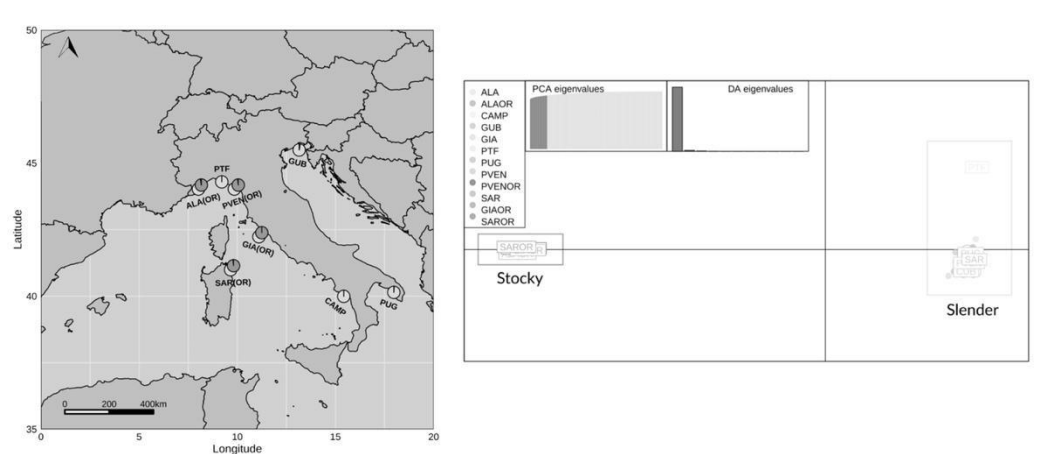
Fig. 1: Left: Map showing the sampling localities within the study. Right: Discriminant Analysis of Principal Components (DAPC) with populations as prior grouping information
