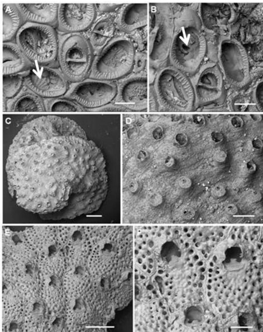
Fig. 3: (A–B) Crassimarginatella mathildae Pica & Berning, 2022 colony overgrowing Cribrilaria radiata (arrowed): (A) Two types of vicarious avicularia with narrow downcurved mucro; (B) Ovicellate zooids and avicularia, a primary orifice of Cribrilaria radiata (arrowed); (C–D) Plagioecia sarniensis (Norman, 1864): (C) Colony; (D) secondary nanozooids developed on closing plates; (E–F) Prenantia cf. inerma (Calvet, 1906): (E) group of autozooids; (F) Details of autozooids. Scales bars: A, B, D, F = 200 µm ; C,E = 500 µm.
