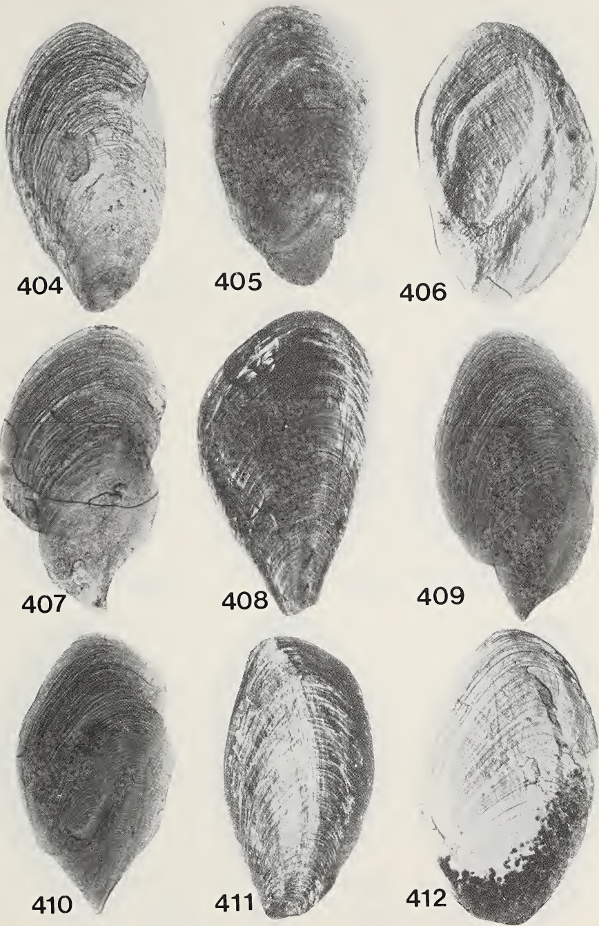
Figs 404-412. Buccinid opercula. 404, Neptunea brevicauda , E. Canada, 6.6 mm. 405, Neptunea antiqua , off Korsfjorden, Bergen area, 300 m, 4.2 mm. 406, Turrisipho fenestratus , W of Korsfjorden, 280 m, 2.5 mm. 407, Turrisipho moebii , same locality, 3.9 mm. 408, Turrisipho moebii , off Reykjanes, Iceland, 19.2 mm. 409, Turrisipho lachesis , INGOLF st 28, 5.3 mm. 410 and 411, Turrisipho voeringi , INGOLF st 105, 6.5 mm and 14.4 mm. 412, Troschelia bernicensis , southern Bay of Biscay, 400-690 m, 15.7 mm.
