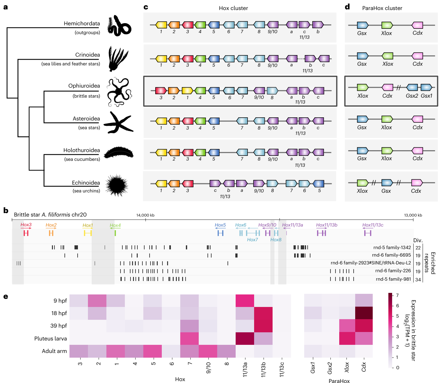
Fig. 2 | Hox and ParaHox clusters organization across echinoderms.
