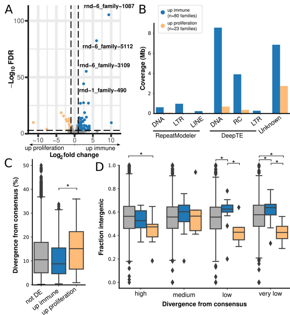
Extended Data Fig. 10 | Differential transcriptional activity of repetitive elements in the immune and proliferative phases of brittle star arm regeneration.
