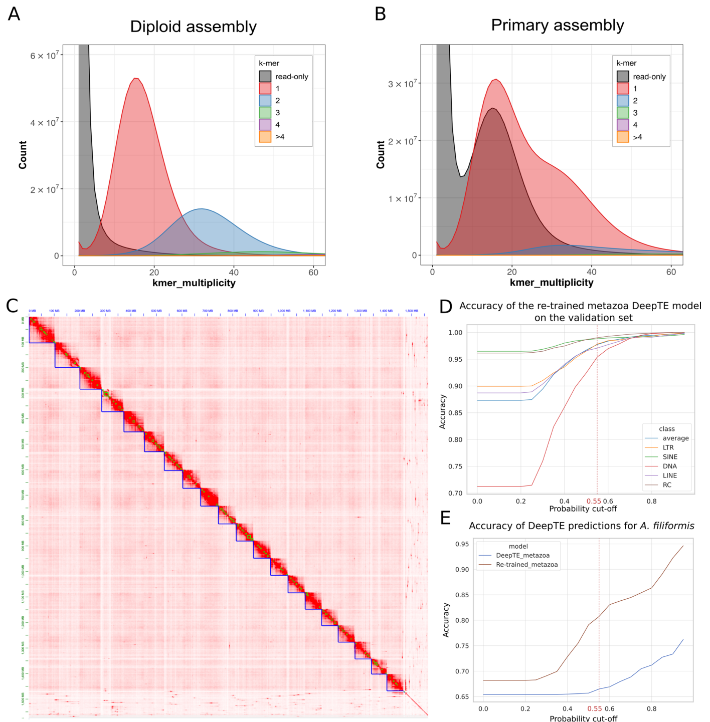
Extended Data Fig. 1 | Genome assembly and repeat classification. A. K-mer spectrum of the diploid assembly, that is before haplotype removal. Read-only k-mers (black curve) correspond to sequencing errors, and are not represented in the assembly. The 1-copy k-mer peak at 15X coverage (1n, red) corresponds to reads from heterozygous regions, whereas the 2-copy k-mer peak at 30X coverage (2n, blue) corresponds to homozygous regions. B. K-mer spectrum of the primary assembly, that is after haplotype removal. Following the collapse of haplotypes, half of the k-mers of the heterozygous peaks are accordingly not represented in the assembly anymore and homozygous regions are present as single copies only. C. Hi-C contact map showing the density of interactions
