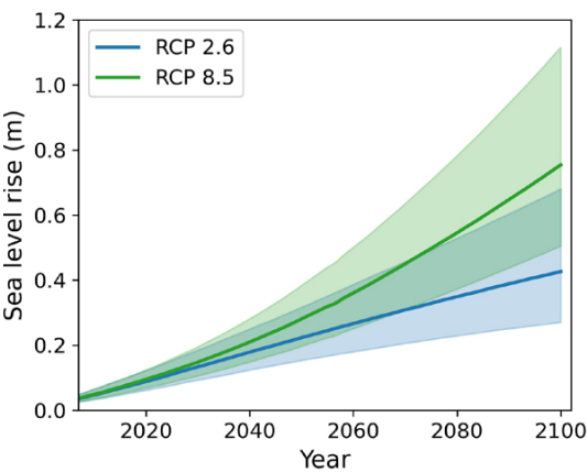
FIGURE 1. Sea level rise projections for the River Humber for a low (RCP2.6) and high emission scenario (RCP8.5), showing 5 th , 50 th (solid line), and 95 th percentiles. Underlying data are from UKCP18 (Palmer et al., 2018). The RCP numbers refer to the projected radiative forcing at 2100 under different climate change scenarios, for example, 2.6 W m -2 and 8.5 W m -2 .
