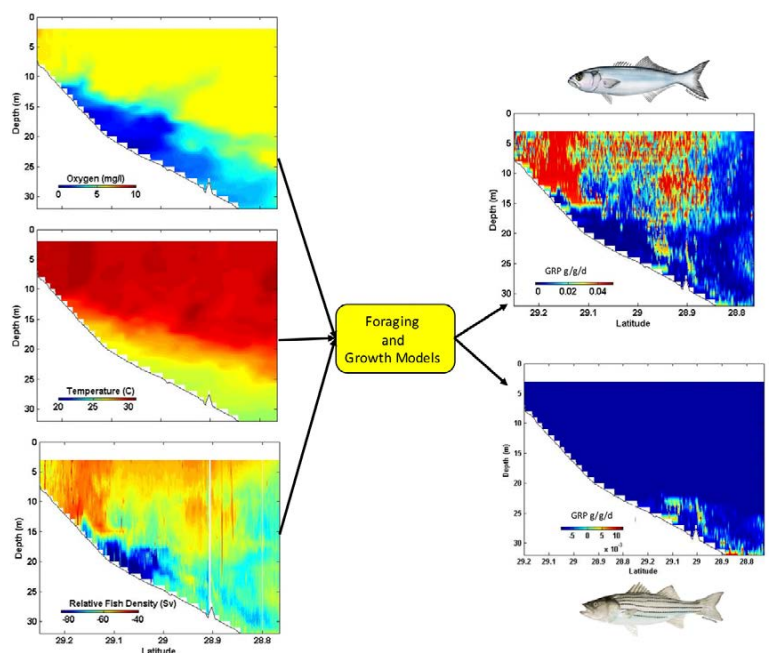
FIGURE 3. Dissolved oxygen, temperature, and fish prey density, along with resultant growth rate potentials for adult bluefish and striped bass across a transect in the Northern Gulf of Mexico.
