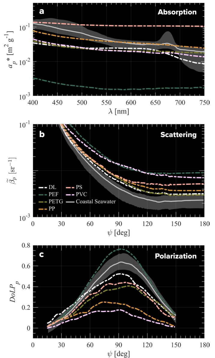
FIGURE 3. (a) Absorption, (b) scattering, and (c) polarization properties of six microplastic samples in comparison with coastal seawater samples from Southern California and Northern Alaska. Microplastic samples are plotted with dash-dotted lines. Solid gray lines represent median data and gray shaded regions represent 10 th and 90 th percentile data from 52 natural seawater samples from nearshore oceanic and coastal waters. Panel (a) shows the particulate absorption spectra normalized by particle mass concentration for each of the six samples, (b) shows the particulate phase function \tilde{\beta}_p (the normalized intensity of the scattered light as a function of angle), and (c) shows the particulate degree of linear polarization DoLP p (the fraction of scattered light that is linearly polarized in the vertical orientation as a function of angle). Note that these results refer to absorption and scattering properties of particles only, with contributions of molecular water and dissolved salts removed. Data shown in (b) and (c) utilize only green light of wavelength \lambda = 532 nm.
