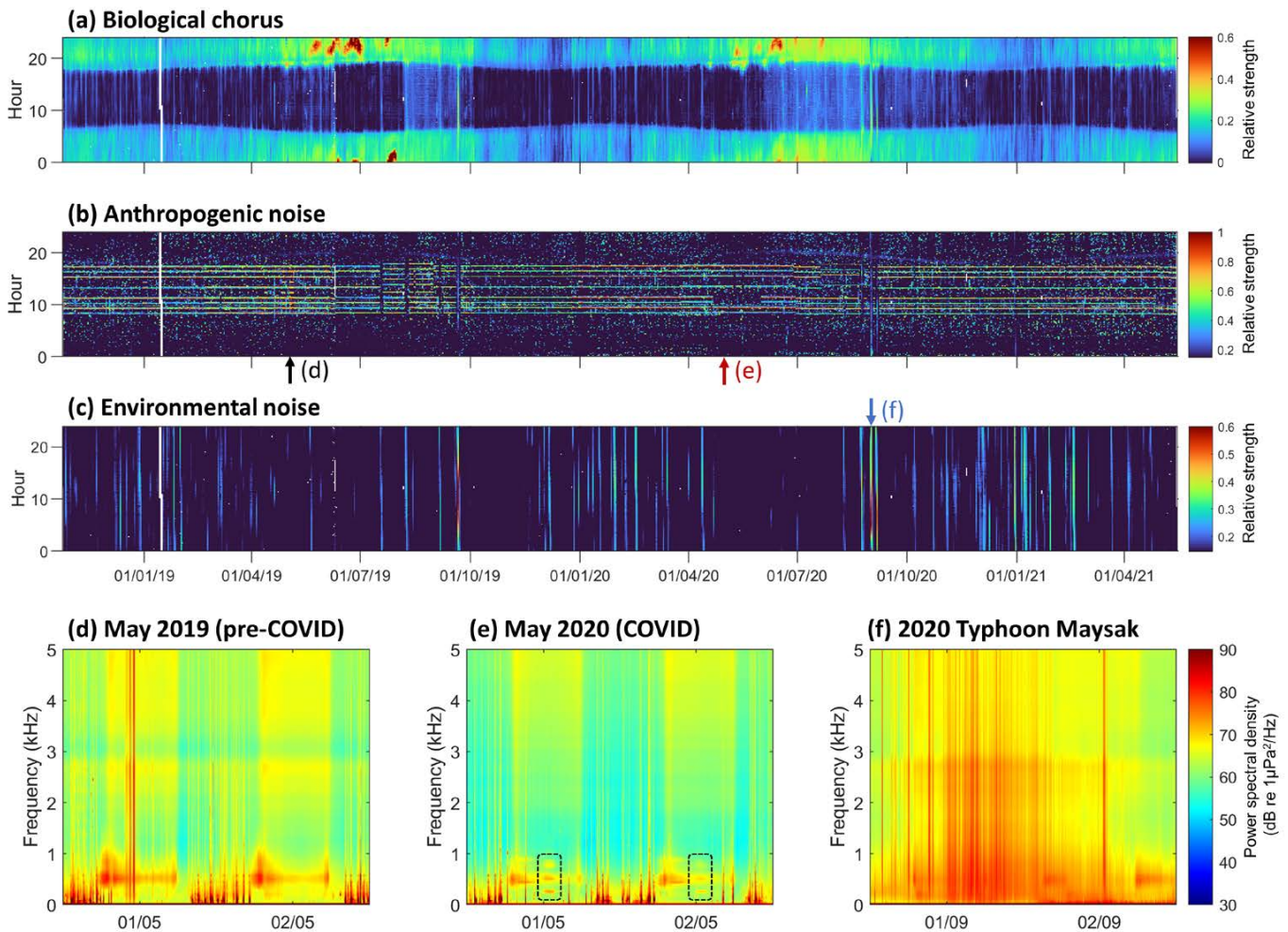
FIGURE 6. Dynamic soundscapes from a coral reef site at 20 m depth off Sesoko Island from October 2018 to May 2021. (a) Biological choruses displayed marked diurnal and seasonal variations. Particularly in warm seasons, more nighttime fish choruses were recorded, and their intensities varied with tidal and lunar phases. (b) Noise events that regularly occurred between 8 a.m. and 6 p.m. were associated with ferries. Other noise events were attributed to fishing vessels, tugboats, and freight ships. (c) Wind and wave noises were mainly produced during typhoon season (June–September) and northeastern monsoon season (December–March). Colors represent the relative strength of each sound source. The arrows indicate the dates corresponding to the long-term spectrograms of (d) the 2019 Golden Week holiday, (e) the first nationwide state of emergency in 2020, and (f) September 1, 2020, when Typhoon Maysak was closest to Okinawa Island. Dashed squares indicate the new type of fish chorus detected during the COVID-19 anthropause. Colors of the long-term spectrograms represent the median power spectral densities measured every 10 min.
