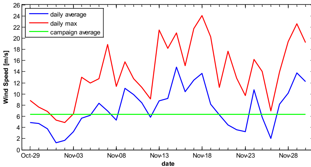
Figure 4-4 – Day-averaged wind speed (blue line), maximum wind speed (red line) and campaign average (green line).
