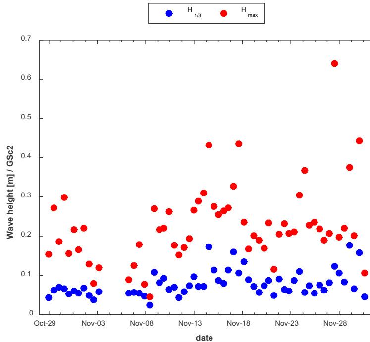
Figure 4-30 – Significant ( H_{1/3} ) and maximum wave height per tidal cycle at Gsc2 location (southern transect –high mudflat).
