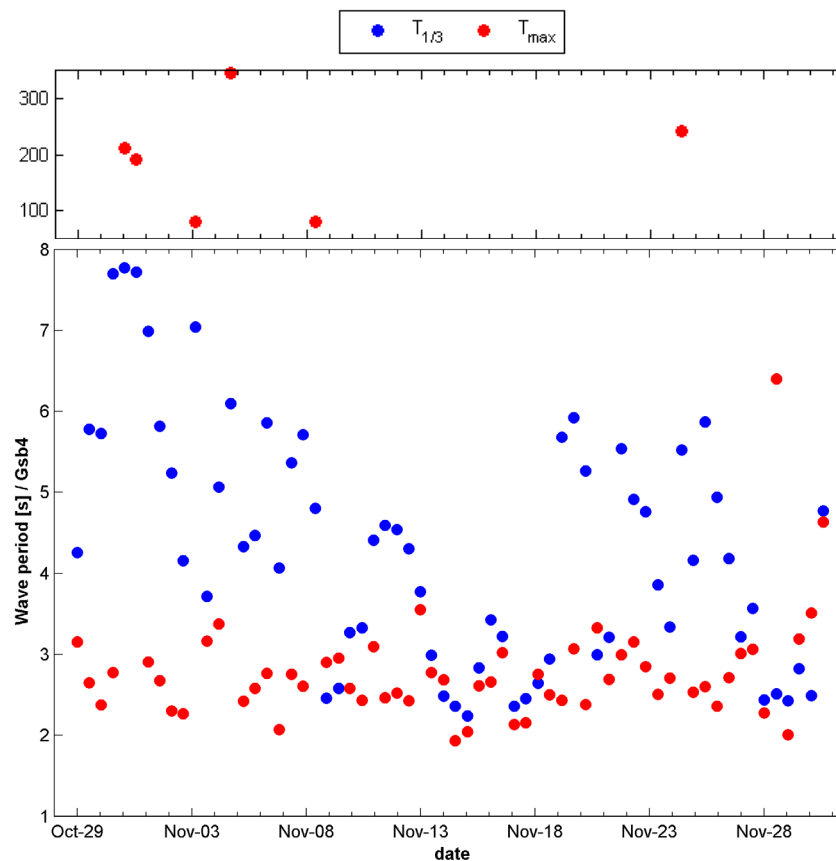
Figure 4-23 – Mean wave period of the highest 1/3 wave ( T_{1/3} ) and wave period of the highest wave ( T_{\max} ) per tidal cycle at Gsb4 location (northern transect). T_{\max} outliers are denoted in separate window above.
