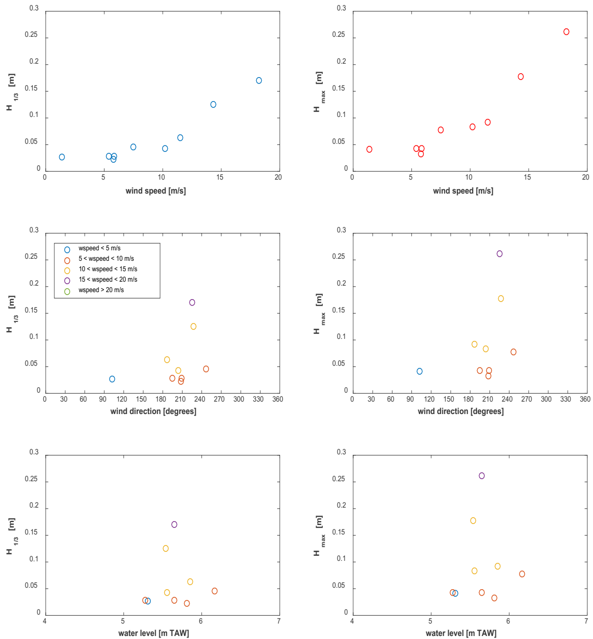
Figure 7-4 – Significant (left figures) & maximum wave heights (right figures) versus wind speed, wind direction and water level for the no-ship events detected at GSb2.
