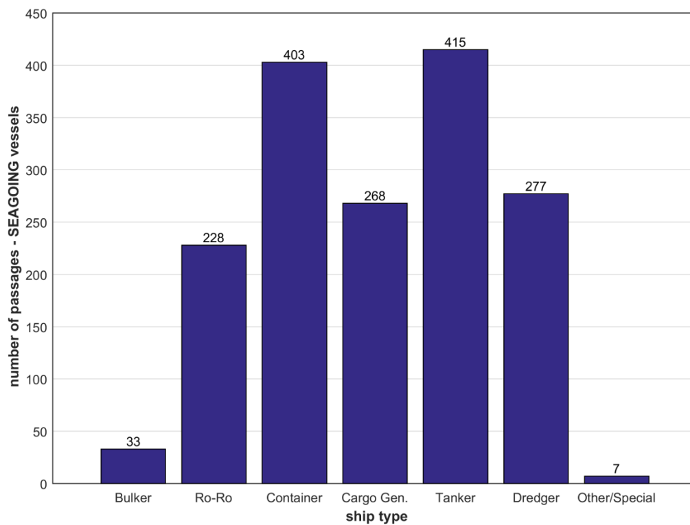
Figure 5-7 – Seagoing vessel passage frequency with respect to ship length and type at SFD entry line (north transect) during the measuring campaign.
