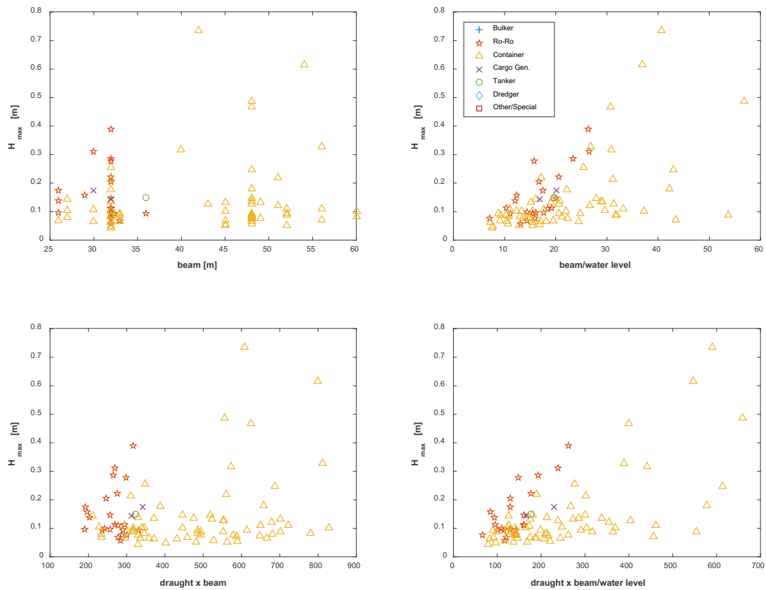
Figure 6-39 – H_{\max} versus the ship beam, the ratio of the beam to water level, the product of beam and draught, and the product of beam and draught divided by water level for the large vessel events at Gsb4 (north) location.
