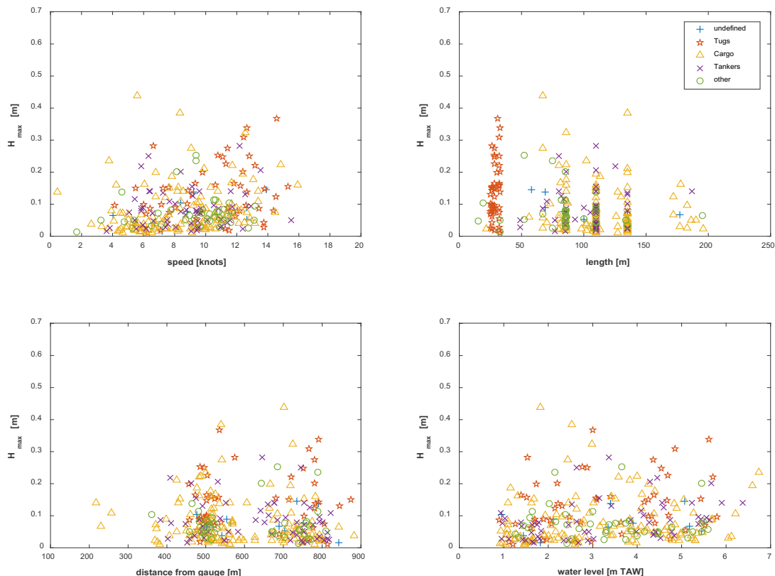
Figure 6-13 – Secondary wave height versus ship speed&amp; length, distance from the measuring gauge, and water level for the selected inland ship events at Gsb4 lower tidal flat (north) location.
