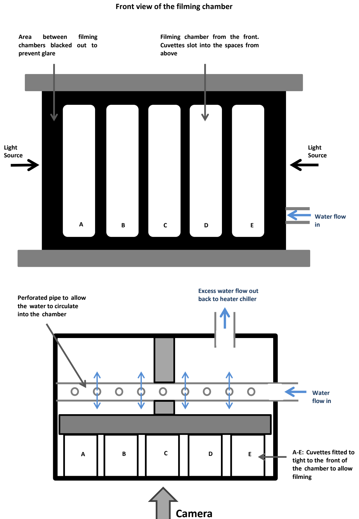
Figure 5.2: The experimental filming chamber used to film the larvae from above and from the front. The cuvettes were held flush against the front of the chamber by a holding bar, to prevent image distortion. The temperature was maintained by a constant flow of water in to the chamber, which insulated the cuvettes but did not mix with the water inside them.
