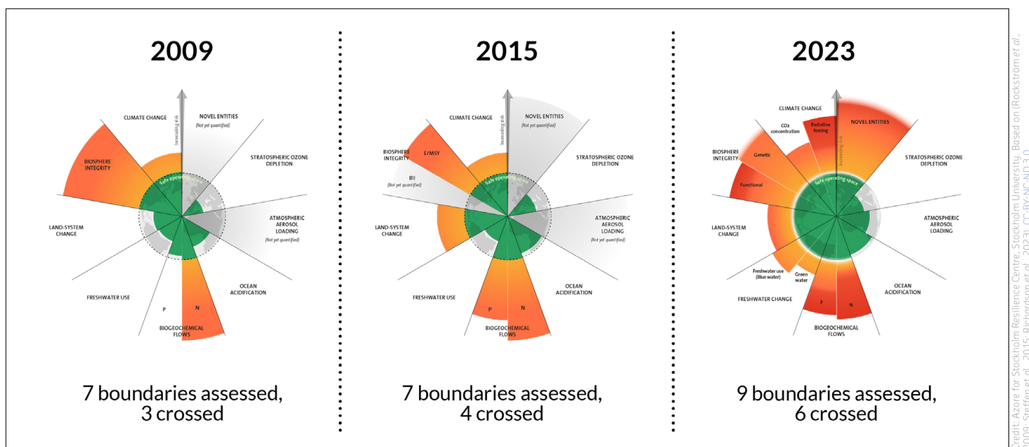
Figure 1.1 The evolution of the planetary boundaries' framework. By 2009 humanity had crossed three of these boundaries (biosphere integrity, climate change and biogeochemical flows); by 2015 we had also crossed land-system change; and by 2023 the boundaries of novel entities introduced by humans (e.g. chemical compounds) and freshwater change were also crossed.
