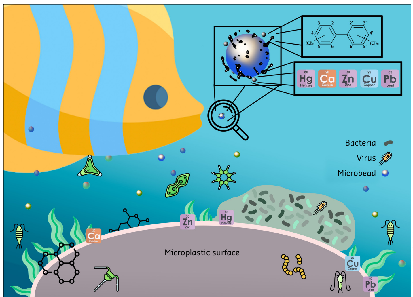
Figure 4.5 Bioaccumulation of organic and inorganic substances to the plastisphere in marine plastics
