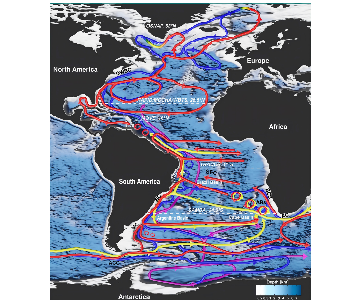
Figure 3.1 Schematic representation of the overturning circulation in the Atlantic Ocean. The figure shows the pathways of surface (red), intermediate (yellow), deep (blue), and abyssal (purple) waters over the bottom topography (blue shading).
