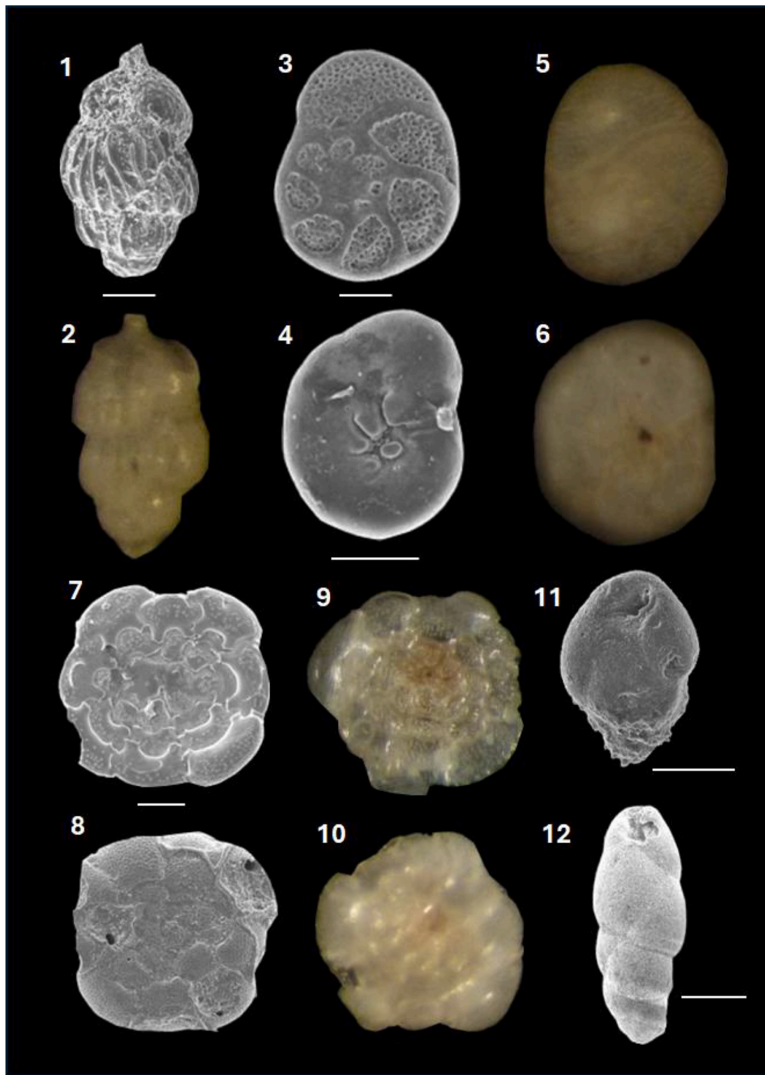
Fig. 6. Pliocene species (cont.). 1–2. Uvigerina peregrina . 3–5. Rosalina bradyi . 4–6. Rosalina bradyi . 7–9. Planorbulina mediterranensis . 8–10. Planorbulina mediterranensis . 11. Bulimina marginata . 12. Bulimina elongata . 2–5–6–9–10: direct photos with binocular magnifying glass. Scale: 100 \mu\text{m} .
