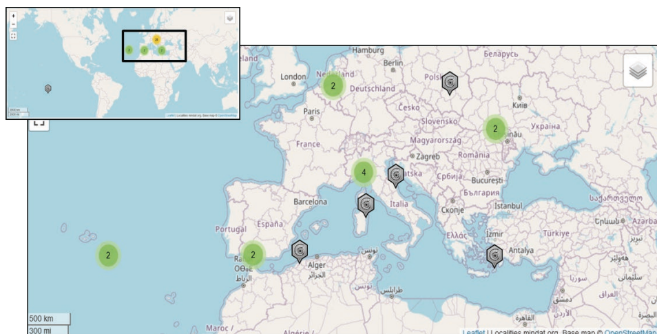
Fig. 3. Fossil findings of the genus Neopycnodonte (Mindat.org, https://www.mindat.org/taxon-2286103.html , October 2023)
