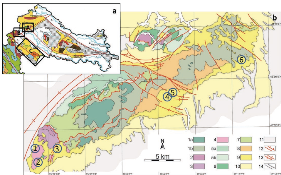
Fig. 5. Findings of Neopycnodonte oysters in north-western and central Croatia: a) Locations of N. cochlear samples housed in the CNHM collections: A. Mt. Medvednica; B. Zaprešić Brijeg; C. Glinsko Pokuplje. Geological map partly after VELIĆ, I. & VELIĆ, J. (1995). b) Field findings of Neopycnodonte on the Mt. Medvednica mentioned by KOCHANSKY (1944). Localities (numbers in circles 1–6): 1–Jarek, 2–Podsusedsko dolje, 3–Bizek, 4–Sv. Barbara, 5–Goranec, 6–Zelina (Zagrad). Geological map after TOMIJENović (2002). Legend: 1a,b. Silurian to Middle Triassic metamorphics; 2–4. Triassic sedimentary rocks; 5 a,b. Mesozoic ophiolites; 6. Aptian to Cenomanian marine sedimentary rocks; 7. Uppermost Cretaceous to Palaeocene rocks; 8. Lower to Middle Miocene freshwater deposits; 9. Middle Miocene dominantly marine deposits ; 10. Upper Miocene brackish deposits; 11. Pliocene freshwater deposits; 12. Tectonic faults; 13. Fold axes; 14. Normal and transgressive boundaries. Gryphaeid oysters were found in the Middle Miocene deposits (9), bolded in the Figure caption and marked by the yellow color on the map.
