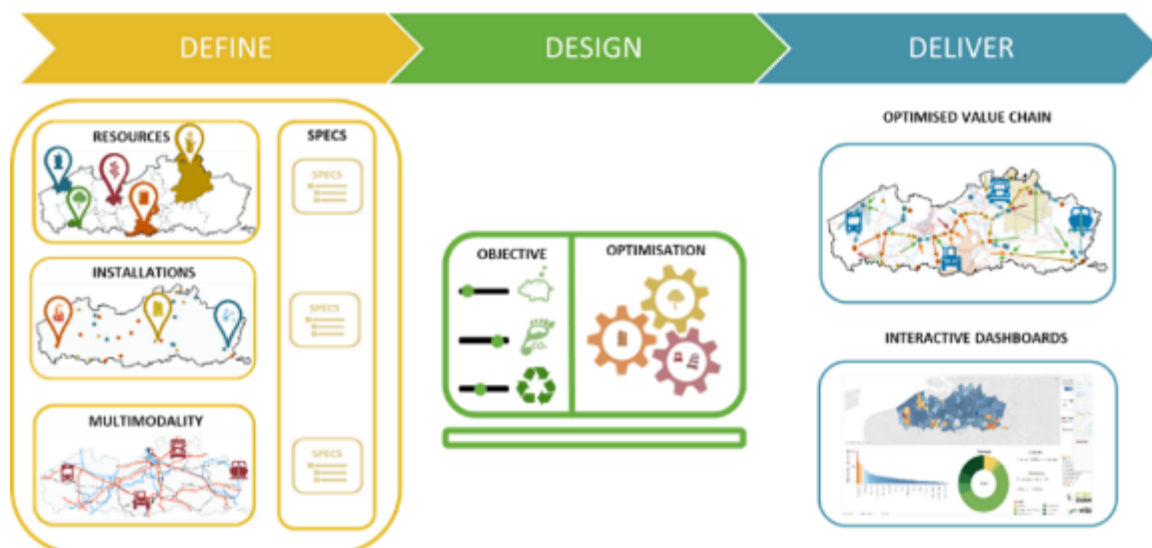
Figure 3 MooV methodology.
