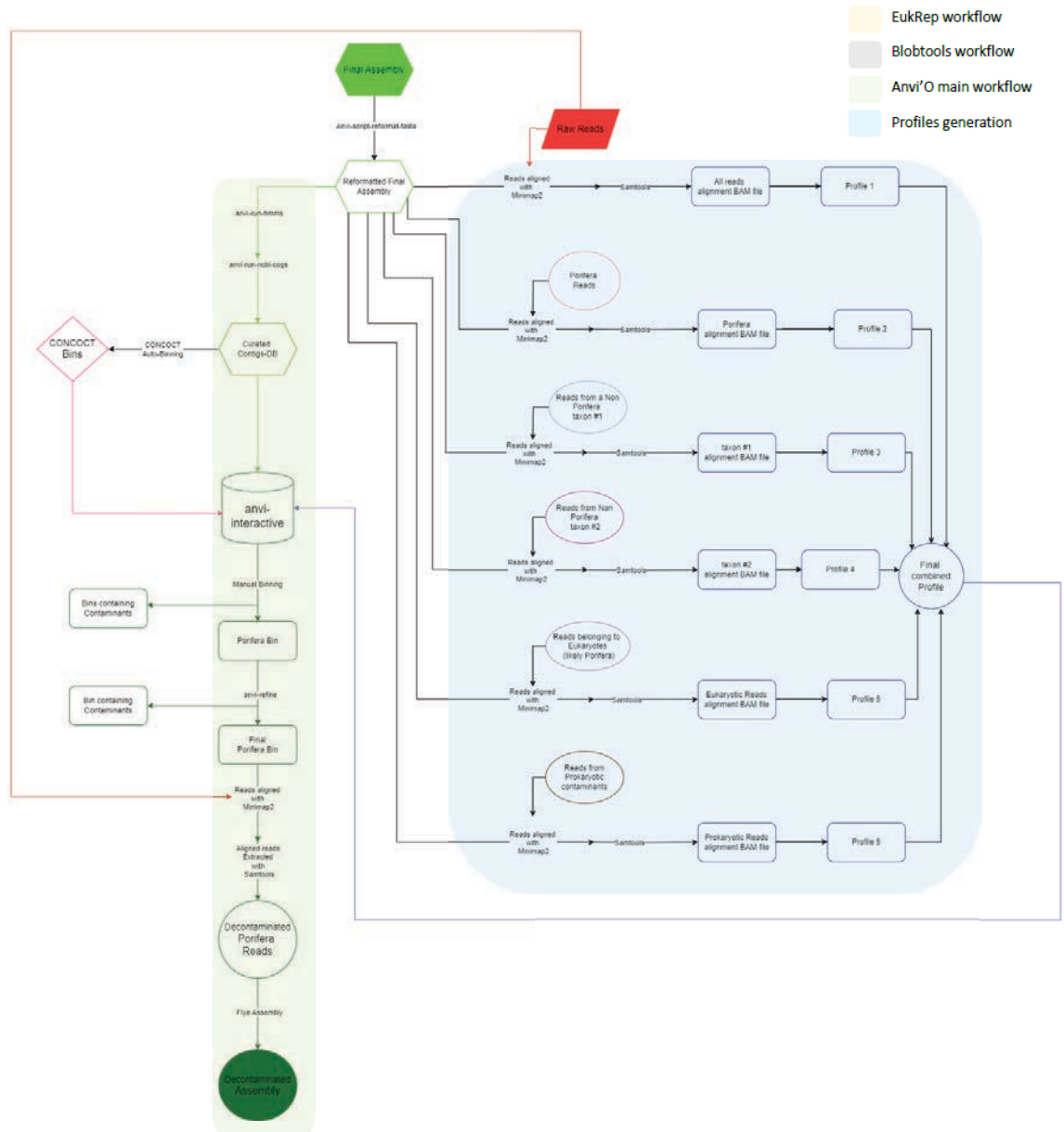
Figure 3. 10, decontamination workflow using Blobtools, EukRep and Anvi'O of Ircana campana sample. First reads belonging to Eukaryotes and Prokaryotes as determined by EukRep along with reads from Porifera and microbial contaminants determined by the Blobtools workflow were extracted (a). These reads were then aligned to the Anvi'O curated assembly to create the interactive cladogram used for manual binning (b). Original drawio files and higher quality versions of these figures are available on GitHub repository: abhiraj1105/workflow .
