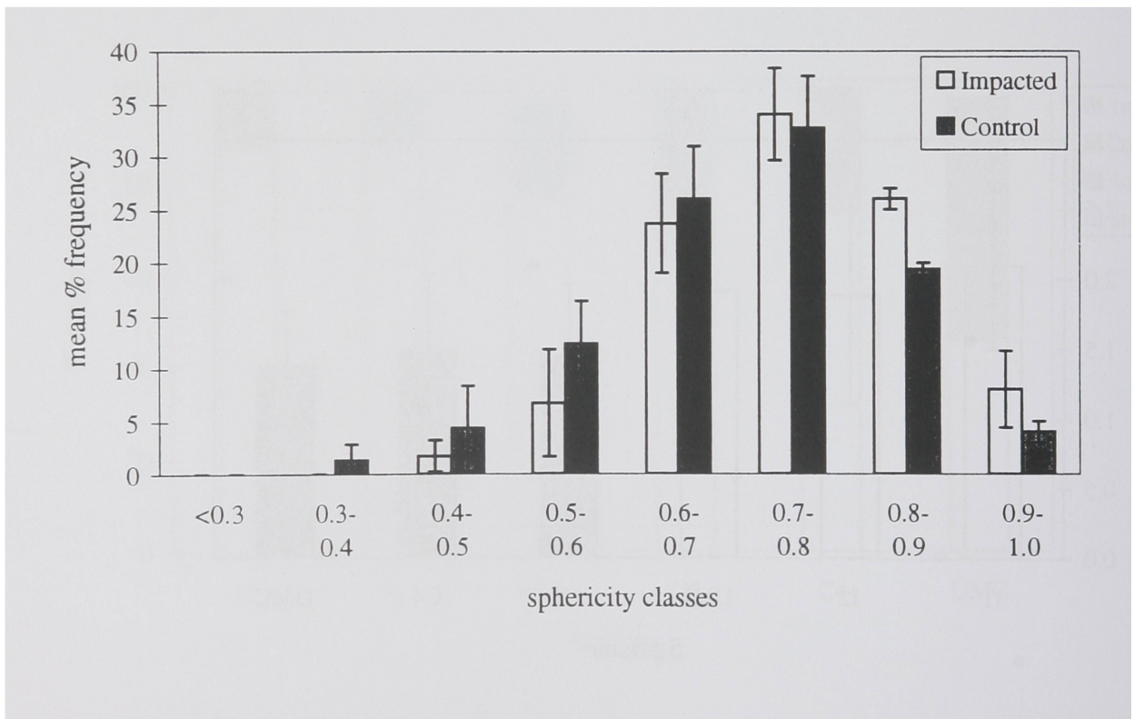
Figure 5 The mean percentage frequency of the rhodoliths in each sphericity class for impacted (I1; I2; UMI) and control stations (C3; C4; UMC). Error bars represent standard deviations.
