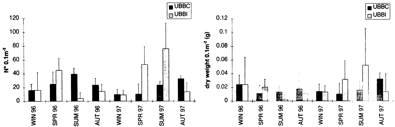
Fig. 3.71. Comparison between control and impacted sites in the Bay of Brest for 1996 and 1997 for N. unicornis .
