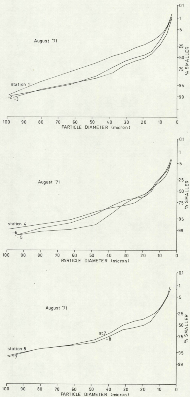
Fig. 2, (Cont.). Cumulative particle size distribution of the non-living fraction of samples collected during the 1971 cruises. See Fig. 1 for location of stations.
