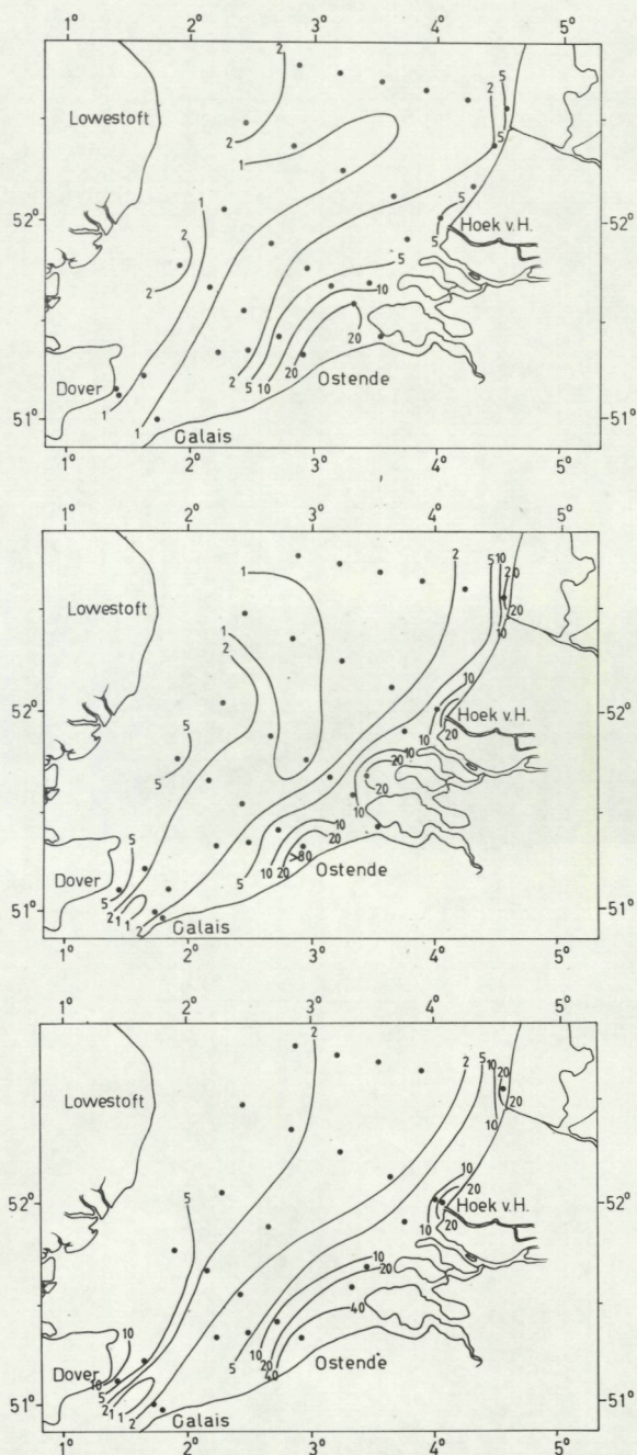
Fig. 6 a-c. Distribution of non-living suspended matter in the size range 3-120 \mu\text{m} , in ppm (by volume; 1 ppm = 1 \text{mm}^3 per liter), JONSDAP cruises 1973. a. 3-7 Sept. 1973 b. 1-5 Oct 1973. c. 29 Oct. - 3 Nov. 1973.
