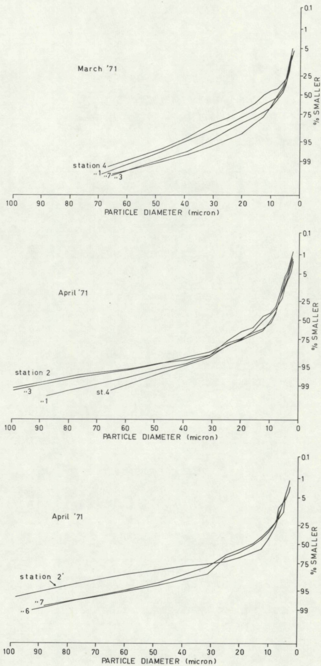
Fig. 2. Cumulative particle size distribution of the non-living fraction of samples collected during the 1971 cruises. See Fig. 1 for location of stations.
