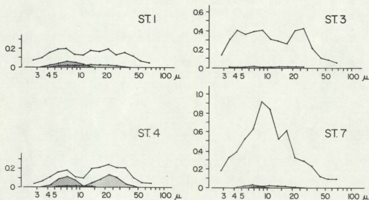
Fig. 1a. Size spectra of suspended particles (surface samples), beginning of March 1971. Abscissa: particle diameter ("equivalent" diameter), \log scale. Ordinate: volume of particles (in ppm by volume; 1 ppm = 1 mm 3 per liter). Upper line in each diagram; all suspended particles (both living and non-living). Hatched: \mu -flagellates only. Dotted: diatoms only.
