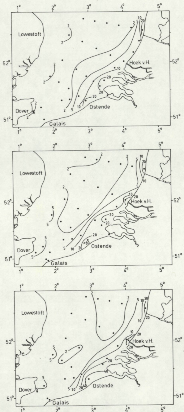
Fig. 5 a-c. Distribution of total suspended matter in the size range 3-120 μm, in ppm (by volume; 1 ppm is 1 mm 3 per liter) during JONSDAP cruises 1973. a. 3-7 Sept. 1975. b. 1-5 Oct. 1973. c. 29 Oct. - 3 Nov. 1973.
