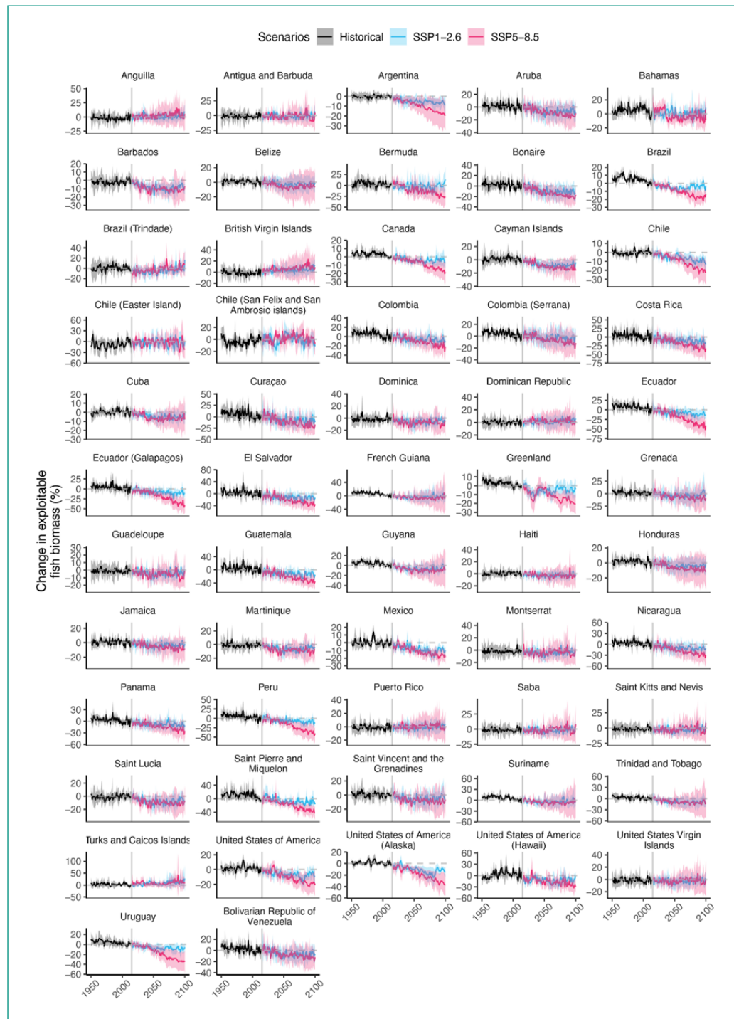
Figure 12. Trends in exploitable fish biomass for countries and territories in the Americas
