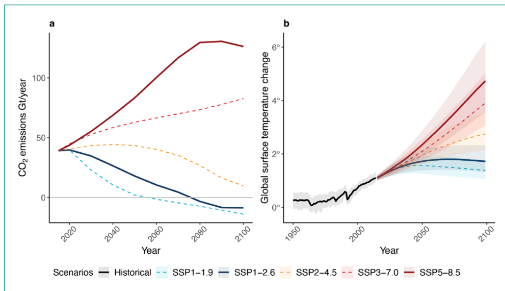
Figure 3. Low and high emissions scenarios in terms of carbon dioxide ( \text{CO}_2 ) emissions and surface temperature trajectories
