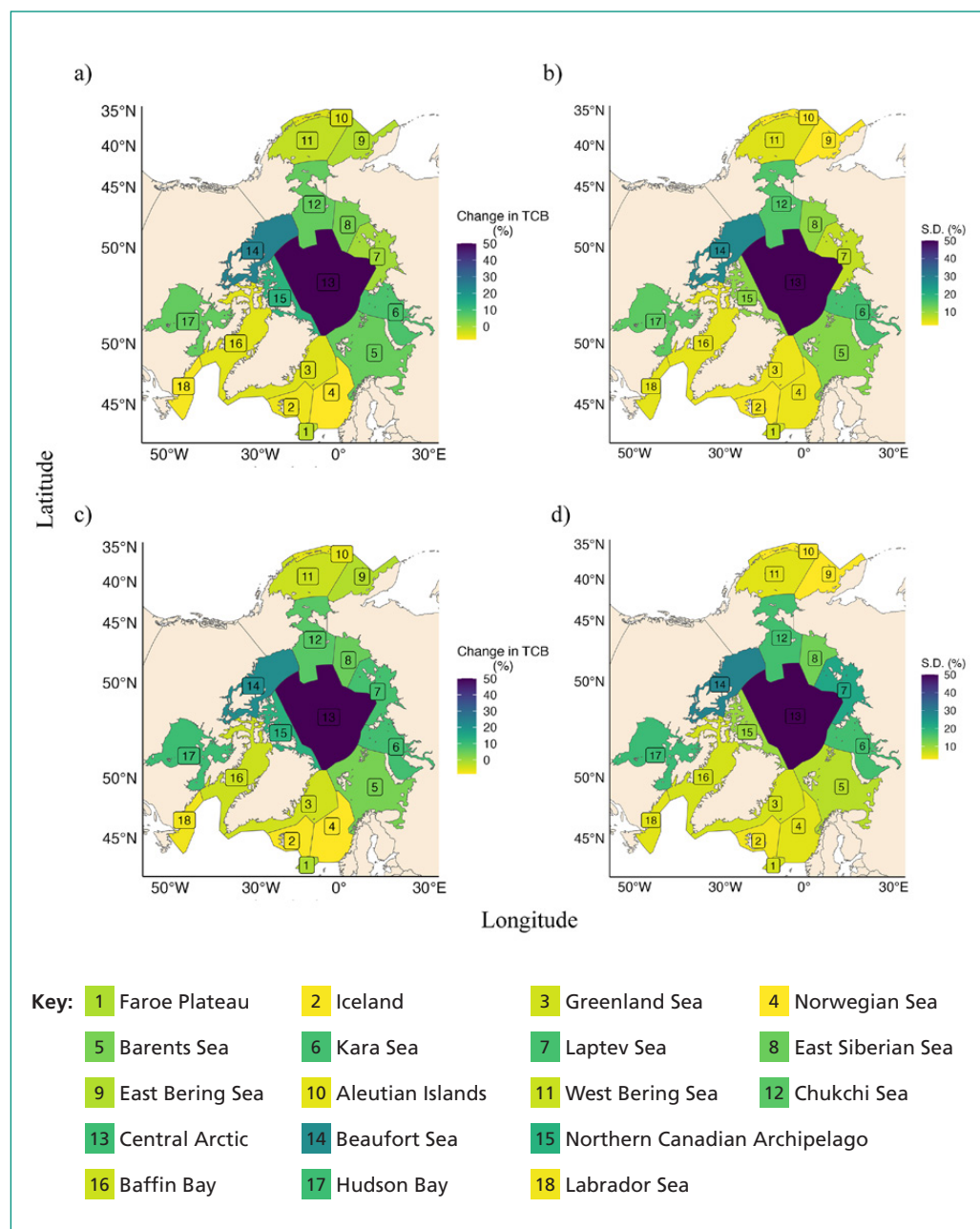
Figure 25. Percentage change in total marine animal biomass for the Arctic
