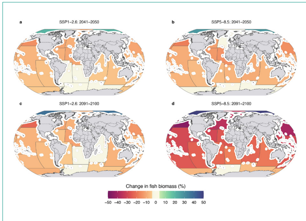
Figure 19. Percentage change in exploitable fish biomass for waters outside national jurisdiction, aggregated into FAO Major Fishing Areas
