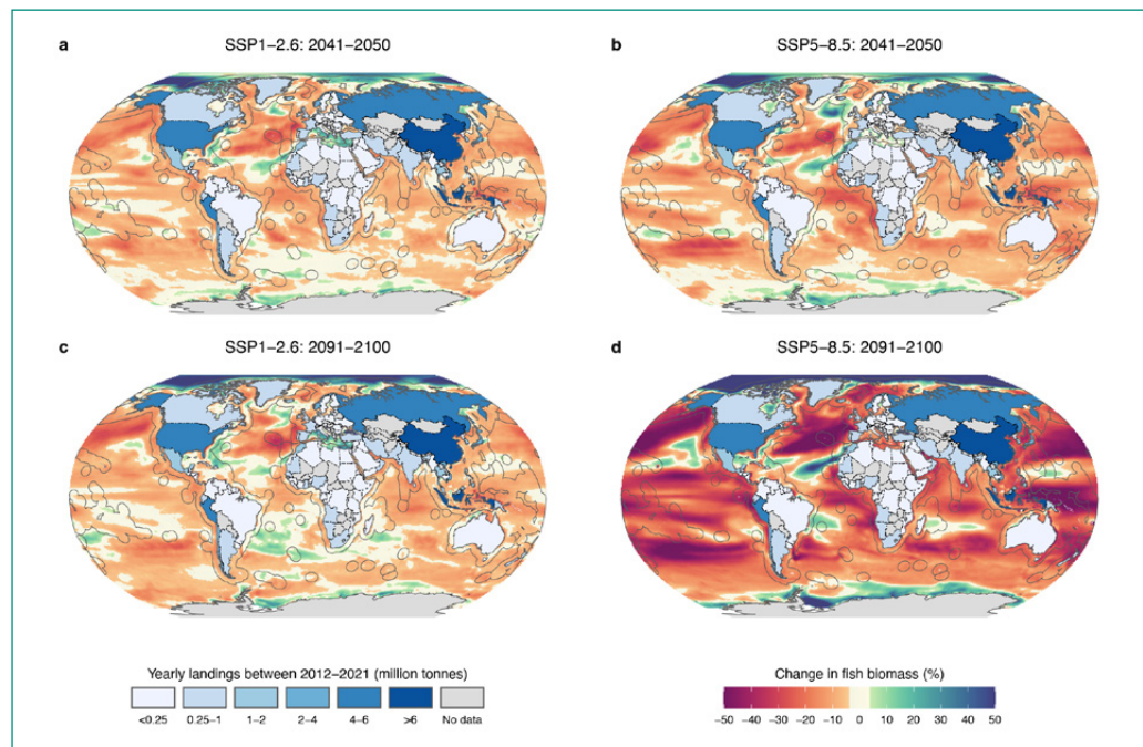
Figure 7. Percentage change in exploitable fish biomass
