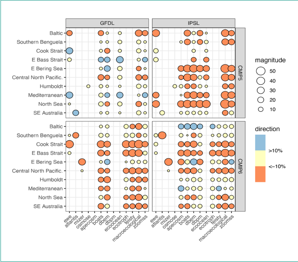
Figure 26. Percentage change in total marine animal biomass across regional and global FishMIP models
