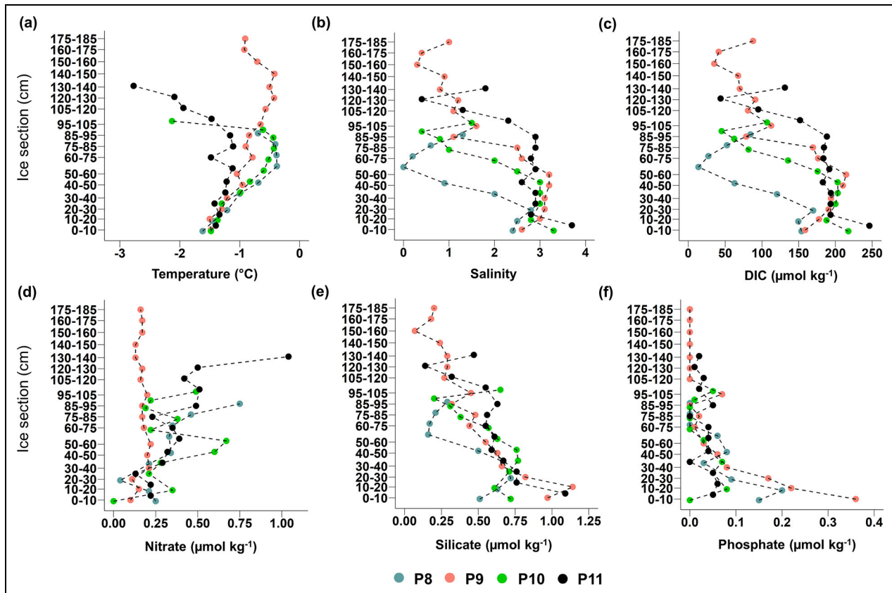
Figure 3. Vertical depth profiles of physico-chemical properties in sea ice. (a) Temperature ( ^{\circ}\text{C} ), (b) bulk salinity, (c) bulk dissolved inorganic carbon (DIC, \mu\text{mol kg}^{-1} ), (d) nitrate ( \mu\text{mol kg}^{-1} ), (e) silicate ( \mu\text{mol kg}^{-1} ), and (f) phosphate ( \mu\text{mol kg}^{-1} ) for different sections of the sea ice (cm) collected at (color-coded) stations P8–P11. The 0–10 cm ice section indicates the ice-water interface. Lengths of the entire ice cores varied by station: 98 cm at P8, 184 cm at P9, 109 cm at P10, and 141 cm at P11. Ice section lengths varied between approximately 10 cm and 15 cm. Values in panels (d–f) are also bulk values. Sea-ice DIC data can be found in Fransson et al. (2025a) and nutrient data are published in Fransson et al. (2025b). Figure prepared in Software R (v4.1.0; R Core Team, 2021), using the ggplot2 package (Wickham, 2016).
