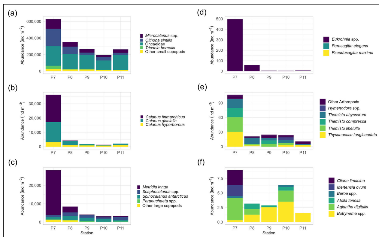
Figure 13. Abundance and composition of zooplankton communities. (a–c) Abundances of the numerically dominant species of mesozooplankton (ind. m -2 ) based on Multinet 64 µm and 180 µm tows, separated into (a) small copepods, (b) Calanus spp., and (c) other large copepods. Abundances of macrozooplankton (ind. m -2 ) based on MIK-net 1,500 µm tows are separated into (d) chaetognaths, (e) arthropods, and (f) molluscs, cnidarians, and ctenophores collected at stations P7–P11. Note the different scales for the different groups. Figure prepared in Software R (v4.2.0; R Core Team, 2021), using the ggplot2 package (Wickham, 2016).
