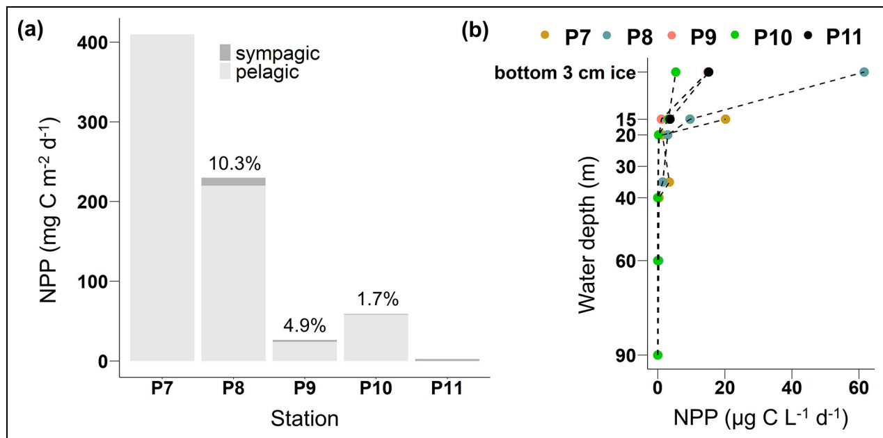
Figure 11. Sympagic and pelagic net primary production. (a) Rates of integrated net primary production (NPP; \text{mg C m}^{-2} \text{ d}^{-1} ) in sea ice (sympagic) and the water column (pelagic) with percentages representing the relative contribution of sea-ice NPP to total NPP for stations where both water and ice values were available (P8–P10), and (b) vertical profiles of NPP ( \mu\text{g C L}^{-1} \text{ d}^{-1} ) collected at (color-coded) stations P7–P11 from the bottom 3 cm of ice to 90 m depth in the water column. In panel (a), sympagic data represent the integrated activity in the lowermost 3 cm of the ice, and pelagic data the integrated activity down to 90 m water depth except for station P11 where only data within the uppermost 15 m were available. Figure prepared in Software R (v4.1.0; R Core Team, 2021), using the ggplot2 package (Wickham, 2016).
