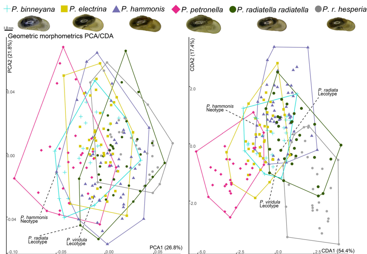
Fig. 3. Position of landmarked Perpolita shells along the first two axes of principal component analysis (PCA) and canonical discriminant analysis (CDA) based on geometric morphometrics of Holarctic Perpolita species. Colours and shapes of each plot indicate species/subspecies and type specimens used in these analyses were labelled individually. See Supplemental Table S4 for information of specimens used in the analyses, Supplemental Dataset S1 for full results of PCA and CDA, and Supplemental Table S5 for the eigen values and the proportion of variances for PCA.
