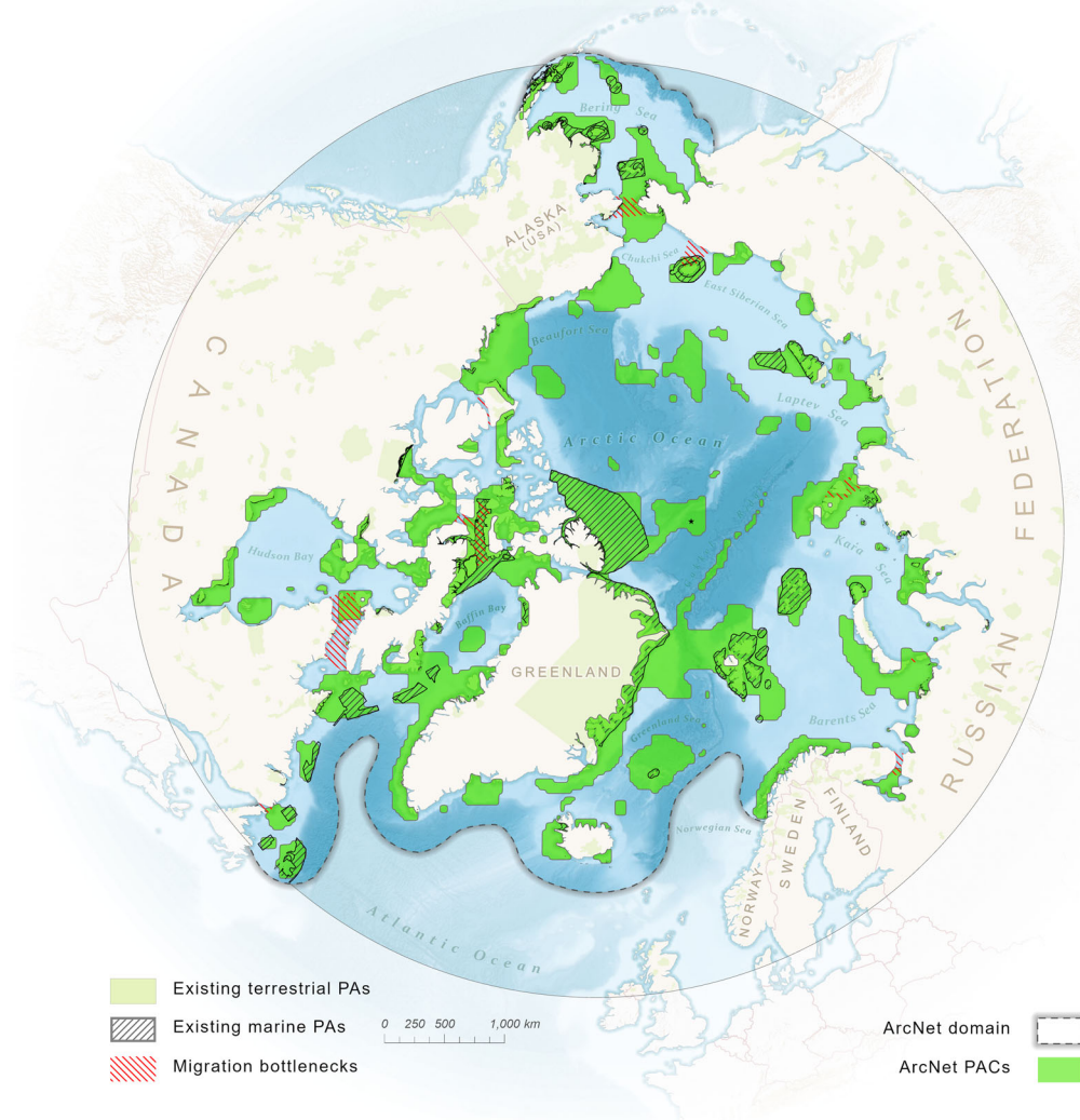
Fig. 1 | The ArcNet domain and PAC network. The ArcNet domain was defined by the southern border of the 18 PAME-defined regions of the Arctic Ocean and adjacent seas, known as the Arctic Large Marine Ecosystems (LMEs) 33 , and focussed on the Arctic realm as defined by the Marine Ecoregions of the World 58 , with some
