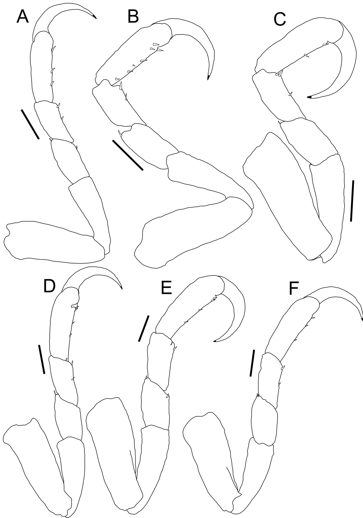
Fig. 12. Pereopods 7 of aegathoid stages of Anilocra prionuri Williams and Bunkley-Williams, 1986 collected from a scalpel sawtail, Prionurus scalprum Valenciennes, 1835. A–F, SML-V0772–V0777 (BL14.2, 14.4, 14.8, 15.5, 17.6, and 18.0 mm). Scale bar = 0.5 mm.
