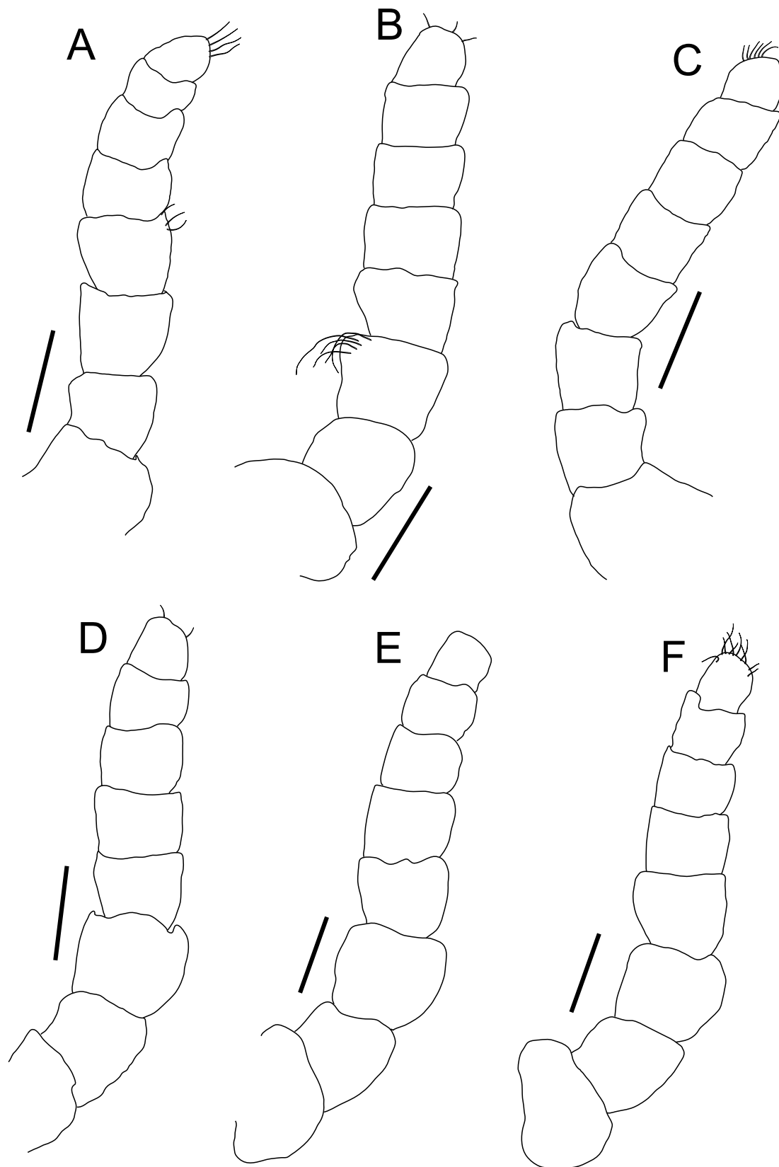
Fig. 8. Antennules of aegathoid stages of Anilocra prionuri Williams and Bunkley-Williams, 1986 collected from a scalpel sawtail, Prionurus scalprum Valenciennes, 1835. A–F, SML-V0772–V0777 (BL14.2, 14.4, 14.8, 15.5, 17.6, and 18.0 mm). Scale bar = 0.3 mm.
