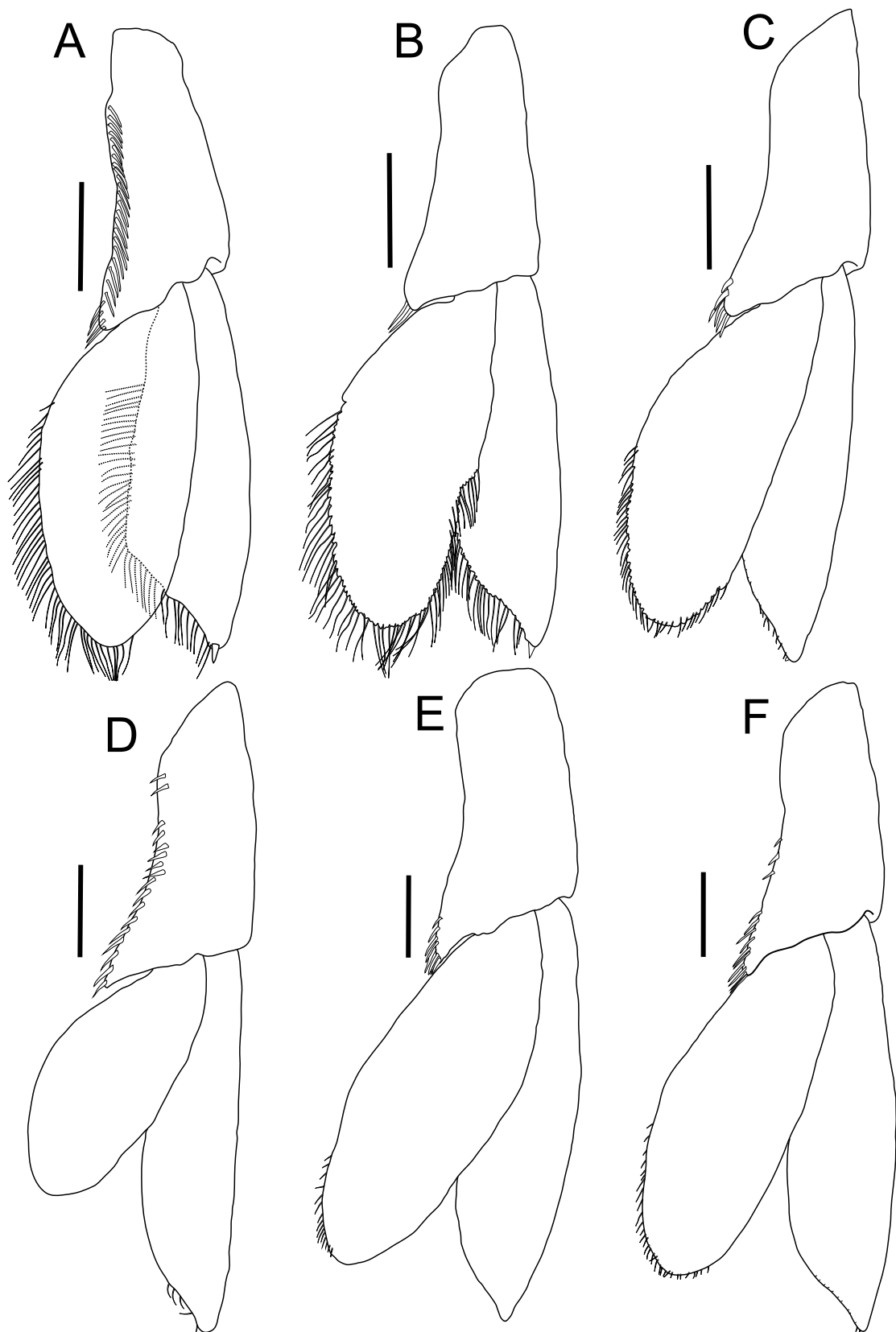
Fig. 18. Uropods of aegathoid stages of Anilocra prionuri Williams and Bunkley-Williams, 1986 collected from a scalpel sawtail, Prionurus scalprum Valenciennes, 1835. A–F, SMBL-V0772–V0777 (BL14.2, 14.4, 14.8, 15.5, 17.6, and 18.0 mm). Scale bar = 0.5 mm.
