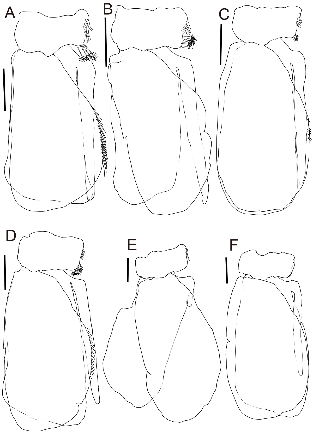
Fig. 16. Pleopods 2 of aegathoid stages of Anilocra prionuri Williams and Bunkley-Williams, 1986 collected from a scalpel sawtail, Prionurus scalprum Valenciennes, 1835. A–F, SMBL-V0772–V0777 (BL14.2, 14.4, 14.8, 15.5, 17.6, and 18.0 mm). Scale bar = 0.5 mm.
