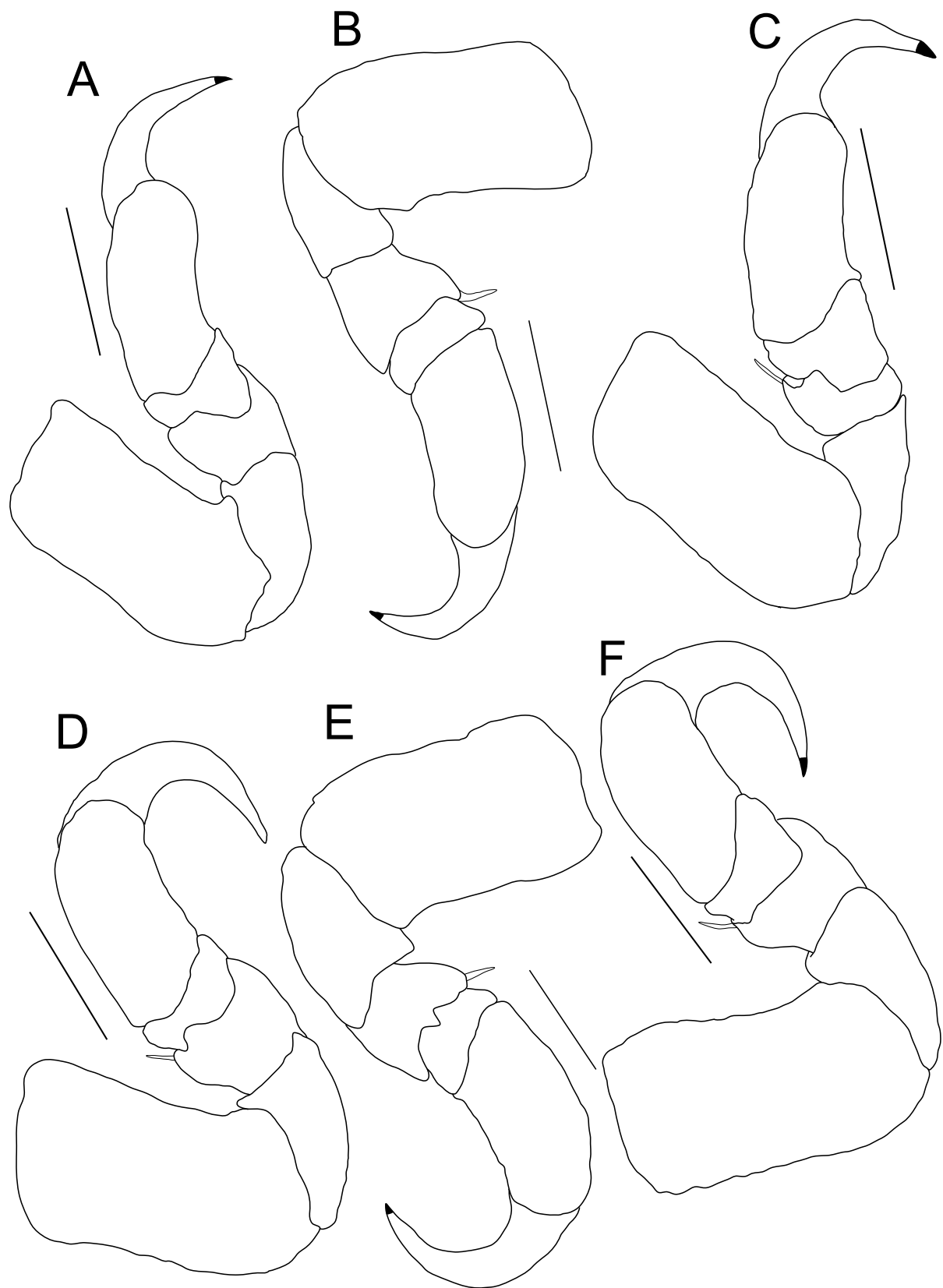
Fig. 10. Pereopods 1 of aegathoid stages of Anilocra prionuri Williams and Bunkley-Williams, 1986 collected from a scalpel sawtail, Prionurus scalprum Valenciennes, 1835. A–F, SMBL-V0772–V0777 (BL14.2, 14.4, 14.8, 15.5, 17.6, and 18.0 mm). Scale bar = 0.5 mm.
