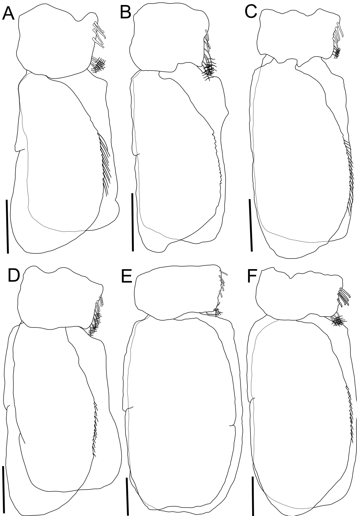
Fig. 14. Pleopods 1 of aegathoid stages of Anilocra prionuri Williams and Bunkley-Williams, 1986 collected from a scalpel sawtail, Prionurus scalprum Valenciennes, 1835. A–F, SML-V0772–V0777 (BL14.2, 14.4, 14.8, 15.5, 17.6, and 18.0 mm). Scale bar = 0.5 mm.
