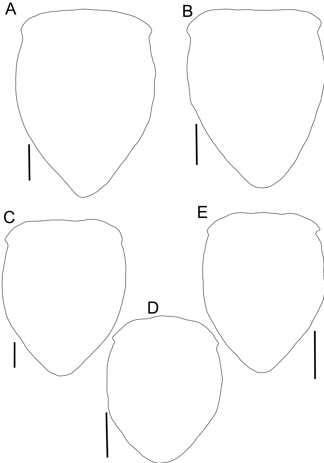
Fig. 7. Pleotelsons of Anilocra prionuri Williams and Bunkley-Williams, 1986 collected from a scalpel sawtail, Prionurus scalprum Valenciennes, 1835. A, B, males SMBL-V0778, V0779 (BL20.0 and 20.1 mm); C, SMBL-V0780, transitional (BL24.7 mm); D, E, SMBL-V0781, V0782, ovigerous females (BL34.0 and 34.2 mm). Scale bar: A–C = 1 mm; D, E = 3 mm.
