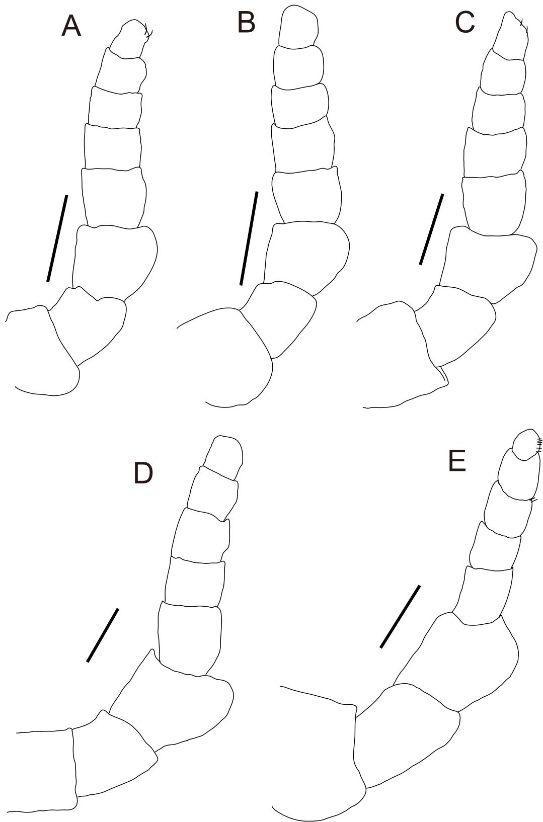
Fig. 9. Antennules of Anilocra prionuri Williams and Bunkley-Williams, 1986 collected from a scalpel sawtail, Prionurus scalprum Valenciennes, 1835. A, B, males SMBL-V0778, V0779 (BL20.0 and 20.1 mm); C, SMBL-V0780, transitional (BL24.7 mm); D, E, SMBL-V0781, V0782, ovigerous females (BL34.0 and 34.2 mm). Scale bar = 0.5 mm.
