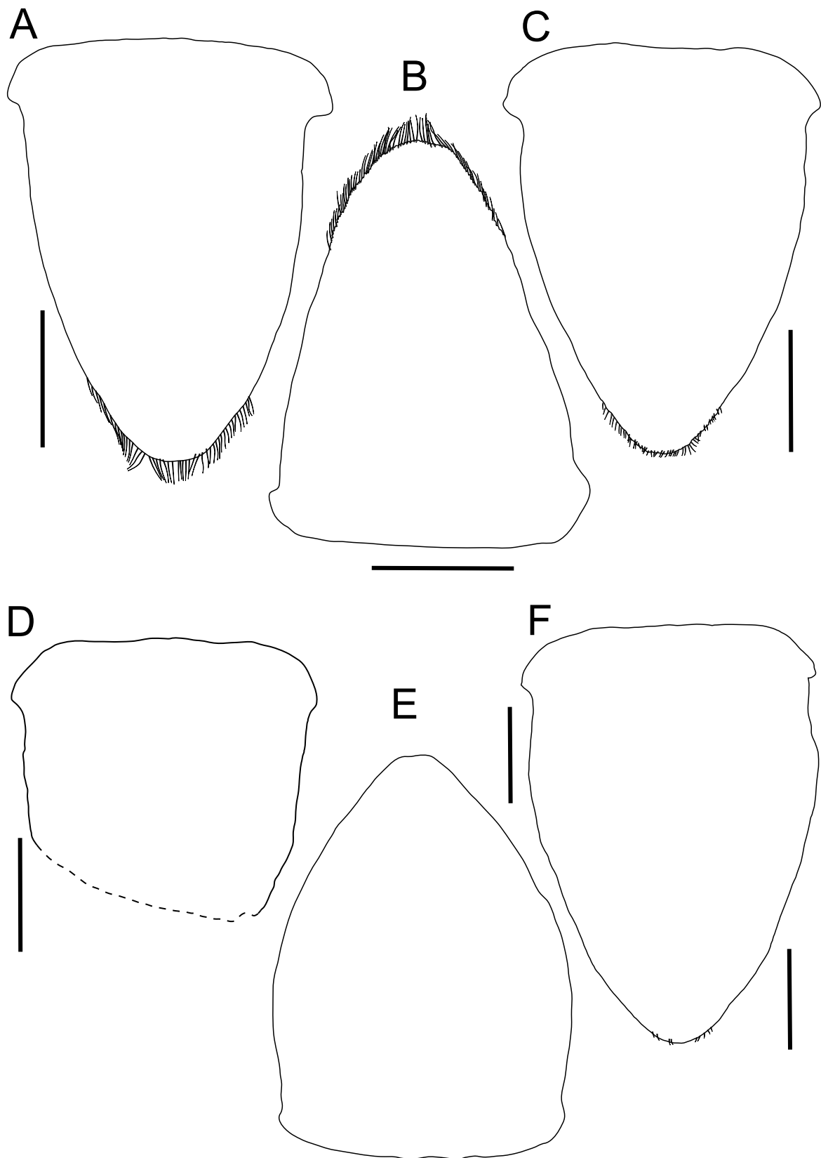
Fig. 6. Pleotelsons of aegathoid stages of Anilocra prionuri Williams and Bunkley-Williams, 1986 collected from a scalpel sawtail, Prionurus scalprum Valenciennes, 1835. A–F, SMBL-V0772–V0777 (BL14.2, 14.4, 14.8, 15.5, 17.6, and 18.0 mm). Scale bar = 1 mm.
