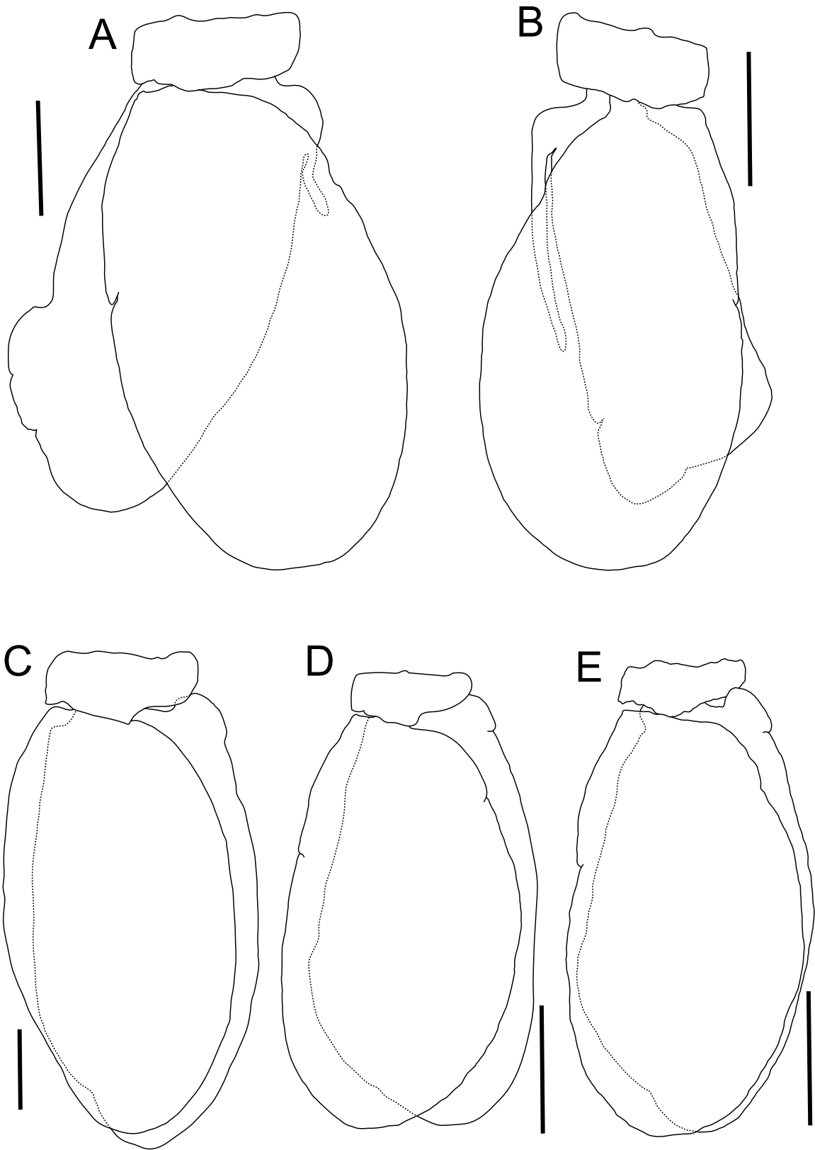
Fig. 17. Pleopods 2 of Anilocra prionuri Williams and Bunkley-Williams, 1986 collected from a scalpel sawtail, Prionurus scalprum Valenciennes, 1835. A, B, males SMBL-V0778, V0779 (BL20.0 and 20.1 mm); C, SMBL-V0780, transitional (BL24.7 mm); D, E, SMBL-V0781, V0782, ovigerous females (BL34.0 and 34.2 mm). Scale bar: A–C = 1 mm; D, E = 3 mm.
