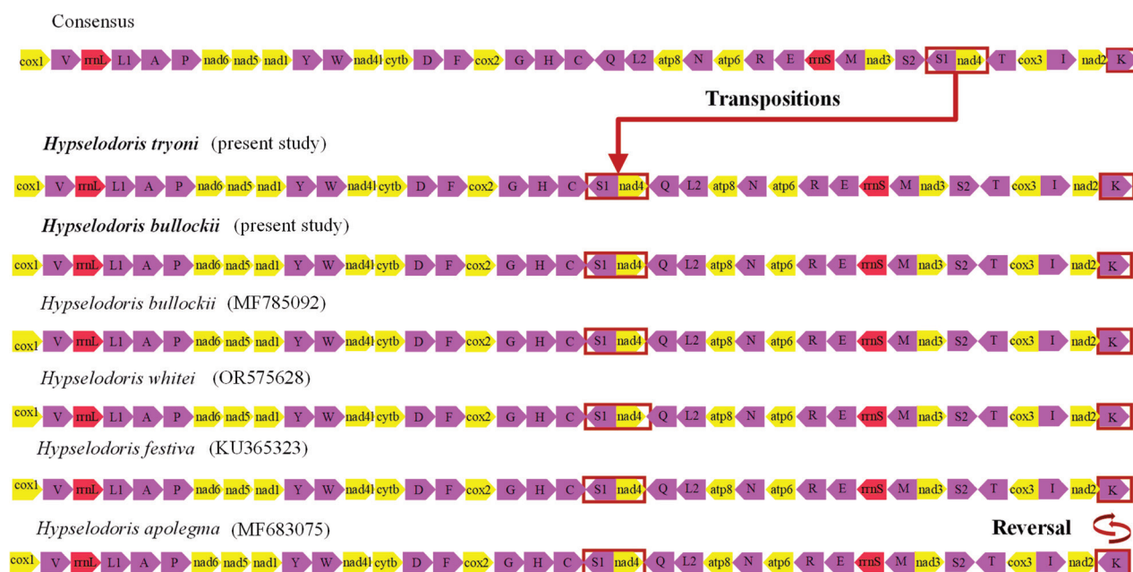
Figure 5. Mitochondrial gene rearrangements of nudibranchs.
