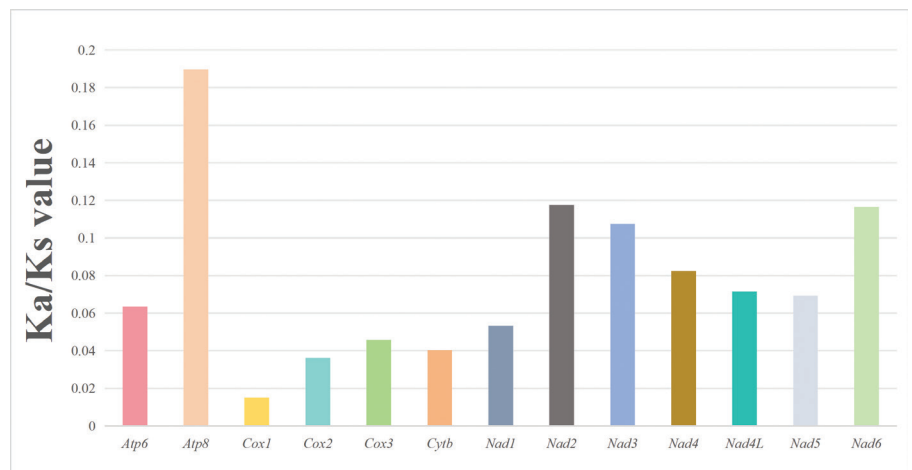
Figure 3. The Ka/Ks ratios of the 13 different mitochondrial genes in nudibranchs.
