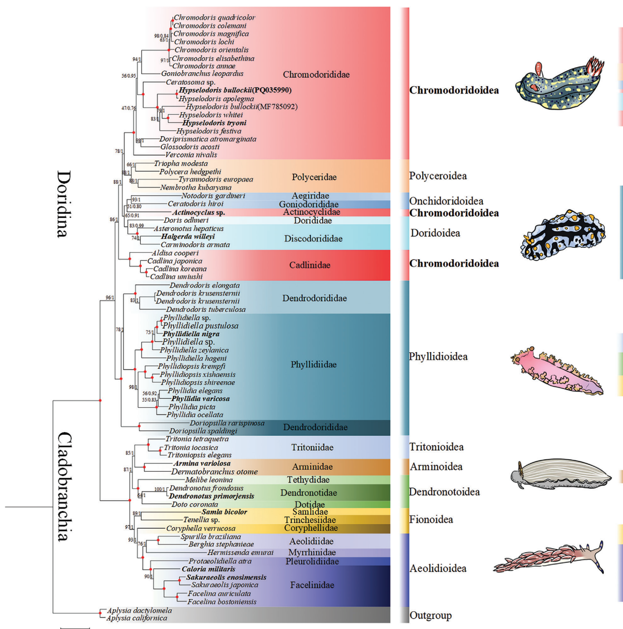
Figure 6. Phylogenetic relationships based on concatenated 13 mitochondrial PCGs and two mitochondrial rRNA genes, with Aplysia californica and A. dactylomela as outgroups. The first number on each node is the bootstrap proportion (BP) of the maximum likelihood (ML) analysis. The second number is the Bayesian posterior probability (PP). Nodes with maximum statistical support (BP = 100; PP = 1) are marked with red solid circles. The 11 newly sequenced mitochondrial genomes and the paraphyletic group Chromodoridoidea are in bold.
