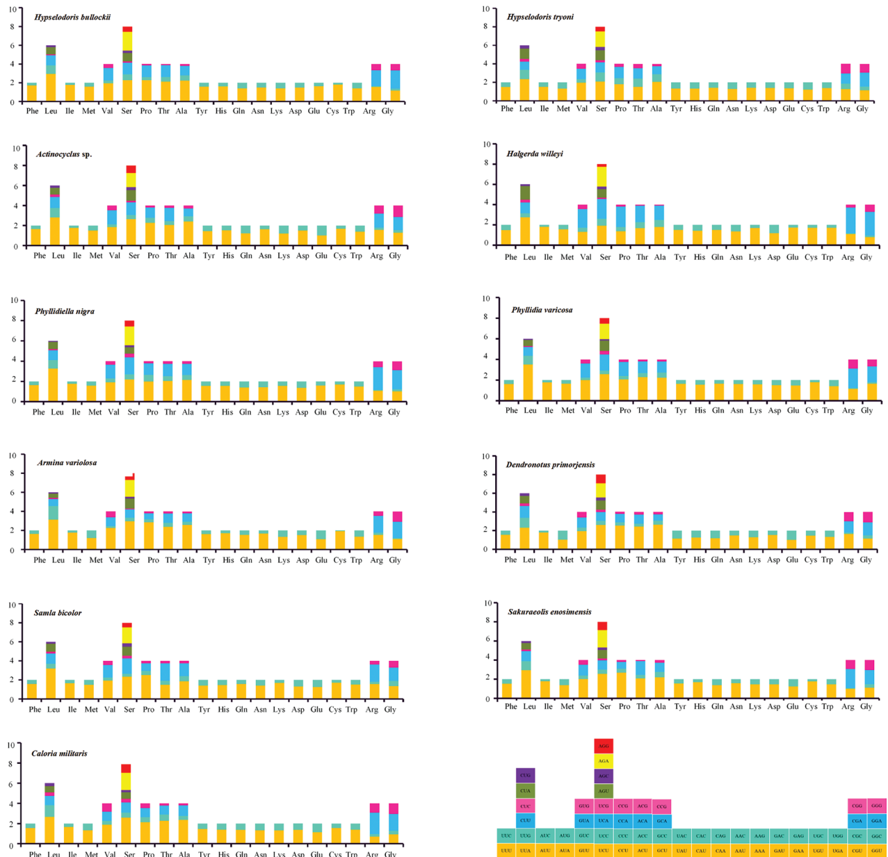
Figure 2. Relative synonymous codon usage (RSCU) for 11 nudibranch species.
