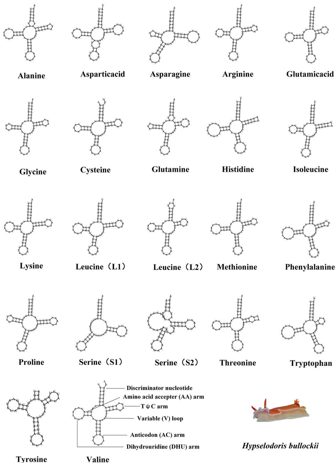
Figure 4. Inferred secondary structures of 22 transfer RNAs (tRNAs) represented by Hypselodoris bullockii .
