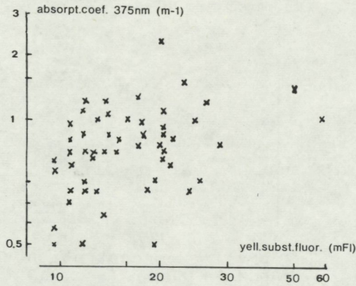
Fig. 6. Relationship between absorption and fluorescence of the yellow substances for 1981 tower experiment ( r = 0.09 , n = 56 ).
