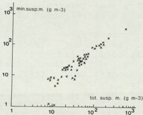
Fig. 5. Suspended mineral matter concentration versus TSM concentration for 1981 tower experiment ( r=0.92 , n=56 ).
