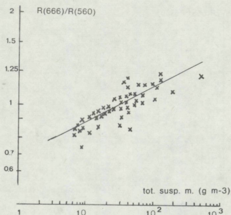
Fig. 10. Reflectance ratio versus total suspended matter concentration for 1981 tower experiment on waters ( r=0.87 , n=48 points ).
