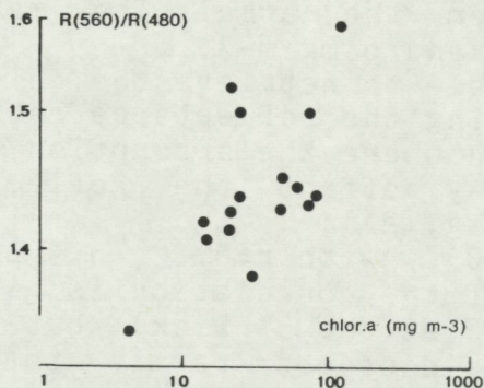
Fig. 22. Reflectance ratio versus chlorophyll a concentration for 1981 airplane experiment on tidal flat ( r=0.63 , n=16 ).
