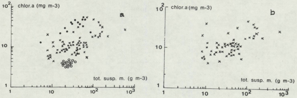
Fig. 6a. Chlorophyll a concentration versus total suspended matter concentration for 1981 experiment ( r=0.64 , n=56 ). b. Chlorophyll a concentration versus total suspended matter concentration for all the experiments: 1981 tower (x) and airplane (●), 1982 airplane (o), ( r=0.50 , n=86 ).
