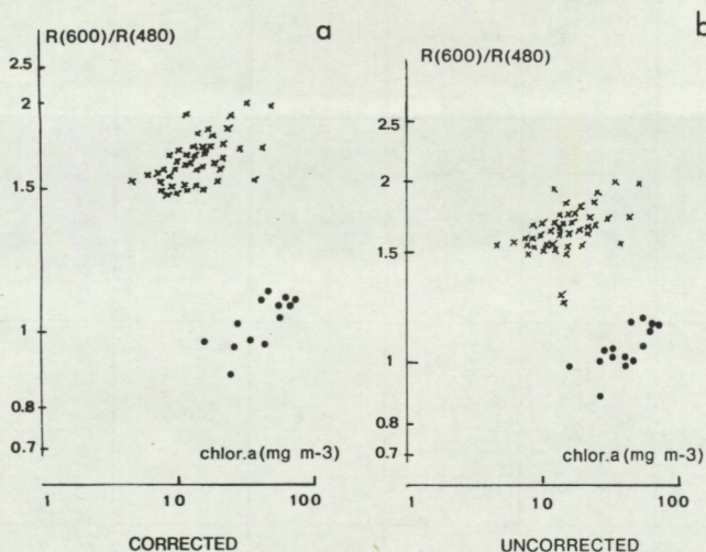
Fig. 23. Different reflectance ratios "red/ blue" versus chlorophyll a concentration for waters for 1981 airplane (o) and tower (x) experiments: a. with corrected; b. with uncorrected reflectances from the sky glitter.
