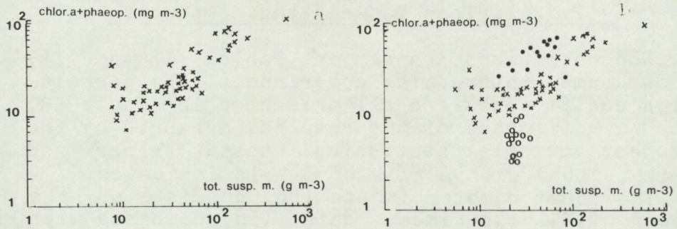
Fig. 3.a. Pigment concentration versus total suspended matter concentration for 1981 tower experiment ( r=0.82 , n=56 ). b. Pigment concentration versus total suspended matter concentration for all experiments: 1981 tower (x) and airplane(●), 1982 airplane(o), ( r=0.64 , n=86 ).
