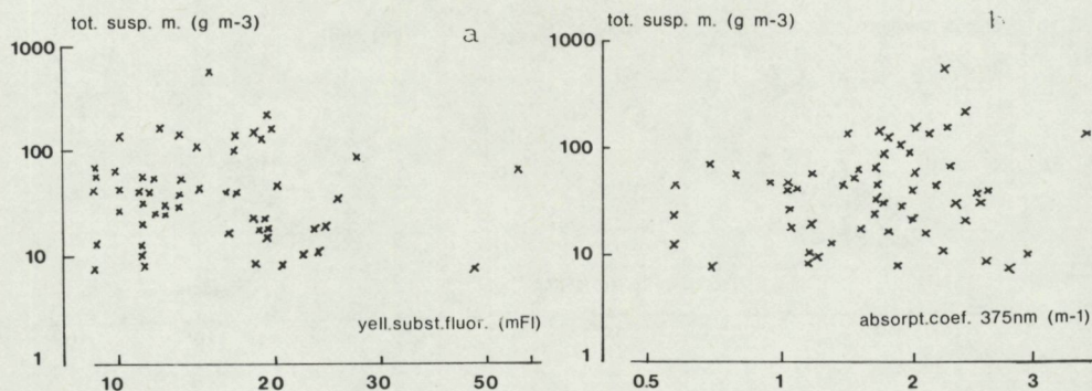
Fig. 8a. Total suspended matter versus yellow substance fluorescence for 1981 tower experiment ( r=-0.08 , n=56 ). b. Total suspended matter concentration versus absorption coefficient at 375 nm for 1981 experiment ( r=0.17 , n=56 ).
