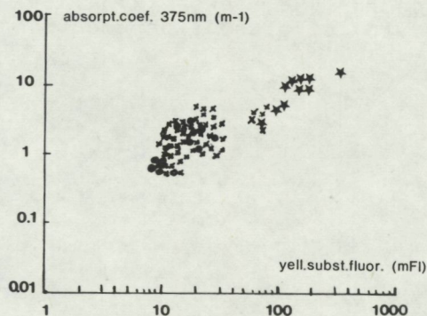
Fig. 7. Relation between absorption and fluorescence of the yellow substances for waters : 1981 tower (x), 1981 and 1982 airplane ( \bullet , \circ ), and for the tidal flat with interstitial waters (*), in log coordinates ( r = 0.879 , n = 104 ).
