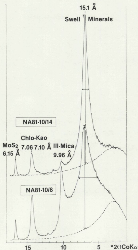
Fig. 2. Width at half peak height of Swell Minerals (combined swelling clay minerals) and the "d" spacings of Ill/Mica (illite/mica), Chlo/Kao (combined chlorite and kaolinite) and \text{MoS}_2 (internal standard) at 50% relative humidity.
