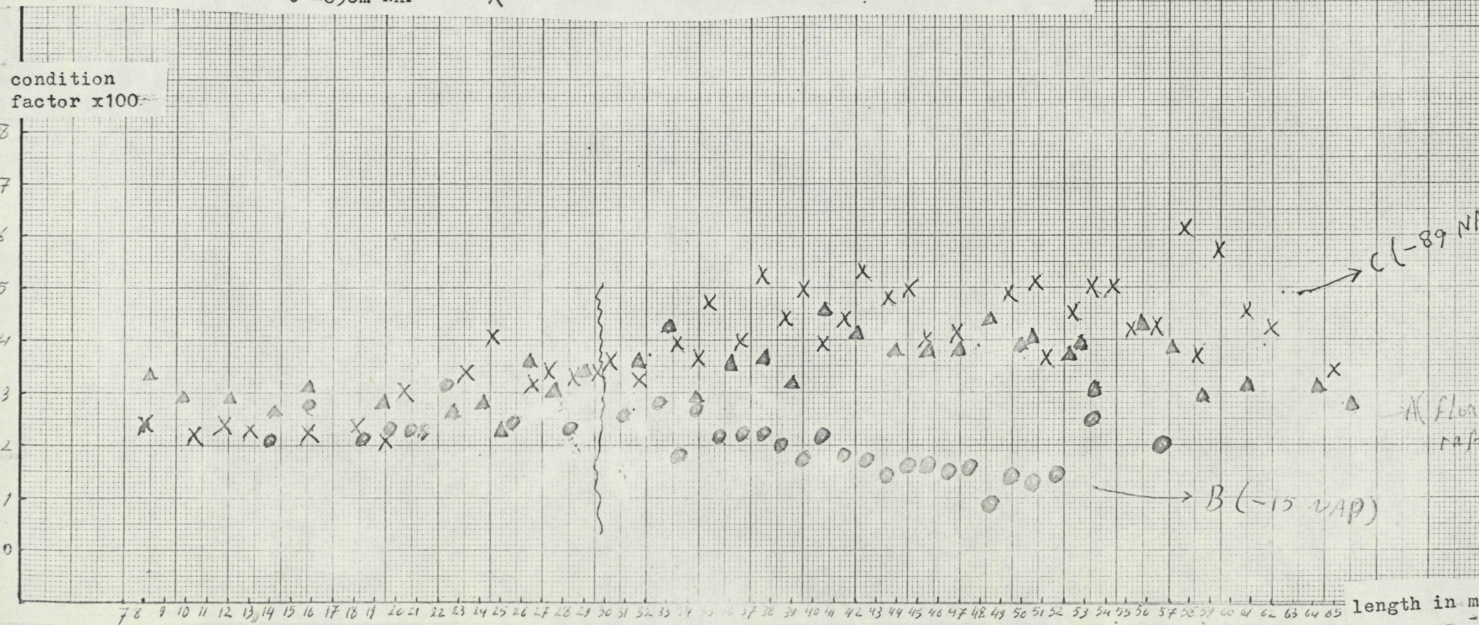
Figure 5 b . Condition factor as a function of length for the mussels from three samples: A floating raft \blacktriangle Condition factor defined as \text{weight} / \text{L.H.W} B -15cm NAP \bullet C -89cm NAP \times
