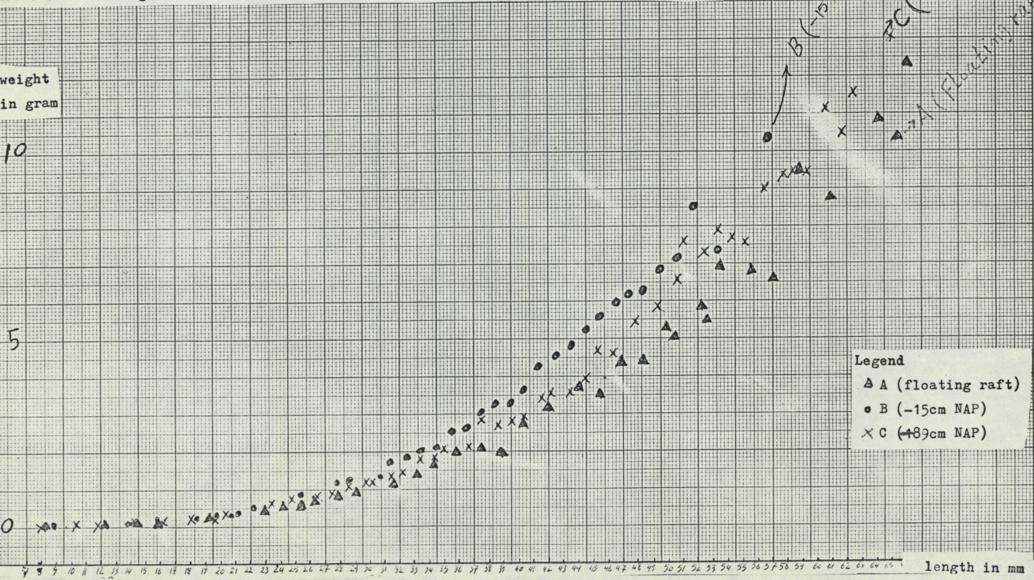
Figure 8 a . Shell weight as a function of shell length in mussels from three levels.
