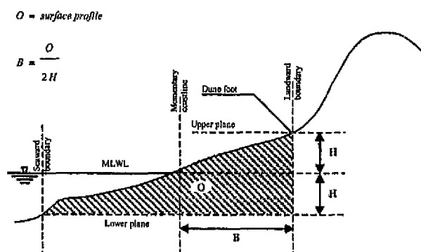
Figure 3.2.6. Calculation method Momentary Coastline (MCL)
