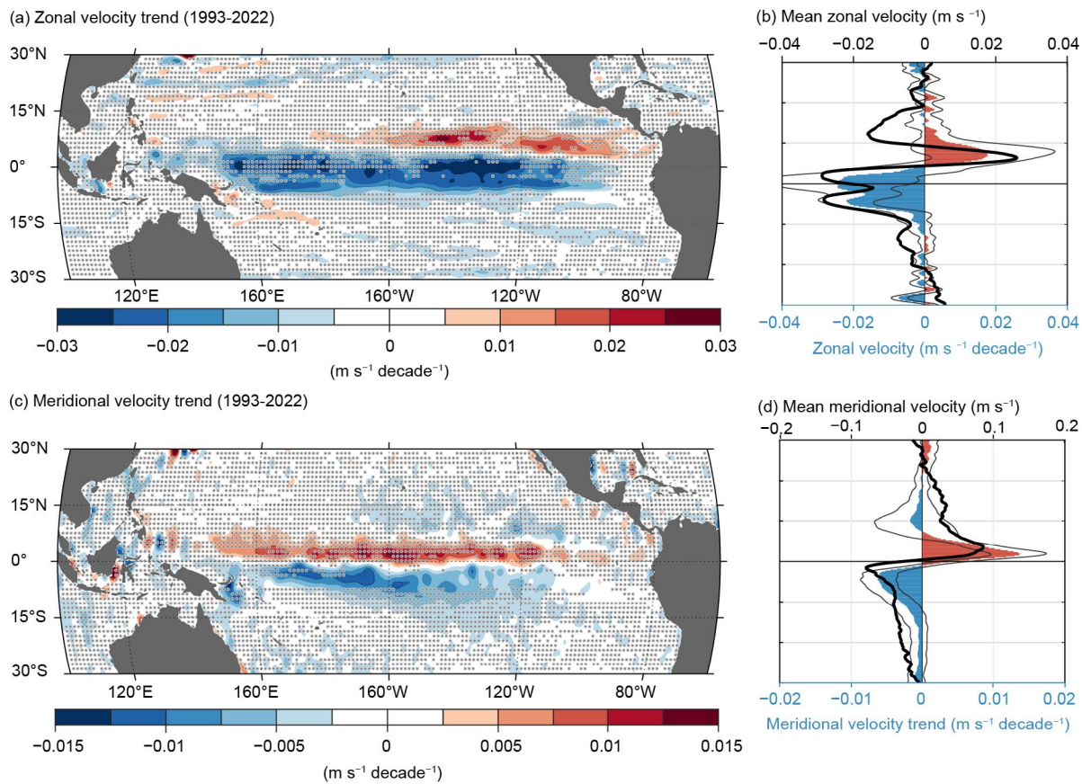
Fig. 3.21. (a) Surface zonal total velocity trend ( \text{m s}^{-1} \text{ decade}^{-1} ) between 1993 and 2022 in the tropical Pacific. Regions where trends are not significantly different from zero at 97.5% confidence are stippled. (b) Zonally averaged ( 100^{\circ}\text{W} – 170^{\circ}\text{W} ) mean surface zonal velocity (black line) and surface zonal velocity trend (colored bars) as functions of latitude. Thin black lines indicate the 2.5%–97.5% confidence intervals on the trend. (c) and (d) Same as (a) and (b) but for total meridional velocity.
