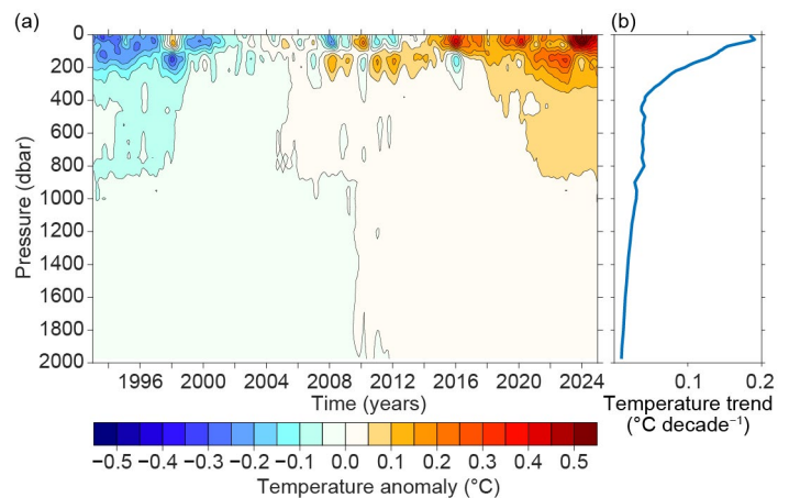
Fig. 3.6. (a) Near-global (66.5°S–81.5°N, but excluding seasonally ice-covered regions within that latitude range) average monthly ocean temperature anomalies ( ^{\circ}\text{C} ; from Random Forest Regression Ocean Maps [RFROM] v2.2, Lyman and Johnson [2023]) relative to 1993–2022 average monthly values, smoothed with a five-month Hanning filter and contoured at 0.05^{\circ}\text{C} intervals (see color bar) vs. pressure and time. (b) Linear trend of temperature anomalies over the period 2004–24 in (a) plotted vs. pressure in ^{\circ}\text{C decade}^{-1} (blue line) with 5%–95% confidence intervals (light blue shading).
