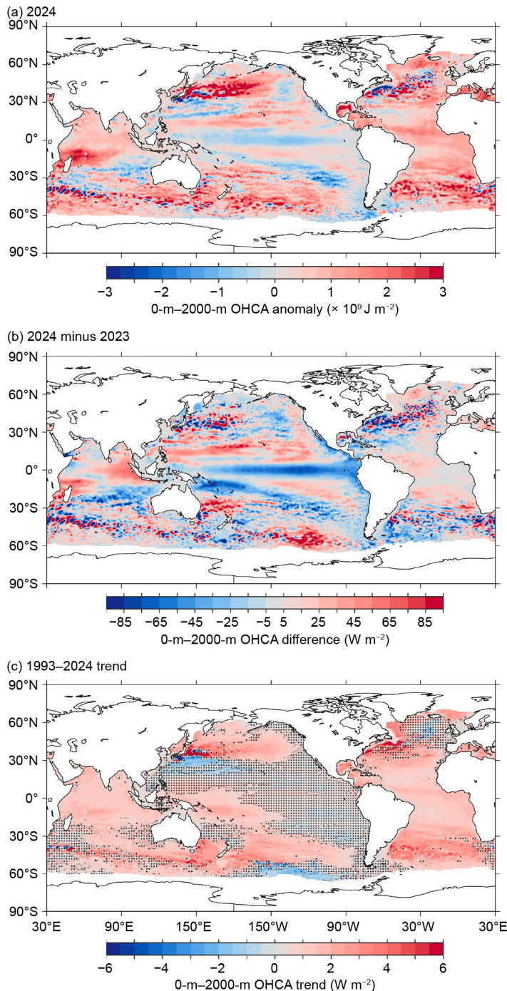
Fig. 3.5. (a) Random Forest Regression Ocean Maps (RFROM) v2 estimate of 0-m–2000-m ocean heat content anomaly (OHCA; \times 10^9 \text{ J m}^{-2} ) for 2024 analyzed following Lyman and Johnson (2023) with v2.2 improvements as in https://www.pmel.noaa.gov/rfrom/ . Values are displayed relative to a 1993–2022 baseline. (b) 2024-minus-2023 of 0-m–2000-m OHCA expressed as a local surface heat flux equivalent ( \text{W m}^{-2} ). For (a) and (b) comparisons, note that 95 \text{ W m}^{-2} applied over one year results in a 3 \times 10^9 \text{ J m}^{-2} change of OHCA. (c) Linear trend for 1993–2024 0-m–2000-m annual OHCA ( \text{W m}^{-2} ). Areas with statistically insignificant trends at 5%–95% confidence (taking into account the decorrelation time scale of the residuals when estimating effective degrees of freedom) are stippled.
