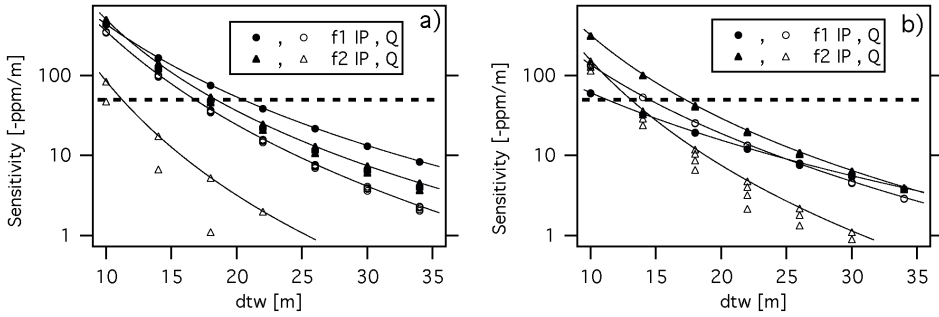
Figure 2. AWI bird sea ice thickness sensitivities for a) Arctic/Antarctic and b) Baltic conditions versus system distance to water (dtw), for both homogeneous half-space models with dtw = \text{bird height } (h) (line) and suites of two layer cases for dtw = \text{ice thickness} + h (markers). The dashed line is at a potential noise level threshold of \sim 50 \text{ ppm/m} (10 cm resolution at 5 ppm ambient noise).
