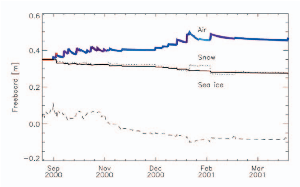
Figure 2. The simulated accumulation of snow in a single profile at 82.5°N 0.0°E during winter 2000/2001. The dashed line show the penetration depth at Ku-band and the dotted line show the depth of the effective scattering surface. The full line is the snow/ice interface. The colours of the snow surface line indicate the snow surface density.
