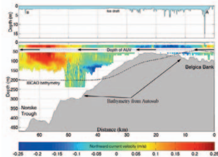
(a) The outward track of an Autosub mission off NE Greenland 21-22 August 2004, run at 40 m depth. The top profile is ice draft measured at crude resolution by upward-looking ADCP. Note smooth undeformed ice over Norske Trough. The bottom profile is the seabed topography measured by Autosub compared with the IBCAO bathymetry (dashed line). The coloured masses are N-S velocity components measured by the downward looking ADCP aboard Autosub. The red area is a strong northward current in the Trough, the Northeast Greenland Coastal Current (NEGCC); the blue area is a hitherto unrecognised southward current on the western flank of Belgica Bank. This image displays graphically the extra value obtained by carrying a number of oceanographic instruments on the AUV.
