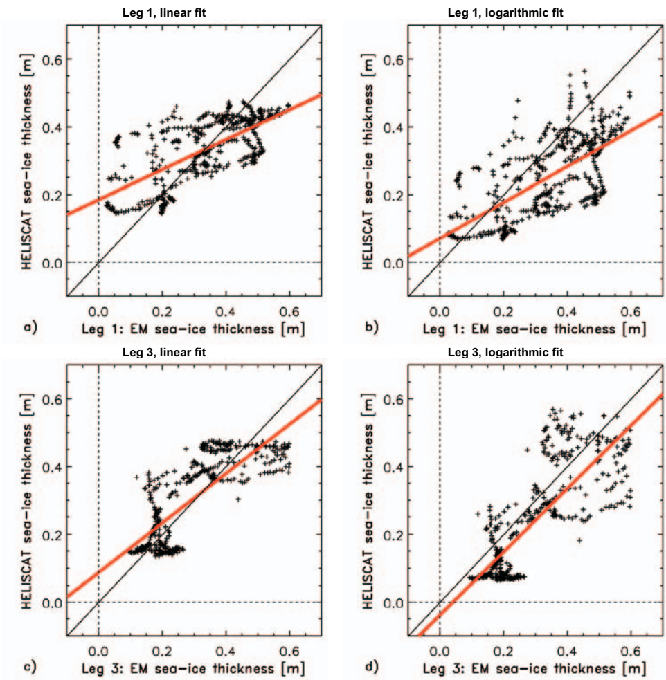
Figure 4. HELISCAT derived vs. EM-Bird observed ice thickness for leg 1 (top) and leg 3 (bottom) using an averaging window of 150m and a SNR > 20 dB; the used fits are derived from data of leg 1. Panel a) shows the thickness for leg 1 using the linear fit, b) is for leg 1 using the logarithmic fit, c) and d) are for the independent data of leg 3 using the linear and the logarithmic fit, respectively. Red lines denote the linear regression between each of the shown thickness data sets. Thin black diagonals denote perfect agreement.
