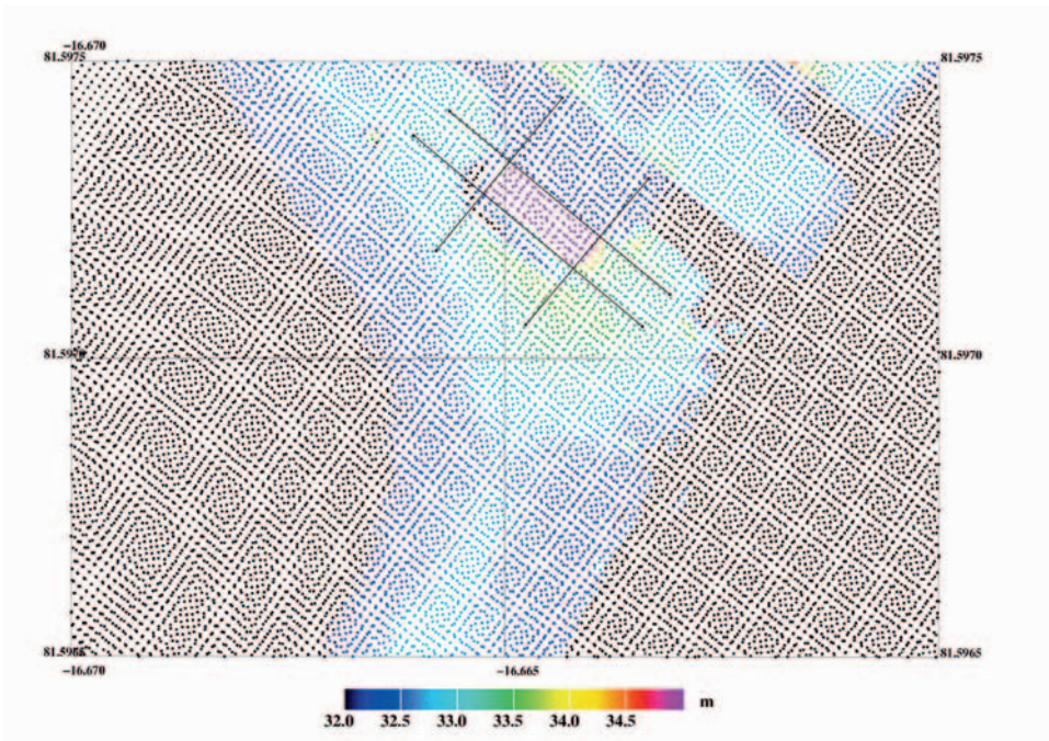
Figure 4. Lidar data from a calibration flight at Station Nord, May 2005.
