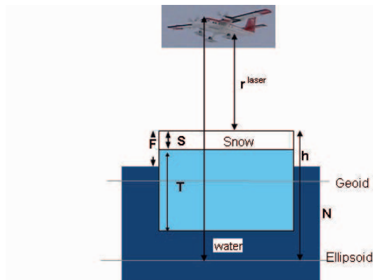
Figure 3. Illustration of the observation principle and principle of freeboard determination.
