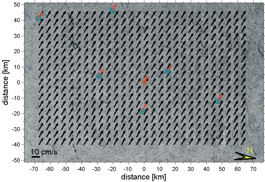
Figure 2. Standard motion products. The SAR scenes and buoy positions from Figure 1 are used to compute velocity vectors to a resolution of 4.8 km which is close to the smallest reasonable continuum scale. Buoy motion vectors (red) are computed from the buoy positions at times corresponding to the SAR scenes for independent comparison of motion products.
