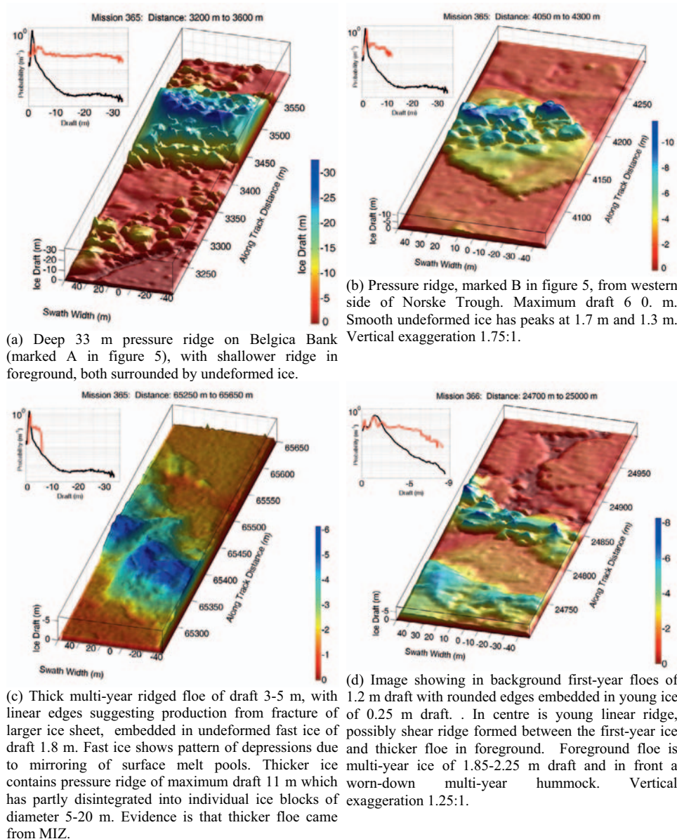
Figure 4. Some examples of EM-2000 multibeam ice draft data in perspective views, as if illuminated by a sun of elevation 20°. Data points fill 2 m x 2 m grid. No vertical exaggeration unless otherwise stated. Each image is accompanied by a probability density function (pdf) of ice draft (red) compared to the pdf of the mission as a whole (black), lin-log scale, 5 cm bins (Wadhams et al., 2006).
