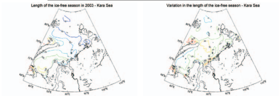
Figure 32. Current length of the ice-free season (left) and its variation between 1979 and 2003 (right) in the Kara Sea.
