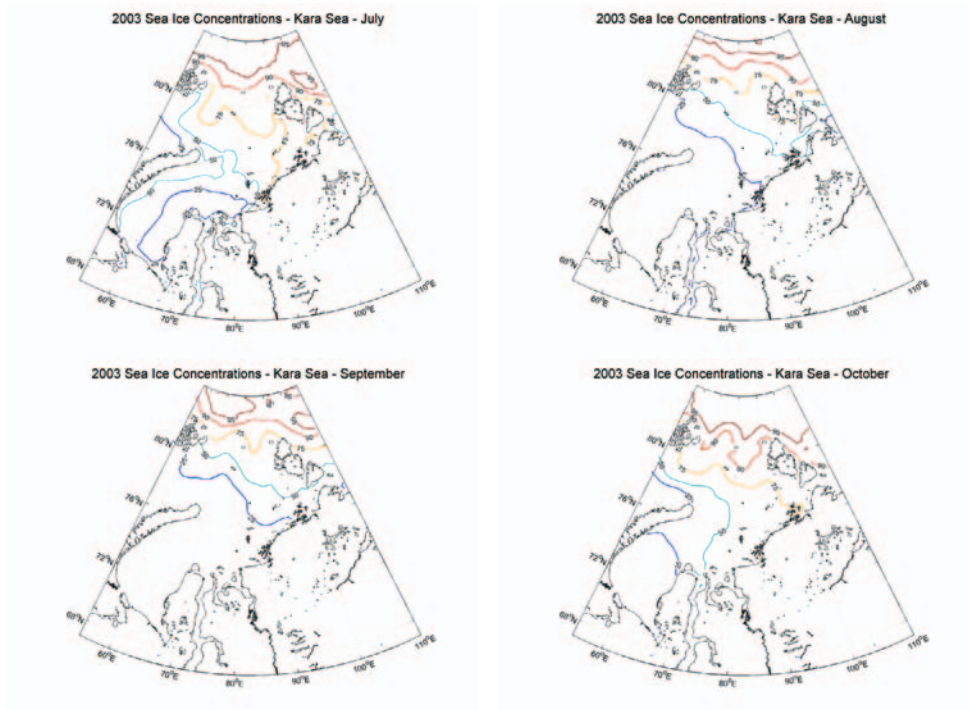
Figure 18. Current distribution of the sea ice concentrations in the Kara Sea.
