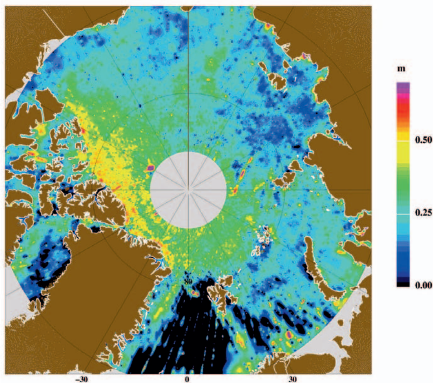
Figure 8. Sea-ice freeboard heights for February/March 2003 from ICESat. Unit m.
