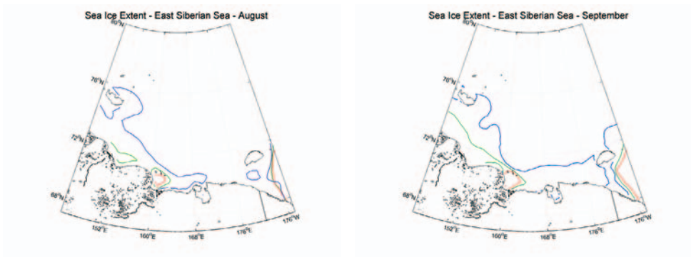
Figure 9. Changes in the sea ice edge in the East Siberian Sea.
