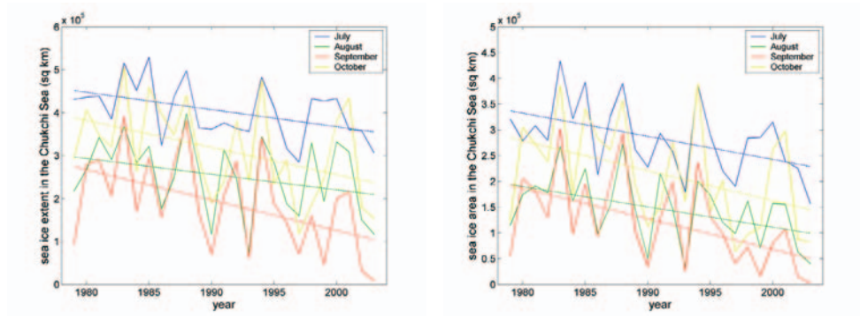
Figure 10. Sea ice extent (left) and sea ice area (right) in the Chukchi Sea during the 1979-2003 period.
