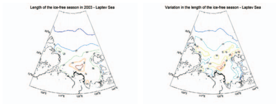
Figure 33. Current length of the ice-free season (left) and its variation between 1979 and 2003 (right) in the Laptev Sea.
