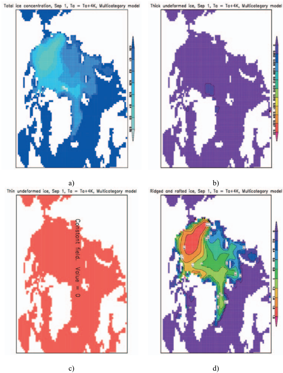
Figure 6. Sea ice response to air temperature change with the multi-category sea ice model, a) total ice concentration b) thick undeformed ice thickness c) thin undeformed ice thickness and d) deformed ice thickness on September 1.
