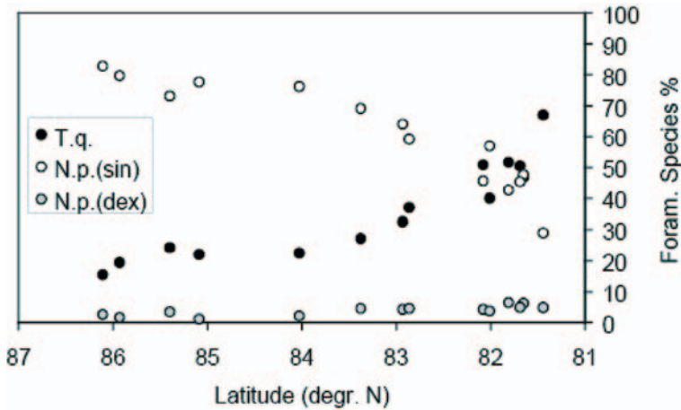
Figure 8. Recent distribution of planktic foraminifera (species >63\mu\text{m} ) in the upper 500 m water column of the Nansen Basin along a S-N transect from the northern Barents Sea margin ( 81^\circ\text{N} ) to the Gakkel Ridge ( 86^\circ\text{N} ). Subpolar species T. quinqueloba are found abundantly in the southern region characterised by strong advection of Atlantic Water. Data from Carstens and Wefer (1992).
