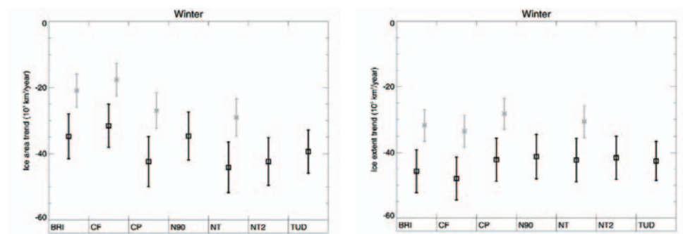
Figure 3. Observed trends in a) ice area and b) ice extent during winter (Oct. – Apr.) for the SSM/I dataset excluding the F8 satellite (1991-2004, black) and the entire dataset (1987-2004, grey). The 85GHz channels were not reliable on F8. Bars show \pm 1 STDEV.
