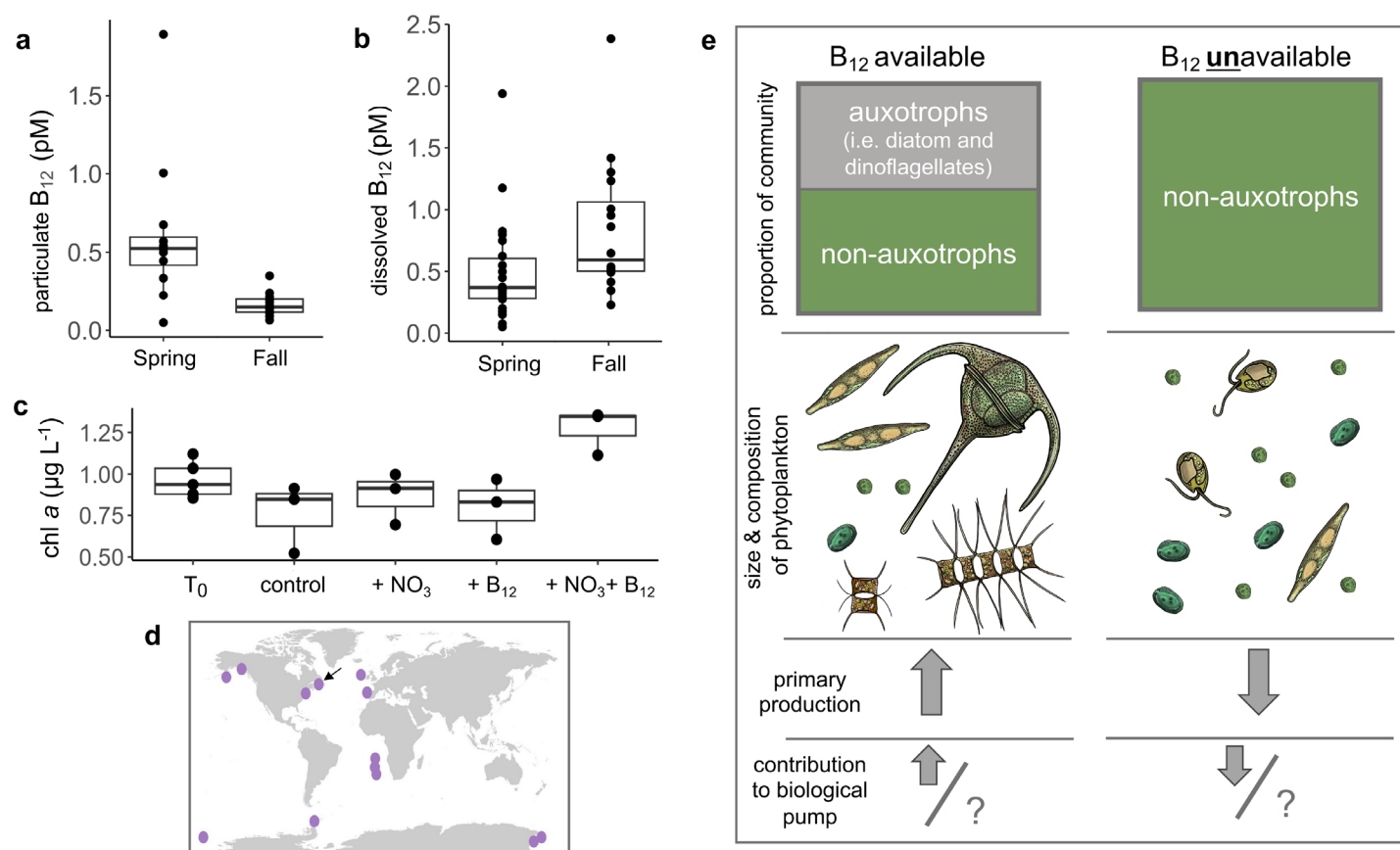
Fig. 3. Vitamin B 12 is a keystone metabolite in the surface ocean. B 12 is found in low pM concentrations in both cells and seawater, but sometimes enriched in particulate phase. Average (a) particulate ( n = 28 ) and (b) dissolved ( n = 33 ) concentrations (pM) of (a) total B 12 (Ado-, Me-, OH- and CN-combined) and (b) OH-B 12 (adjusted for percent recovery) at a coastal station in the Northwest Atlantic Ocean during Spring and Fall from 2016 to 2020. Data replotted from Bannon et al. 2024 with author permission. (c) B 12 and nitrogen added together stimulate chlorophyll a production in a microbial community from the coastal Northwest Atlantic Ocean during Spring. Chl a concentrations (µg L -1 ) measured initially (T 0 ) and 4 d after addition of +NO 3 (10 µM), +B 12 (100 pM) and +NO 3 + B 12 (10 µM, 100 pM; n = 3 ; Bannon et al. 2024). (d) B 12 co-limits phytoplankton growth in various regions. Global map of study sites where B 12 co-limitation was observed (modified from Bannon et al. 2022 under the terms of the Creative Commons Attribution License). Arrow highlighting sampling site of data shown in (a–c). (e) B 12 availability impacts microbial community structure and the biological carbon pump. Simplified illustration of conclusions from Gobler et al. 2007, Koch et al. 2011, and Bertrand et al. 2015. Note that the influence of B 12 on the biological carbon pump has not been systematically tested. This is inferred by evidence that B 12 availability selects for larger phytoplankton, which in turn have been shown to increase sinking rates and impact grazing rates. See Supporting Information Summary and Table S7a–d for details on compiled data. Figure illustrations by Rebecca S. Key.
