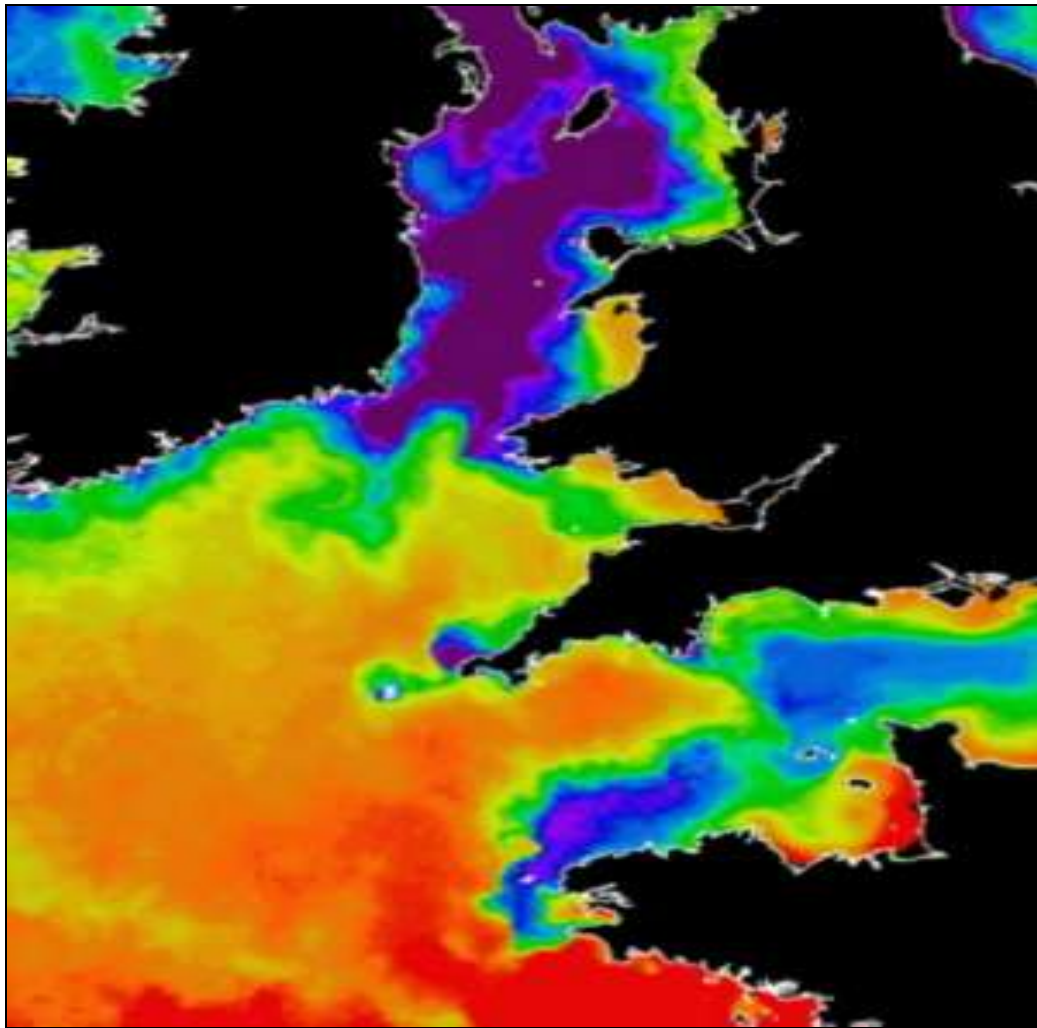
A typical summer sea surface temperature image of the Celtic and Irish Seas, from the Advanced Very High Resolution Radiometer satellite sensor (Image supplied by Remote Sensing Division, Plymouth Marine Laboratory, NERC)
