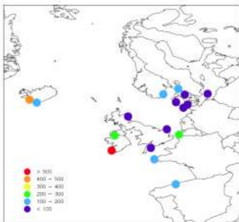
Figure 3.1: As depositions 2007, \mu\text{g}/\text{m}^2 p.a.
