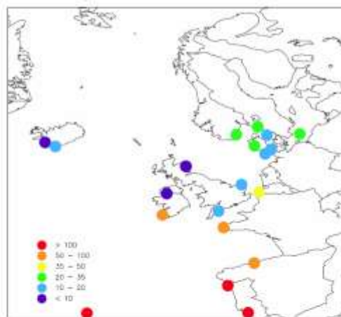
Figure 3.2: Cd depositions 2007, \mu\text{g}/\text{m}^2 p.a.
