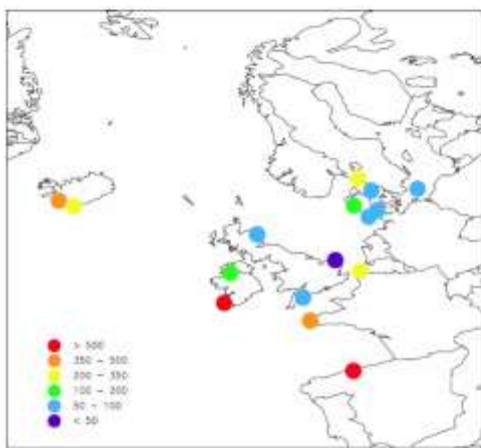
Figure 3.3: Cr depositions 2007, \mu\text{g}/\text{m}^2 p.a.
