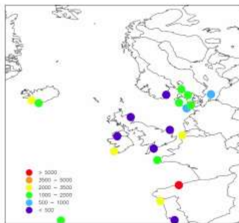
Figure 3.4: Cu depositions 2007, \mu\text{g}/\text{m}^2 p.a.
