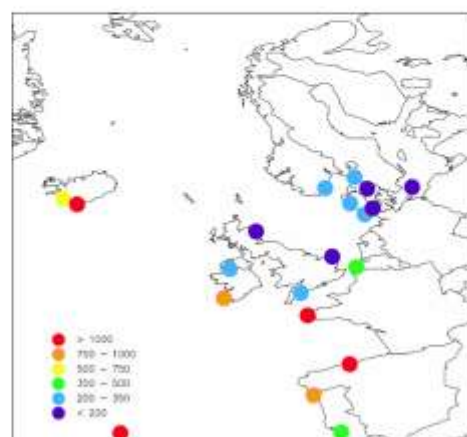
Figure 3.6: Ni depositions 2007, \mu\text{g}/\text{m}^2 p.a.
