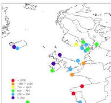
Figure 3.5: Pb depositions 2007, \mu\text{g}/\text{m}^2 p.a.
