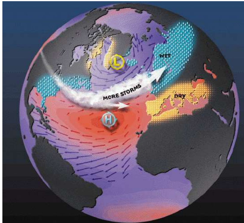
Positive NAO Index
