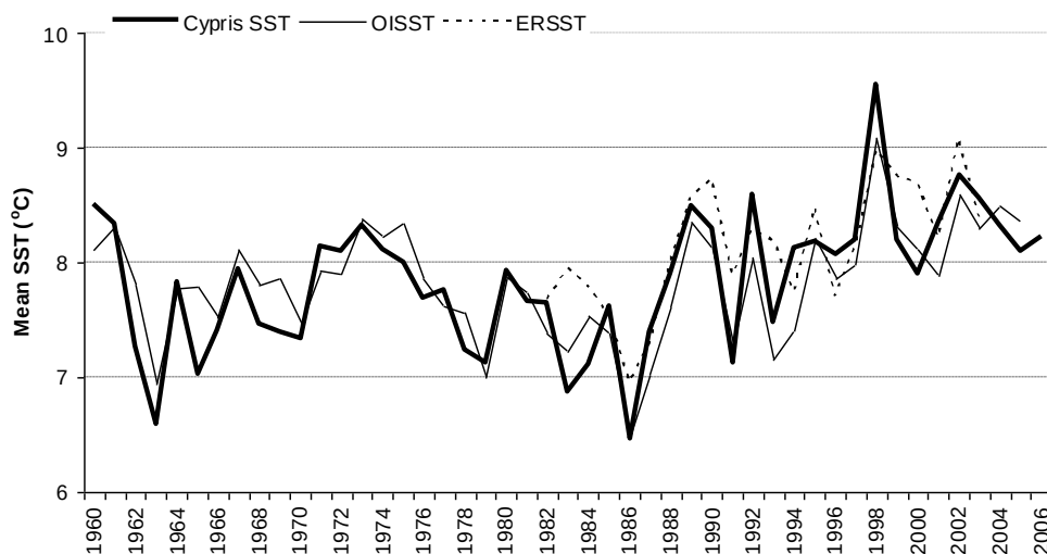
Sea surface temperature in the Irish Sea (1960 – 2006)
