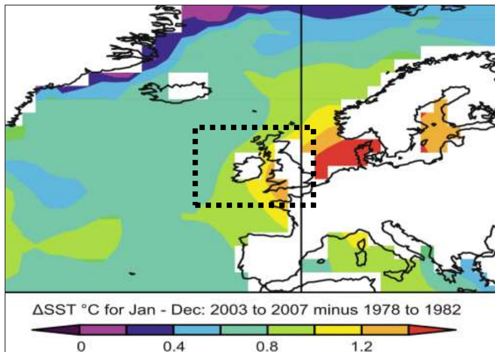
Sea surface temperature (SST), showing the mean for 2003–2007 minus the 1978–1982 mean (Source: ICES 2007). Note the increases in the NWW area, the boundary of which is shown by a dashed line
