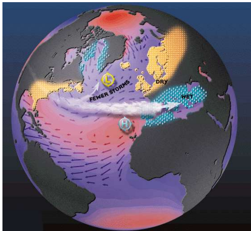
Negative NAO Index
