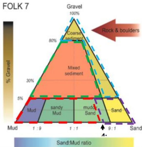
Figure 1. Left inset) BGS Modified Folk classification (Folk15) (Fig. 9); Right inset) Simplified Folk7 classification as well as modified sediment Sand:Mud ratio (i.e. 4:1) applied within the Hybrid class (Table 1). Modified from Kaskela et al., 2019. Only the Folk15 classification (+ rock) map is released here as a digital product (Fig. 9). The Hybrid classification map is shown for illustration purposes only (Fig.10).
