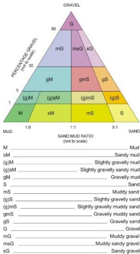
Figure 1. Left inset) BGS Modified Folk classification (Folk15) (Fig. 9); Right inset) Simplified Folk7 classification as well as modified sediment Sand:Mud ratio (i.e. 4:1) applied within the Hybrid class (Table 1). Modified from Kaskela et al., 2019. Only the Folk15 classification (+ rock) map is released here as a digital product (Fig. 9). The Hybrid classification map is shown for illustration purposes only (Fig.10).
