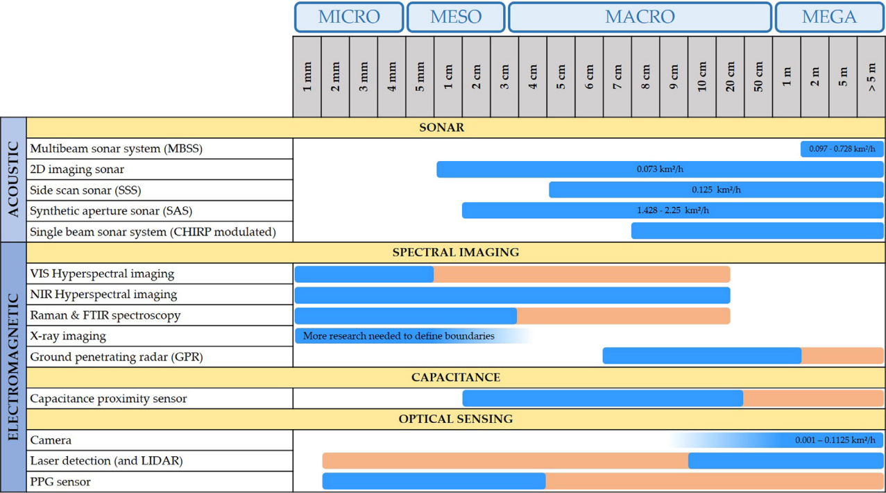
Fig. 4. Detection size range and spatial coverage (in km²/h) by seafloor detection technique. Blue bars show the detection range reported in literature to date. Orange bars show the possible extension of size range based on expert judgement of the co-authors.
