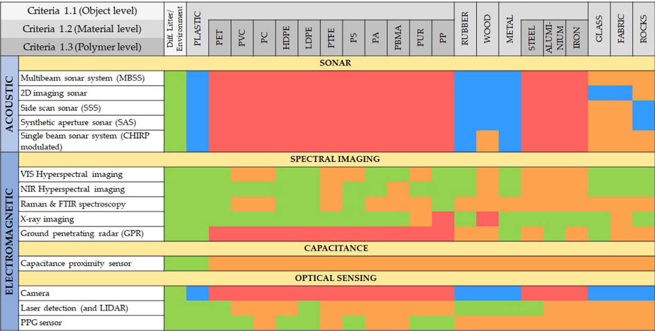
Fig. 3. Material differentiation capacity for each seafloor detection technique. (Green: positive differentiation, Blue: differentiation only based on the shape of target, Orange: not tested, Red: no differentiation).
