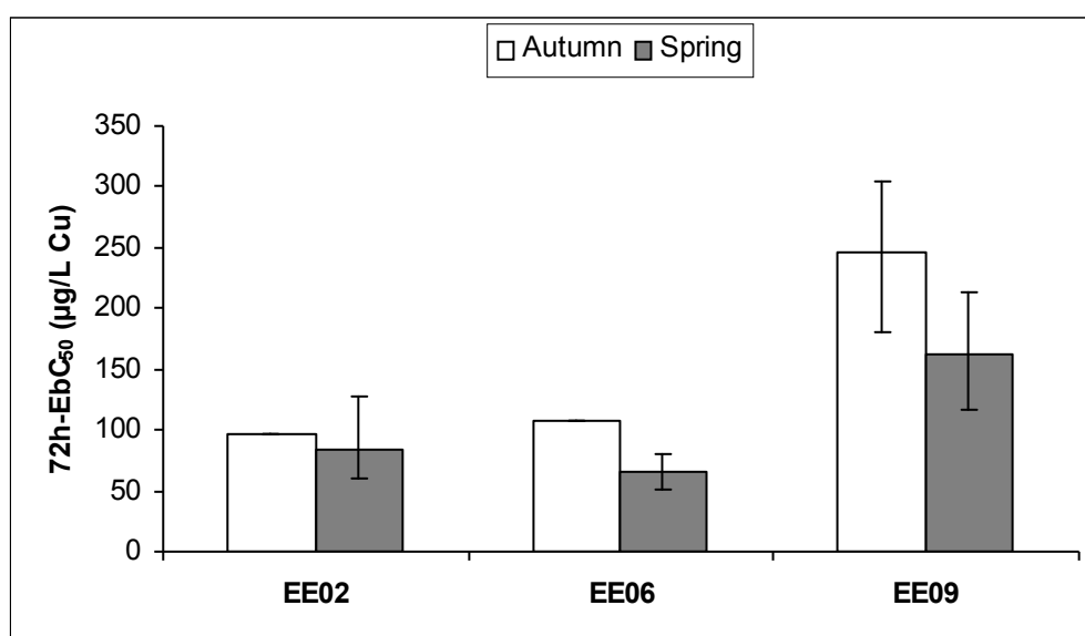
Figure 10: Seasonal differences on observed 72h-EbC 50 for R. subcapitata in 3 surface waters.
