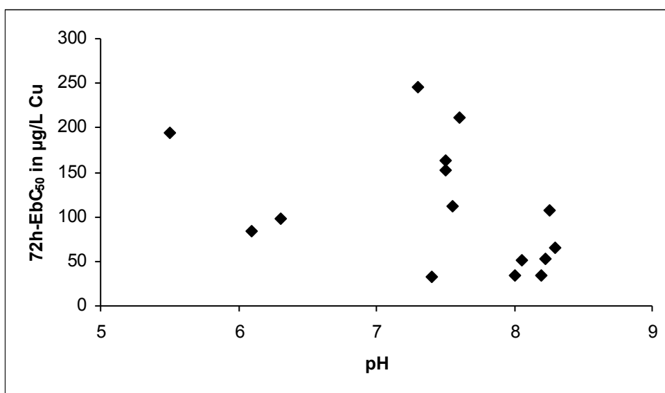
Figure 14: Copper toxicity to the alga R. subcapitata as a function of the pH of the surface water during the test period.
