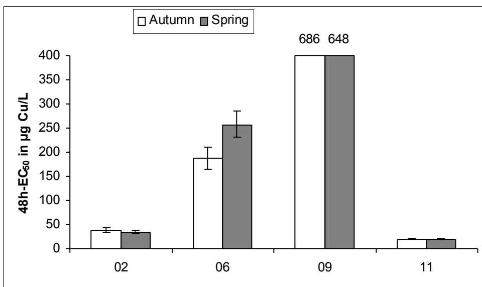
Figure 3: Seasonal differences on observed 48h-EC 50 for D. magna in 4 surface waters.
