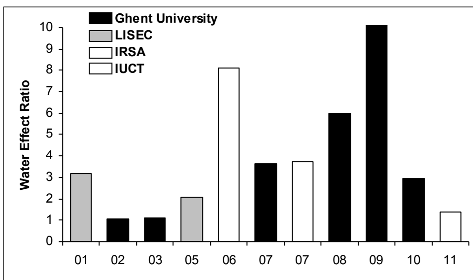
Figure 2: Water Effect Ratio for D. magna (acute) in 10 surface waters spiked with CuSO 4 .
