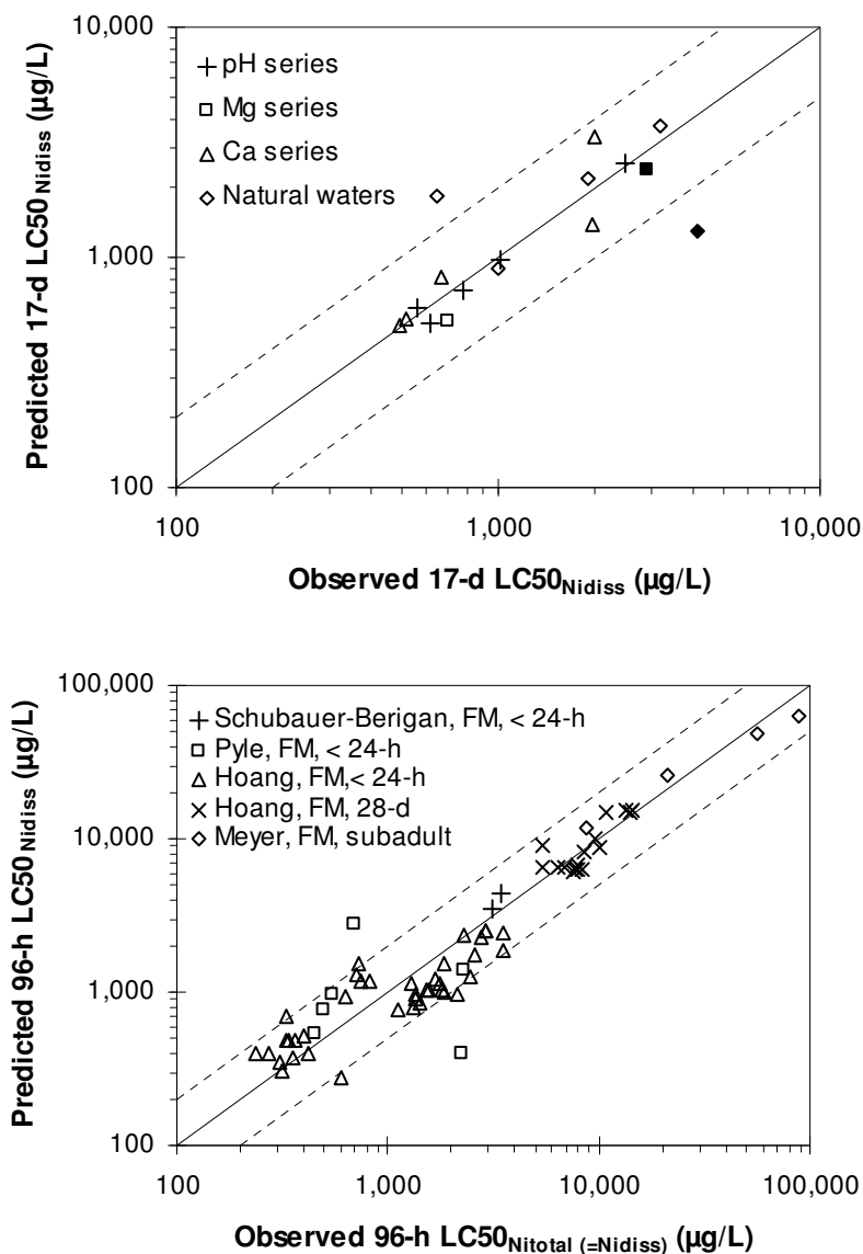
Figure 2.4. Predicted \text{LC50}_{\text{Nidiss}} versus observed \text{LC50}_{\text{Nidiss}} ( \mu\text{g/L} ). 96-h \text{LC50} s (lower panel) were reported in literature as total nickel concentrations but were assumed to be similar based on dissolved nickel concentrations (as mentioned by Hoang et al., 2004). Predictions were made using optimized model parameters (Table 2.4) and Equation 2.3 linked to WHAM VI. The solid line indicates a perfect match between predicted and observed \text{LC50} s; the dashed lines indicate ratios of 0.5 and 2 between observed and predicted \text{LC50} s. Upper panel: 17-d \text{LC50} s for rainbow trout (present study). Filled symbols represent extrapolated 17-d \text{LC50} s (Table 2.3). Lower panel: 96-h \text{LC50} s for fathead minnow (FM) taken from several studies (Schubauer-Berigan et al., 1993; Meyer et al., 1999; Pyle et al., 2002a; Hoang et al., 2004).
