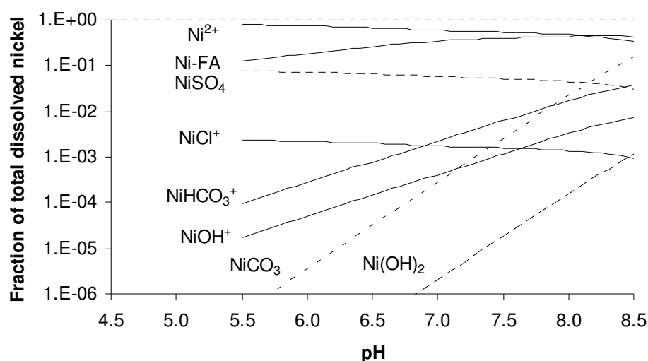
Figure 1.3. Nickel species distribution as a function of pH. Composition of medium = 0.75 mM Ca, 0.25 mM Mg, 1.5-3.0 mM Na (varied to maintain charge balance), 0.05 mM K, 1.0 mM SO 4 2- , 1.55 mM Cl - , 2.0 μM Ni and 5 mg DOC/L. Dissolved inorganic carbon (DIC) concentrations were estimated assuming an open system in equilibrium with the atmosphere using thermodynamic stability constants taken from Stumm and Morgan (1996). Nickel speciation was simulated at a temperature of 20 °C using WHAM VI software (NERC, 2001). Stability constants for inorganic complexes were taken from Smith et al. (2004). Model parameters describing the interactions between nickel and fulvic acid (FA) were optimized as described in chapter 2.
