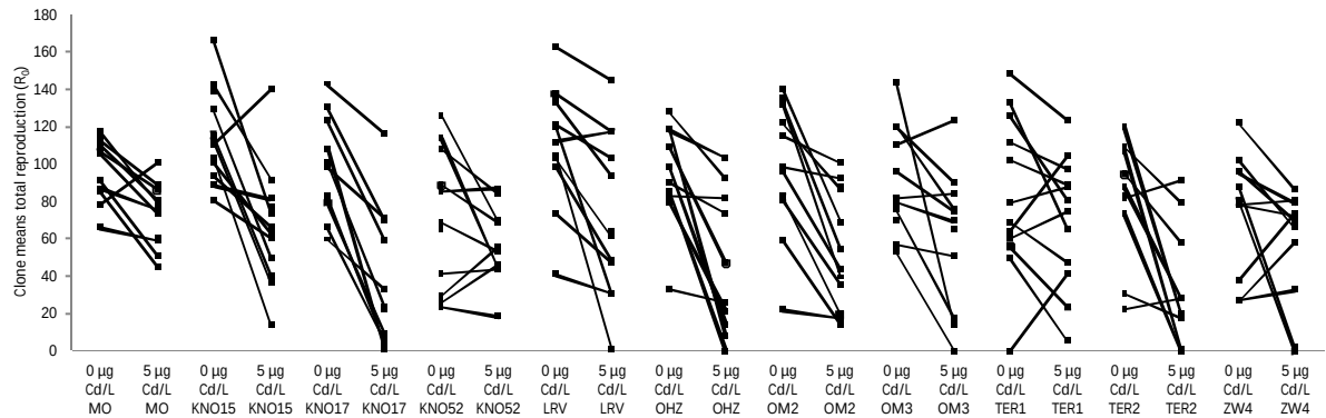
Figure S5.1: Clone means of total reproduction ( R_0 ) for different populations in control and Cd treatment.
