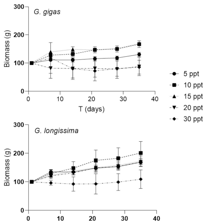
Fig. 3. Growth ( \pm SD) over time of both species per salinity.
