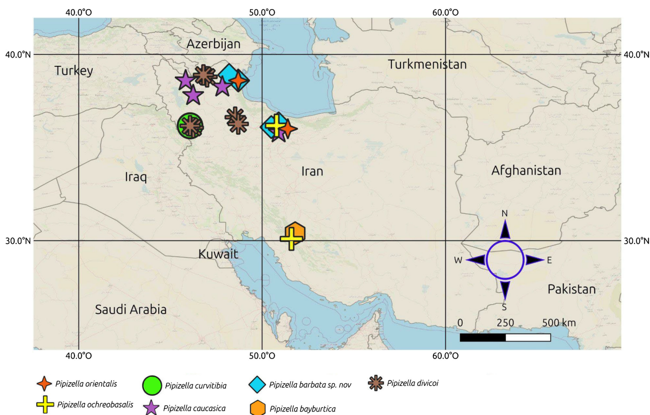
Figure 34. Distribution of Pipizella barbata Mortelmans & van Steenis sp. nov. and the other Pipizella species recorded in Iran and Azerbaijan.
