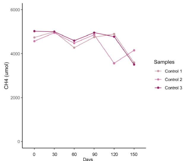
Figure 5.6. Headspace measurements for methane over 150-days for enrichments from controls used for each depth. Controls do not drop below 3500 \mu\text{mol} methane.
