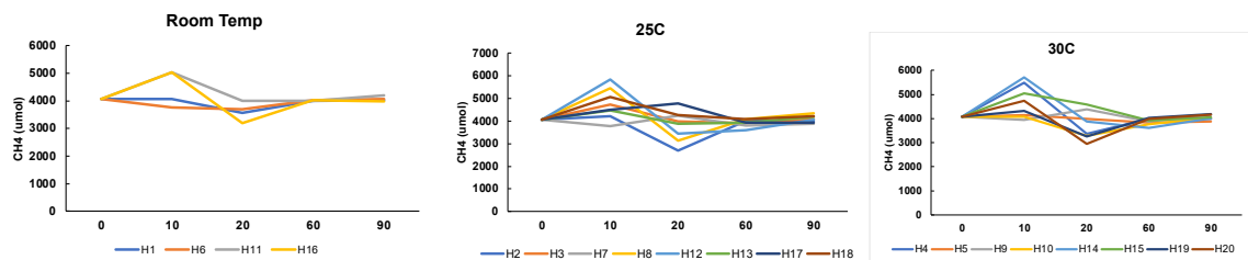
Figure E8. Headspace measurements for methane (µmol) over 90-days for enrichments from Transfer 1 at 21 C (Room Temperature), 25 C and 30 C.
