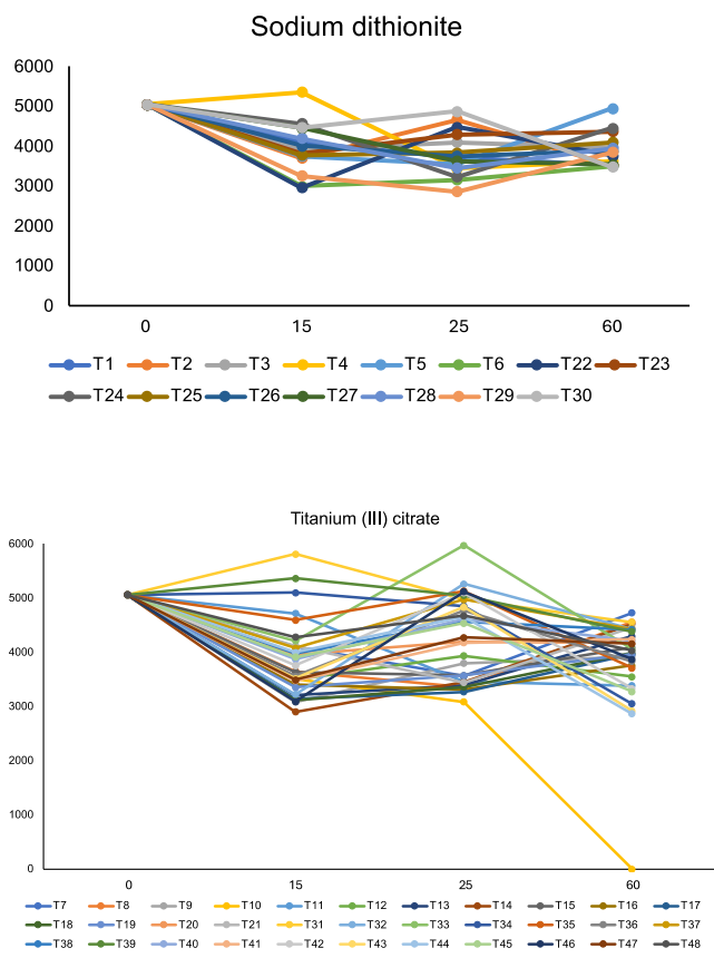
Figure E2. Headspace measurements for methane ( \mu\text{mol} ) over 60-days for enrichments from Transfer 1 using titanium (III) citrate and sodium dithionite.
