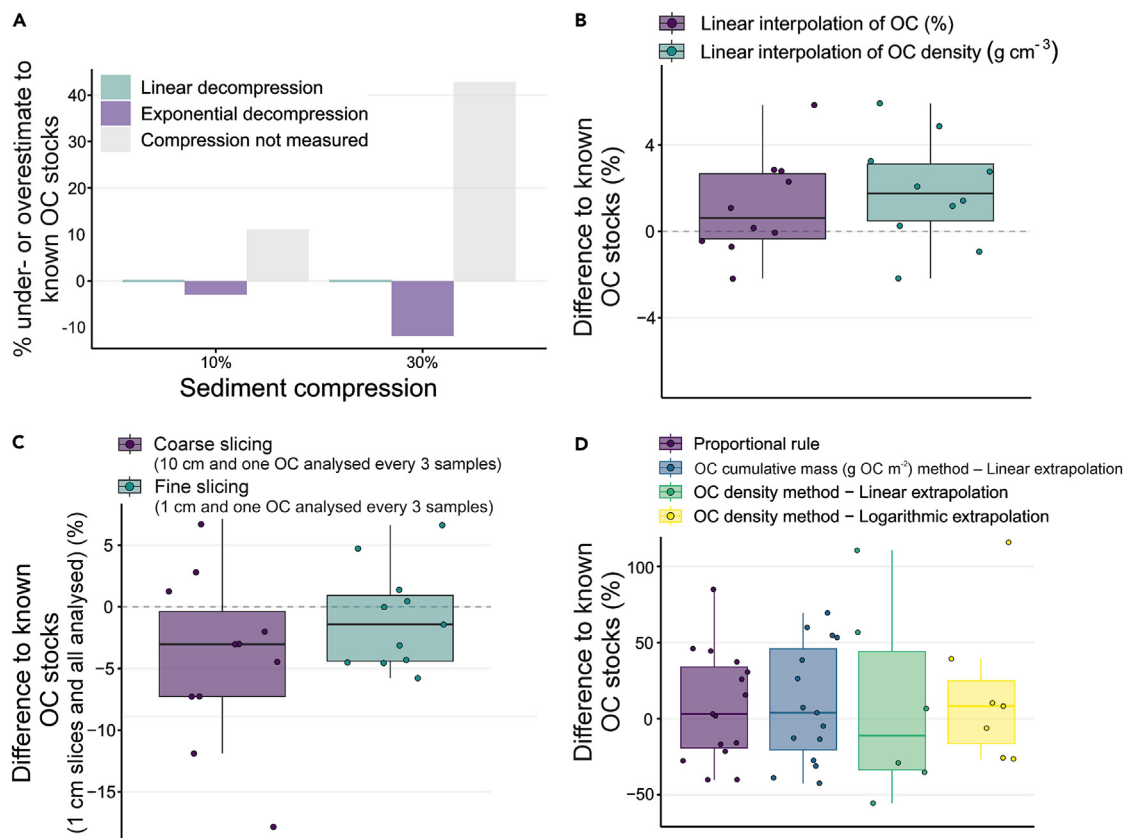
Figure 3. Methodological issues related to soil coring and slicing, and the interpolation and extrapolation of organic carbon (OC) stocks
