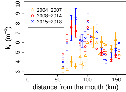
(b) Time-averaged light-extinction coefficient in spring
