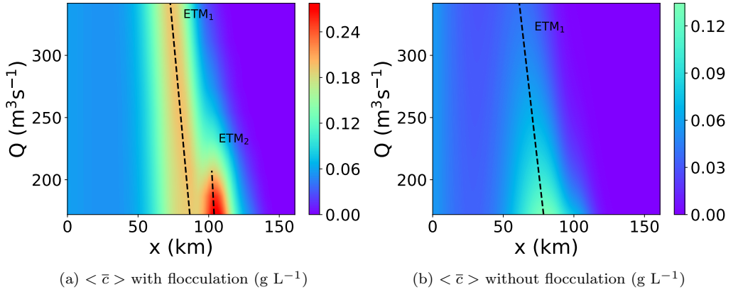
Figure 2.8: Depth-averaged subtidal suspended sediment concentration \langle \bar{c} \rangle (g L -1 ) for varying freshwater discharge Q ( M = 0.00336 s m -1 ). The black dashed lines depict the locations of the ETM. (a) Result with flocculation ( k_B = 5600 s 1/2 m -2 ). (b) Result without flocculation ( w_s^0 = 3 mm s -1 ).
