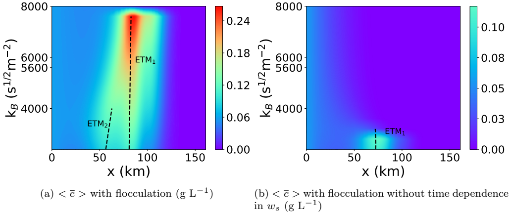
Figure 2.7: Depth-averaged subtidal suspended sediment concentration \langle \bar{c} \rangle (g L -1 ) for varying floc break-up parameter k_B ( Q = 233 \text{ m}^3 \text{ s}^{-1} and M = 0.00336 \text{ s m}^{-1} ) in the case with flocculation. The black dashed lines depict the locations of the ETM. (a) Result with time dependence in w_s . (b) Result in which we excluded the time dependence in w_s .
