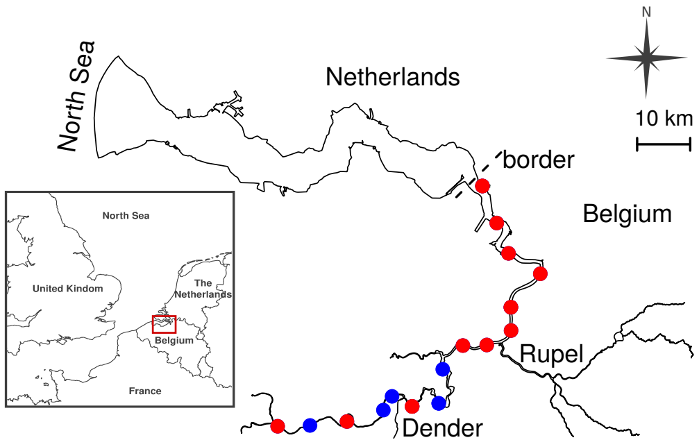
Figure 3.1: The Scheldt estuary and its two main tributaries (Rupel and Dender). The dots represent the locations where monthly and biweekly turbidity and floc size profiles were measured in the frame of the OMES (Dutch: “Onderzoek Milieu Effecten Sigma-plan”) environmental monitoring program. The transparent exopolymer particles (TEP) concentration was only measured at 11 instead of the 16 stations, depicted in red.
