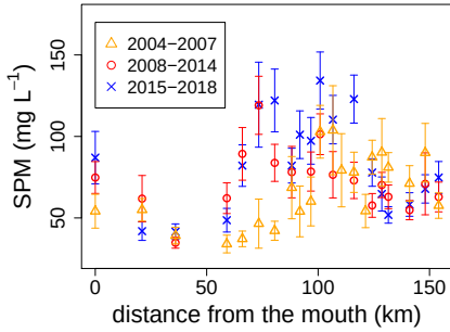
(a) Time-averaged SPM concentration in spring
