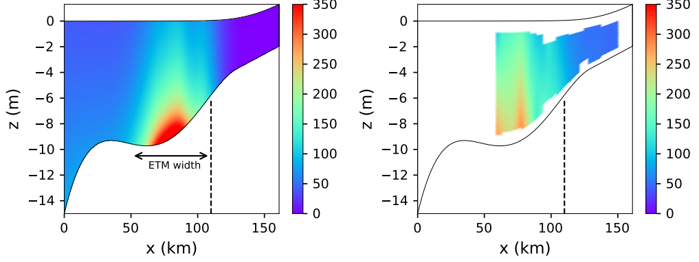
(a) Suspended sediment concentration with flocculation (mg L -1 ) (b) OMES dataset of suspended sediment concentration (mg L -1 )
