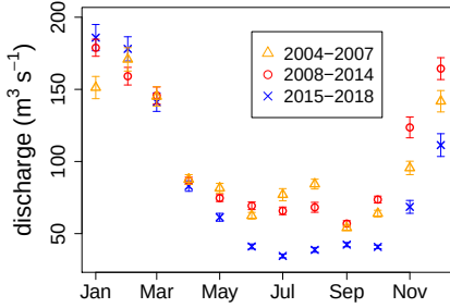
(a) Time-averaged discharge
