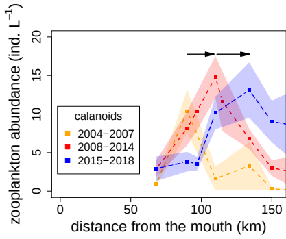
(a) Calanoid abundance in spring
