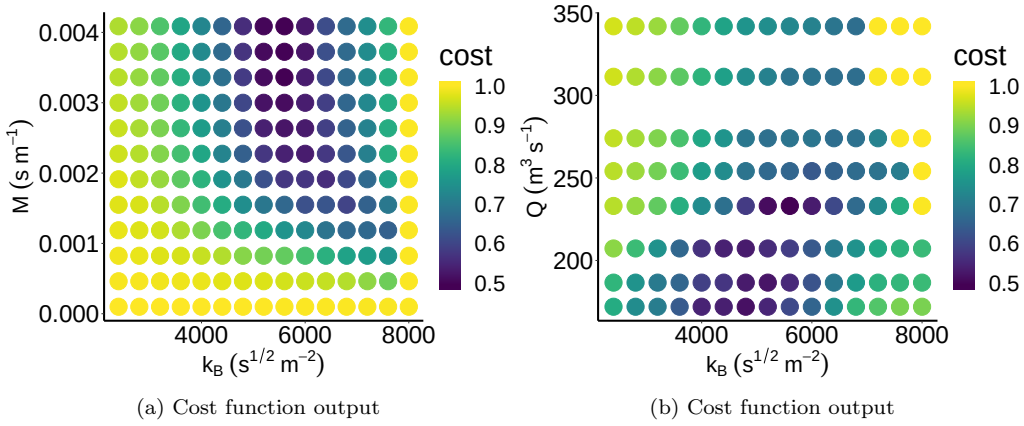
Figure 2.4: Cost function values for (a) various erosion parameter M and floc break-up parameter k_B ( Q = 233 \text{ m}^3 \text{ s}^{-1} ) and (b) various total river discharge Q and floc break-up parameter k_B ( M = 0.00336 \text{ s m}^{-1} ). The optimal calibration parameter set corresponds to k_B = 5600 \text{ s}^{1/2} \text{ m}^{-2} , M = 0.00336 \text{ s m}^{-1} , and Q = 233 \text{ m}^3 \text{ s}^{-1}
