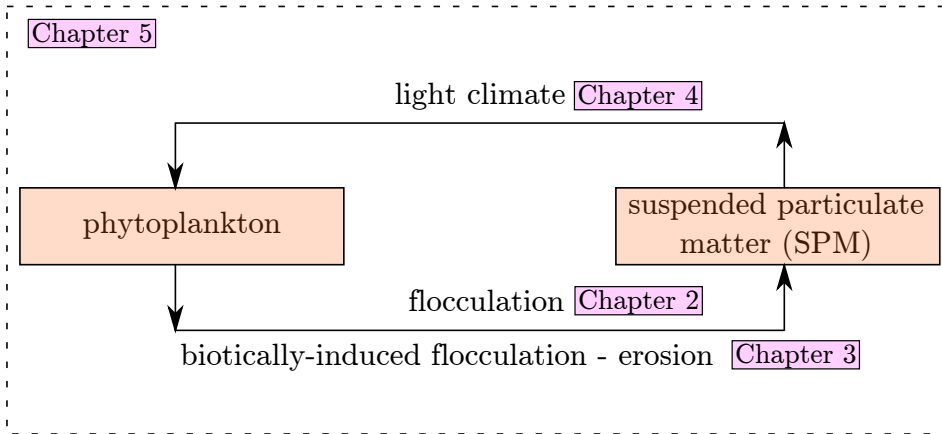
Figure 1.3: Illustration of the interconnection between SPM and phytoplankton studied in this thesis and corresponding chapters. SPM limits phytoplankton growth by deteriorating the light climate in the water column. Phytoplankton may affect SPM dynamics by altering the floc size and structure of flocs and excreting sticky substances that stimulate flocculation of SPM. In Chapter 2, we study the impact of flocculation on SPM. In Chapter 3, we focus on the importance of biotically-induced flocculation on SPM. In Chapter 4, we study the impact of temporal variability in light climate (cf. SPM) on phytoplankton. We combine all results and study a specific case regarding phytoplankton-SPM dynamics in the Scheldt estuary in Chapter 5.
