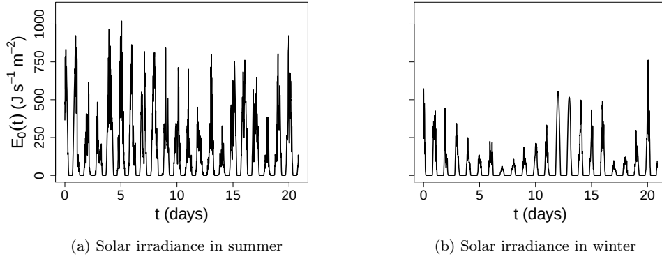
Figure 4.3: Solar irradiance E_0 measured at Stabroek (Belgium) in (a) summer and (b) winter. Stabroek is located approximately 25 km from the monitoring station at Kruibeke.
