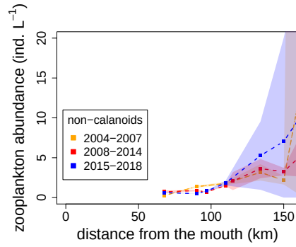
(b) Non-calanoid abundance in spring
