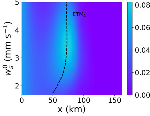
Figure 2.9: Depth-averaged subtidal suspended sediment concentration \langle \bar{c} \rangle (g L -1 ) for varying constant settling velocity w_s^0 ( Q = 233 m 3 s -1 and M = 0.00336 s m -1 ) in the case without flocculation. The black dashed line depicts the locations of the ETM.
