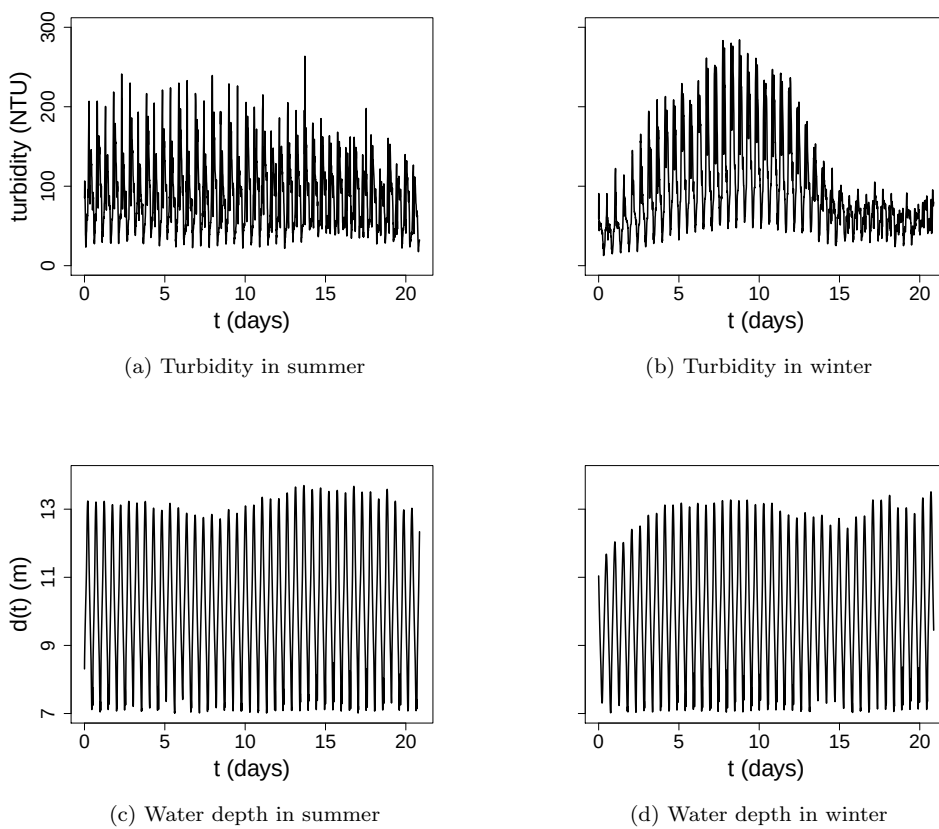
Figure 4.2: (a)-(b) Turbidity and (c)-(d) water depth measured in the Scheldt estuary at Kruike station (Belgium) in summer and winter.
