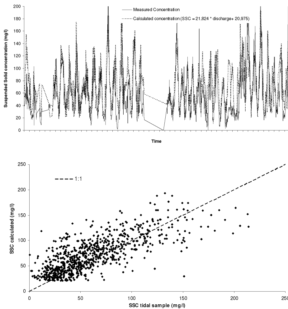
Figure 7. Relation between measured suspended solids concentration of longterm tidal sampling (mg/l) and calculated concentration out of inflow discharge (mg/l)
