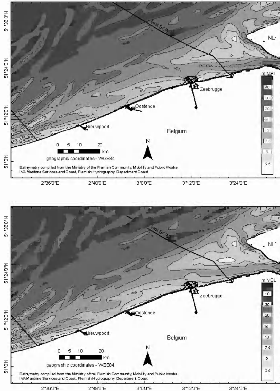
Figure 10: Bathymetry derived respectively from 2003 surveys (above) and from surveys before 1959 (below). Significant differences occur in the coastal zone and navigation channels.
