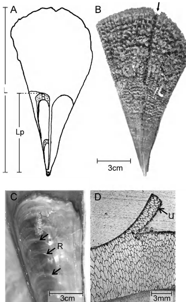
Fig. 2. P. nobilis . (A) Diagrammatic appearance of the inner shell surface to illustrate the position of a ring (R) on the internal posterior adductor muscle scar. L: shell length; Lp: length of the posterior adductor muscle scar. (B) Photograph of the external shell surface adorned with small spines. Arrow indicates the transect along which the pairs of spines were removed for analysis. (C) Photograph of the posterior adductor muscle scar showing several clear rings (R) (arrows). (D) Photomicrograph of a section through the outer shell layer and a spine (U) to show the prismatic shell structure is contiguous through both. Scale bars in B and C = 3 cm and in D = 3 mm.
