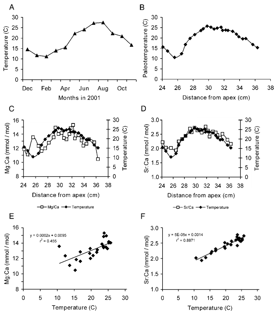
Fig. 3. (A) Seasonal variation (2000–2001) in sea surface temperature (SST) at Malo jezero, Croatia; (B–F) Data from P. nobilis from Malo jezero, Croatia. (B) Shell 1 from Malo jezero, inferred SST profile calculated from the stable oxygen-isotope composition in surface spines from a section of the outer surface; (C, D) comparison of Mg:Ca and Sr:Ca ratios, respectively, and inferred SST from surface spines from the same section of shell in B; (E, F) linear relationship between Mg:Ca and Sr:Ca ratios, respectively, and inferred SST.
