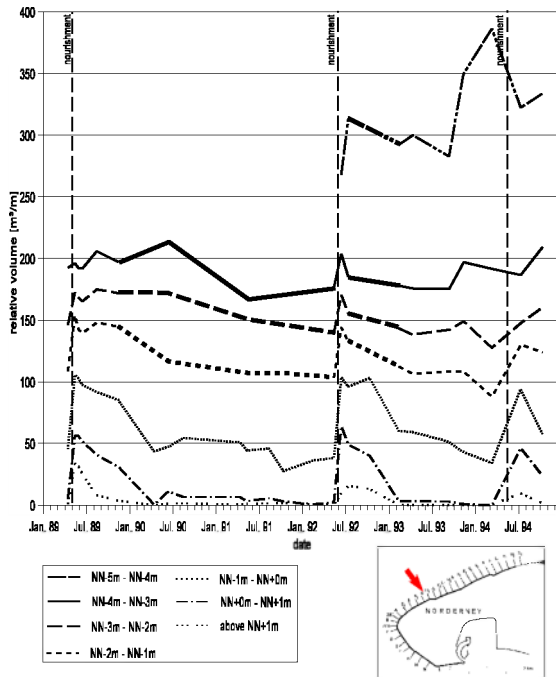
Fig. 9: Relative volumes per m beach length between the groyne G_1 and H_1 between distinct levels after the conventional beach replenishment in 1989 and the combined beach and shoreface nourishment in 1992
