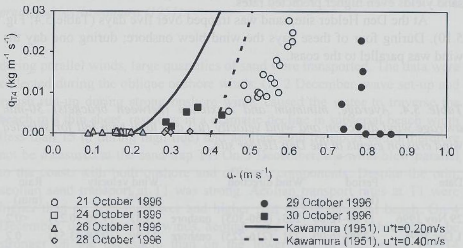
Figure 5.9. Aeolian sand transport at sand trap T4 ( q_{T4} ) versus friction velocity ( u_* ) at the Ameland site. The lines represent the transport rate predicted by Kawamura (1951).
