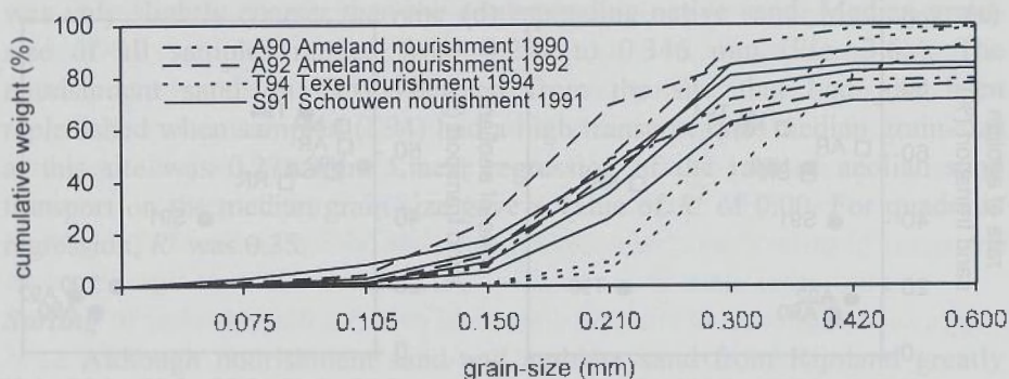
Figure 3.5. Cumulative curves of grain-sizes, showing variation in grain-size distribution within some nourished sites.
