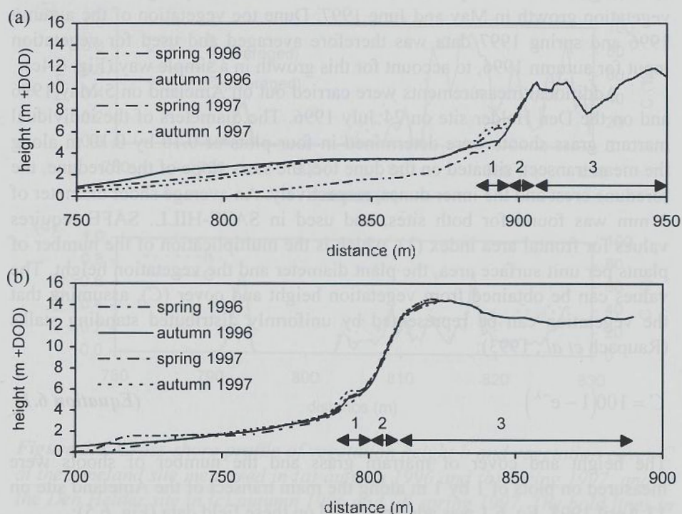
Figure 6.3. Measured topographical development for (a) Ameland and (b) Den Helder. The numbers refer to geomorphological zones, i.e. (1) dune toe, (2) stoss slope of the foredune and (3) foredune crest.
