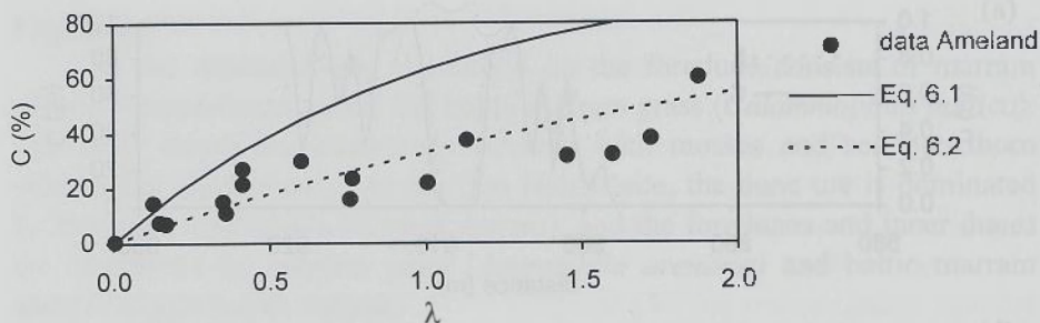
Figure 6.5. Frontal area index \lambda versus vegetation cover C for the marram grass vegetation on the foredune of Ameland. The solid line represents the Raupach et al. (1993) equation. The dotted line represents the equation, based on field data of Ameland, which was used in this study.
