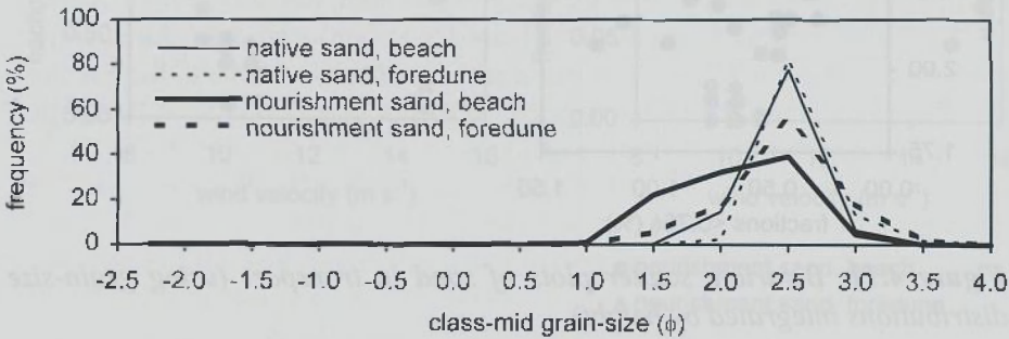
Figure 4.10. Examples of grain-size distributions of sand in transport, integrated by height.
