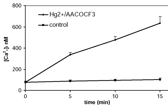
Fig. 3. Effect of AACOCF3 pre-incubation prior to Hg 2+ on [Ca 2+ ] i showing that the drug does not prevent the Ca 2+ rise induced by the metal. Data are means ± S.D. of 10 Ca 2+ measurements.
