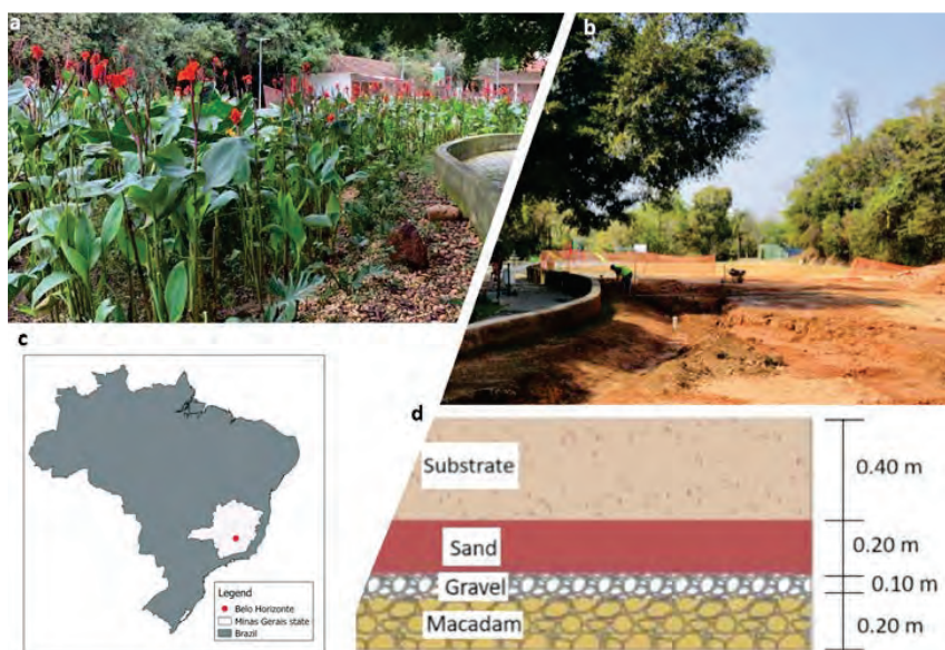
Figure 6.1 | Rain garden in the park Fazenda Lagoa do Nado (Belo Horizonte, Brazil) (a), construction phase (b), (c) location and (d) rain garden layers (figure adapted from Codas (2021)).
