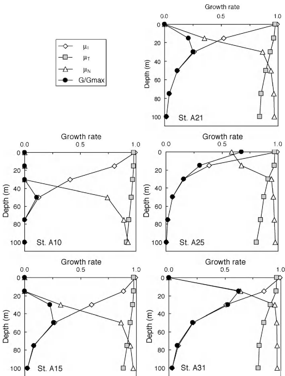
Fig. 10. Vertical profiles of estimated limiting factors and growth rates.
