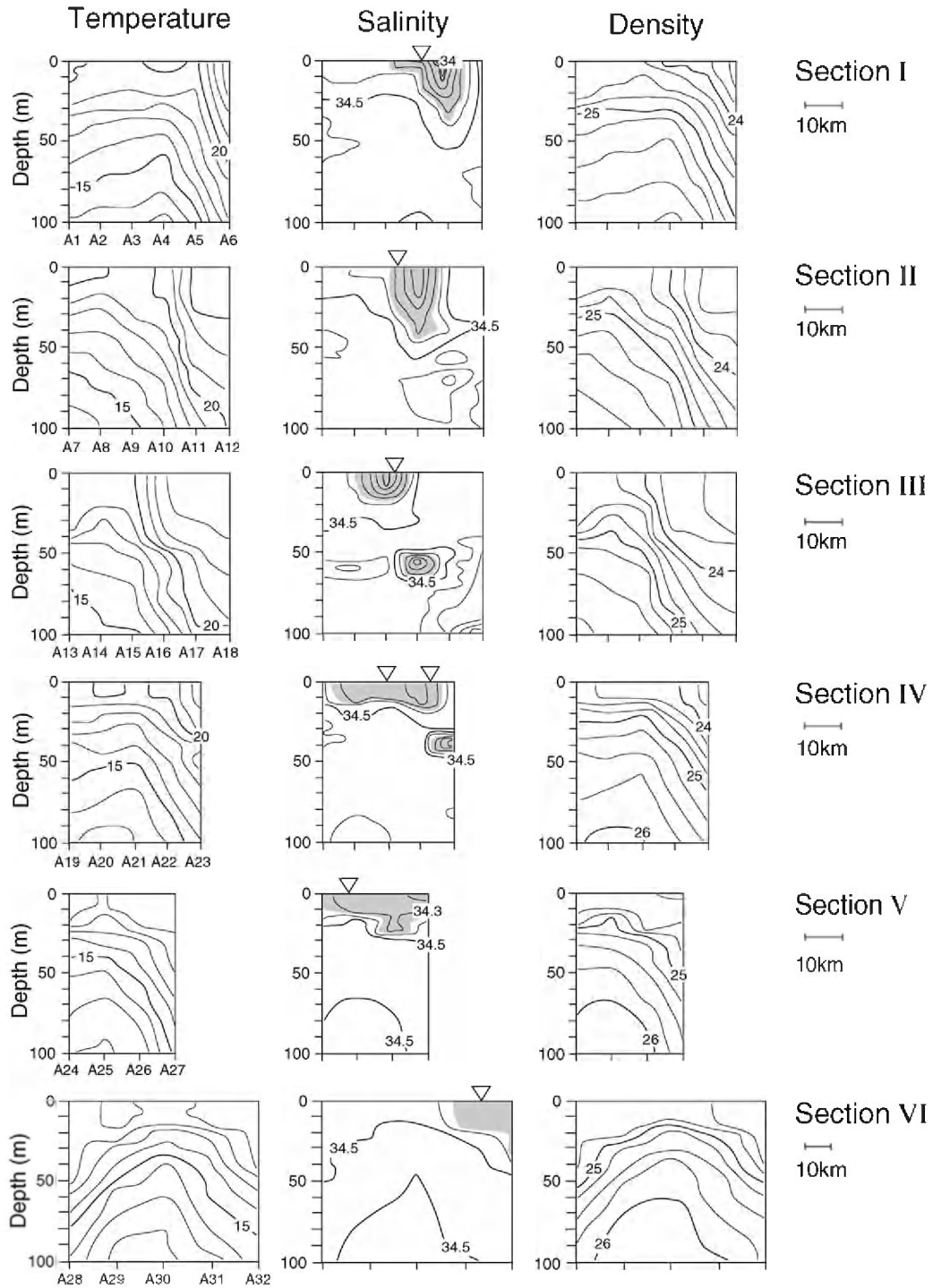
Fig. 4. Vertical distributions of temperature ( ^{\circ}\text{C} ), salinity (practical salinity units, psu) and density ( \sigma_t ) along the six sections. Shaded areas indicate the water with salinity lower than 34.35 psu. Triangles are positions of drifters.
