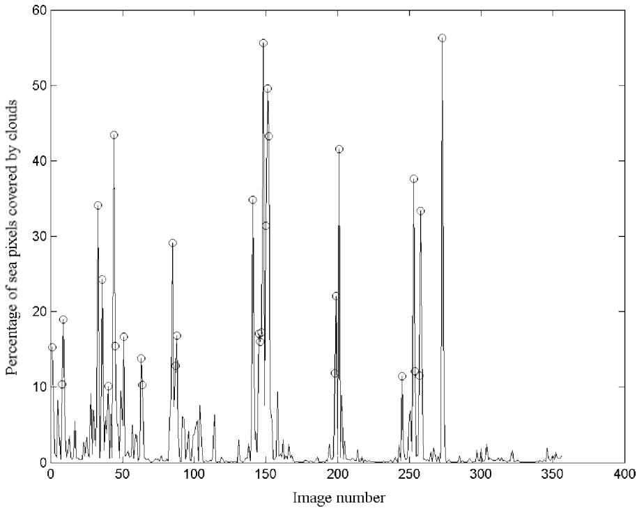
Fig. 2. Percentage of cloudy “sea” pixels versus image number. Circles mark those images with more than 10% of “sea” pixels covered by clouds.
