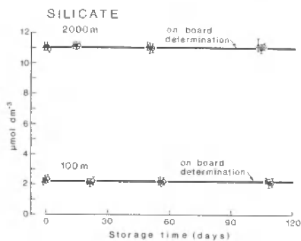
Fig. 3. Silicate concentration ( x \pm 1 st.dev.) in stored samples as a function of time. For symbols see legend to Fig. 1
