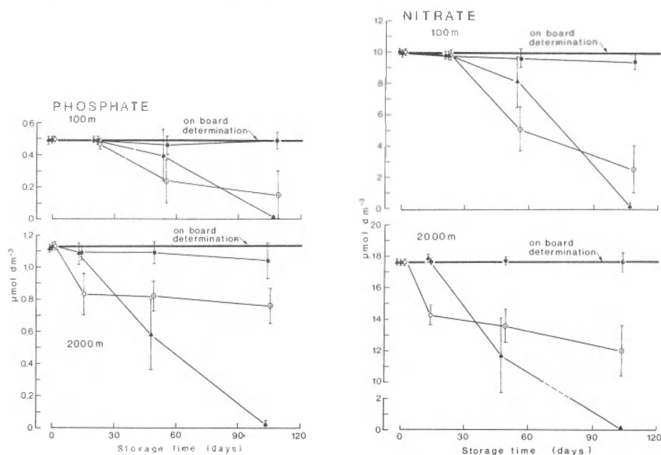
Fig. 1 (left). Phosphate concentration ( x \pm 1 st.dev.) in stored samples as a function of time. The indicated reference value is the average of approximately 150 on board determinations. The symbols refer to the samples stored at -18^\circ\text{C} ( \bullet-\bullet ); 4^\circ\text{C} ( \circ-\circ ); 4^\circ\text{C} and frozen after first time-interval ( \odot-\odot ); 4^\circ\text{C} with 10 \text{ mg dm}^{-3} \text{HgCl}_2 ( \blacktriangle-\blacktriangle ).
