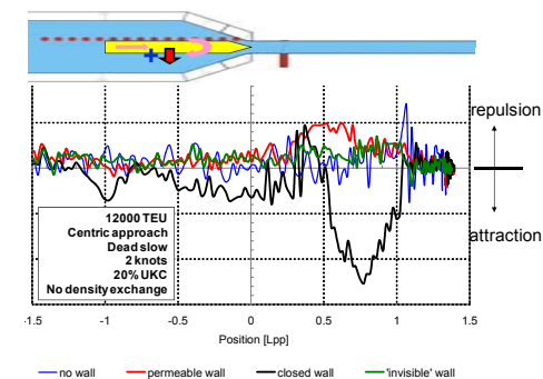
Figure 1. Lateral force on a self-propelled guided ship model during lock approach: effect of approach wall layout. Zero position is sketched above. Source: Flanders Hydraulics Research commissioned by Consorcio Pos Panamax on behalf of Panama Canal Authorities, [1], [2].
