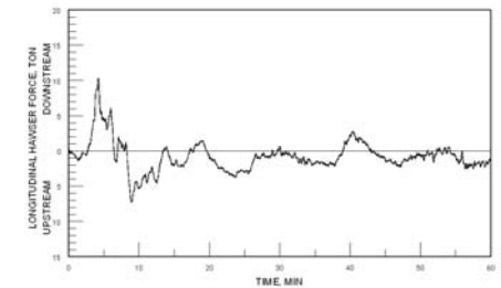
Fig 4: Hawser forces on a tow moored in the upper approach during lock filling
