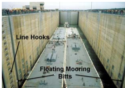
Fig 1: Tow mooring for lock filling
