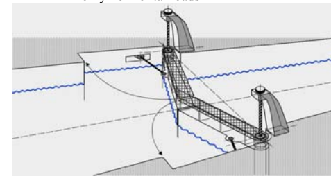
Fig. 3. Suspension miter gates with hinges bearing only horizontal loads
