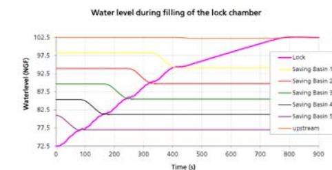
Fig 2: Levels during filling of lock
