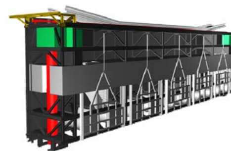
Fig. 3. Lay-out of Malamocco Lock gate in Venice, showing one hydro-foot tube in red.
