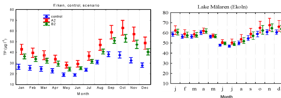
Figure VI.A.8. Mean, maximum and minimum values of predicted total phosphorus (TP) concentration (µg/l) in Lake Erken and in the Ekoln basin of Lake Mälaren for the three climate emission scenarios ( control 1960-1990; A2 - 2070-2100; B2, - 2070-2100 ).
