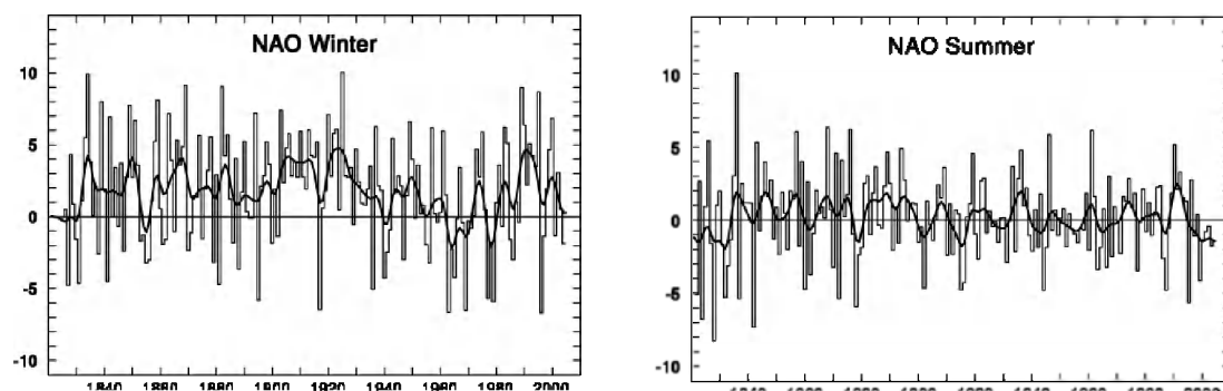
Figure IV.A.2 NAO - North Atlantic Oscillation
