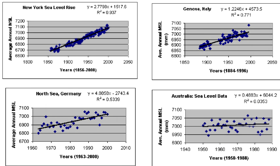
Figure IV.C.1. Average sea level rise (mean sea level MSL, in mm) from tidal gauges collected at different coastal locations around the world.
