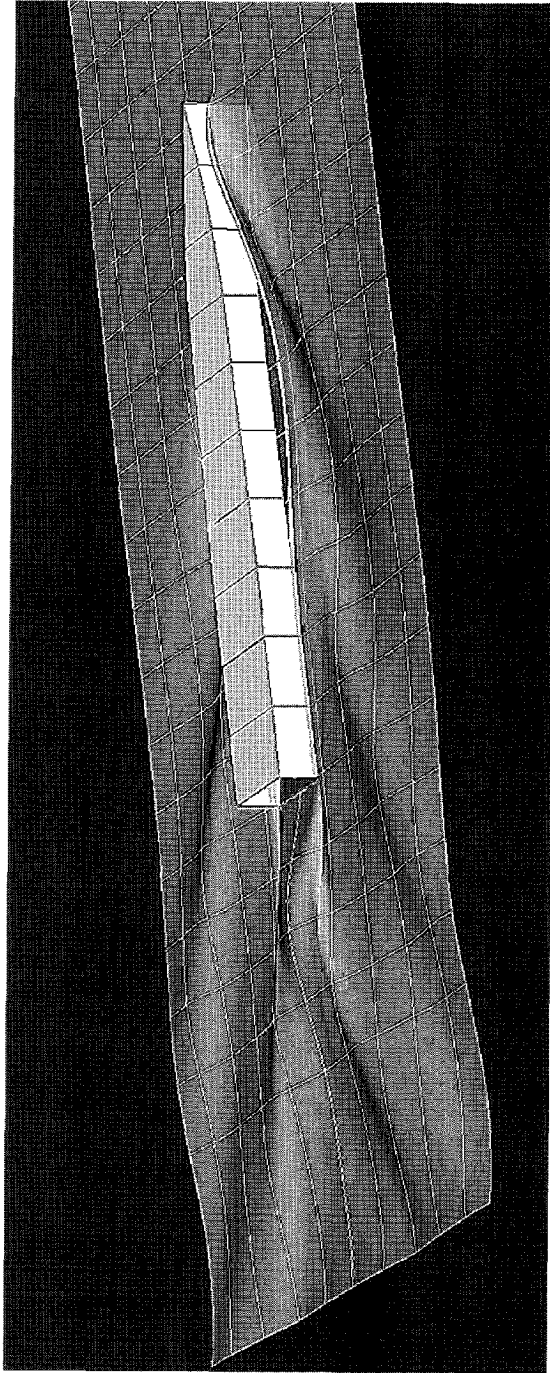
Figure 8.3: Calculated wave pattern for transom stern hull. Fn = 0.4 , Fn_{tr} = 4.0 .
