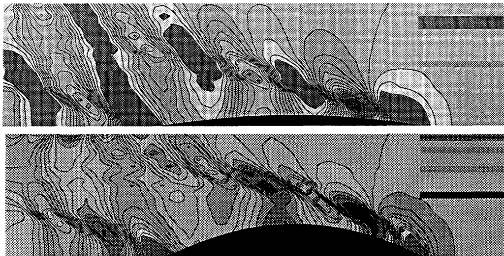
Figure 10.8: Wave pattern of parabolic models with L/B = 12 (top) and L/B = 4 (bottom), calculated using RAPID.
