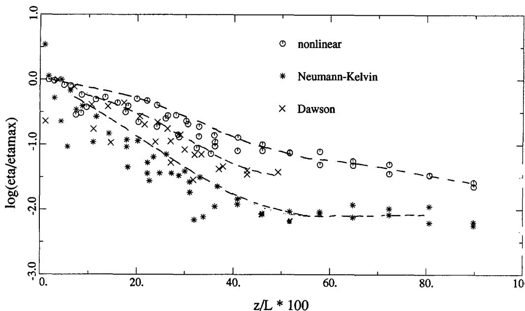
Figure 10.6: Logarithm of normalised maximum height of bow wave system predicted by various methods, for parabolic model with L/B = 4 .
