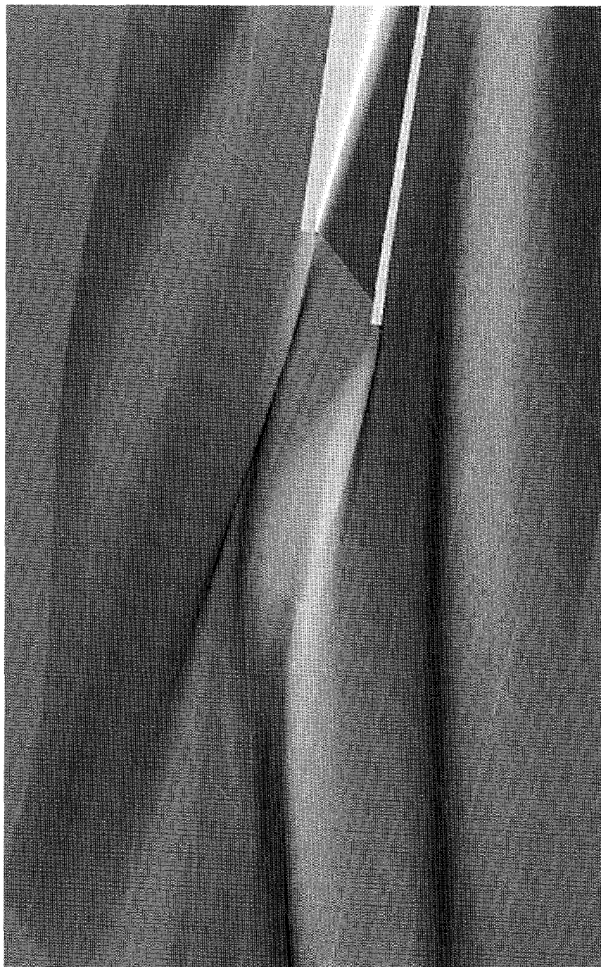
Figure 8.4: Close-up of flow off the transom stern. Fn = 0.4 , Fn_r = 4.0 .
