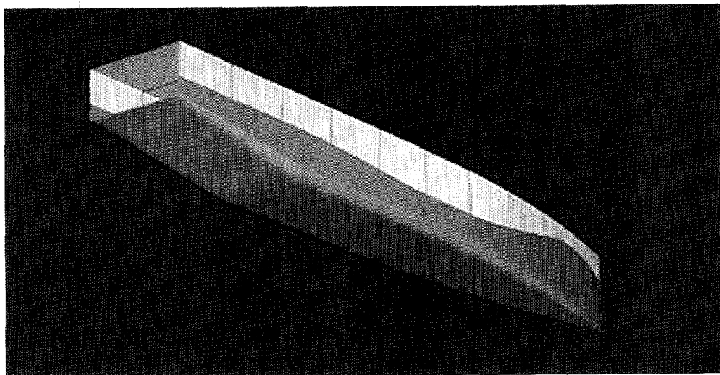
Figure 8.5: Transom stern hull form for test calculations.
