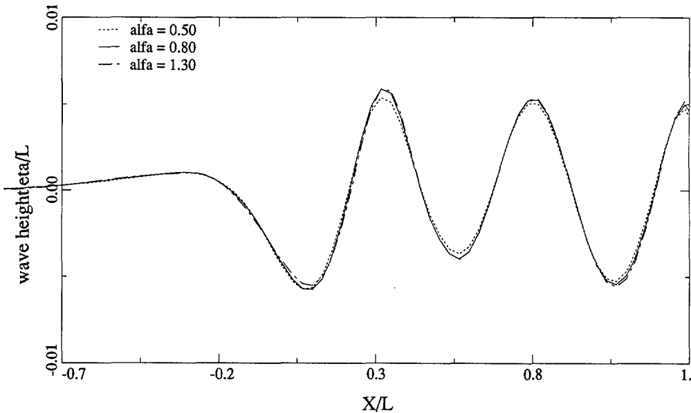
Figure 7.5: Effect of panel elevation on longitudinal cut at z/L = 0.2723 . Series 60 model, Fn = 0.316 , 10 \times 79 free surface panels.
