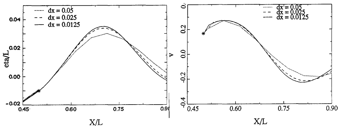
Figure 8.6: Effect of longitudinal panel refinement on wave profile (left) and vertical velocity (right) aft of a transom stern. Fn = 0.4 , \eta_{tr} = -0.01 , Fn_{tr} = 4.0 . Transom edge located at X/L = 0.5 .
