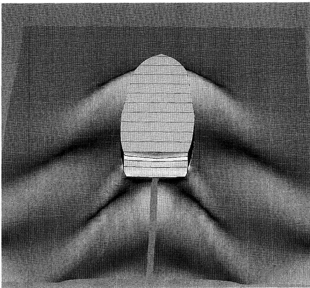
Figure 7.16: The steep wave pattern of a harbour tug, as calculated by RAPID
