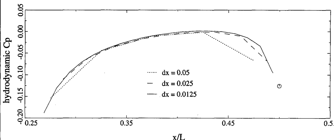
Figure 8.7: Effect of longitudinal panel refinement on hull pressure distribution along the centre-line. Fn = 0.4 , Fn_{tr} = 4.0 . Marker indicates pressure at transom edge according to dynamic condition.
