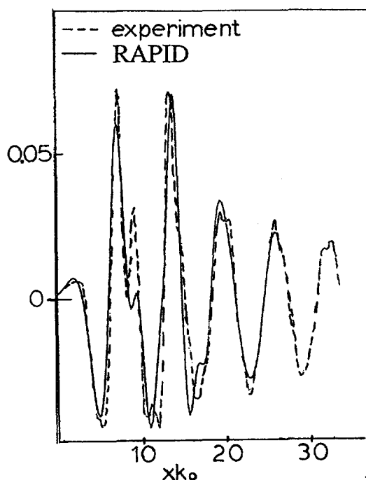
Figure 9.15: Calculated and experimental wave cut; DTRC Model 5415, F_n = 0.4136 , z/L = 0.324 .
